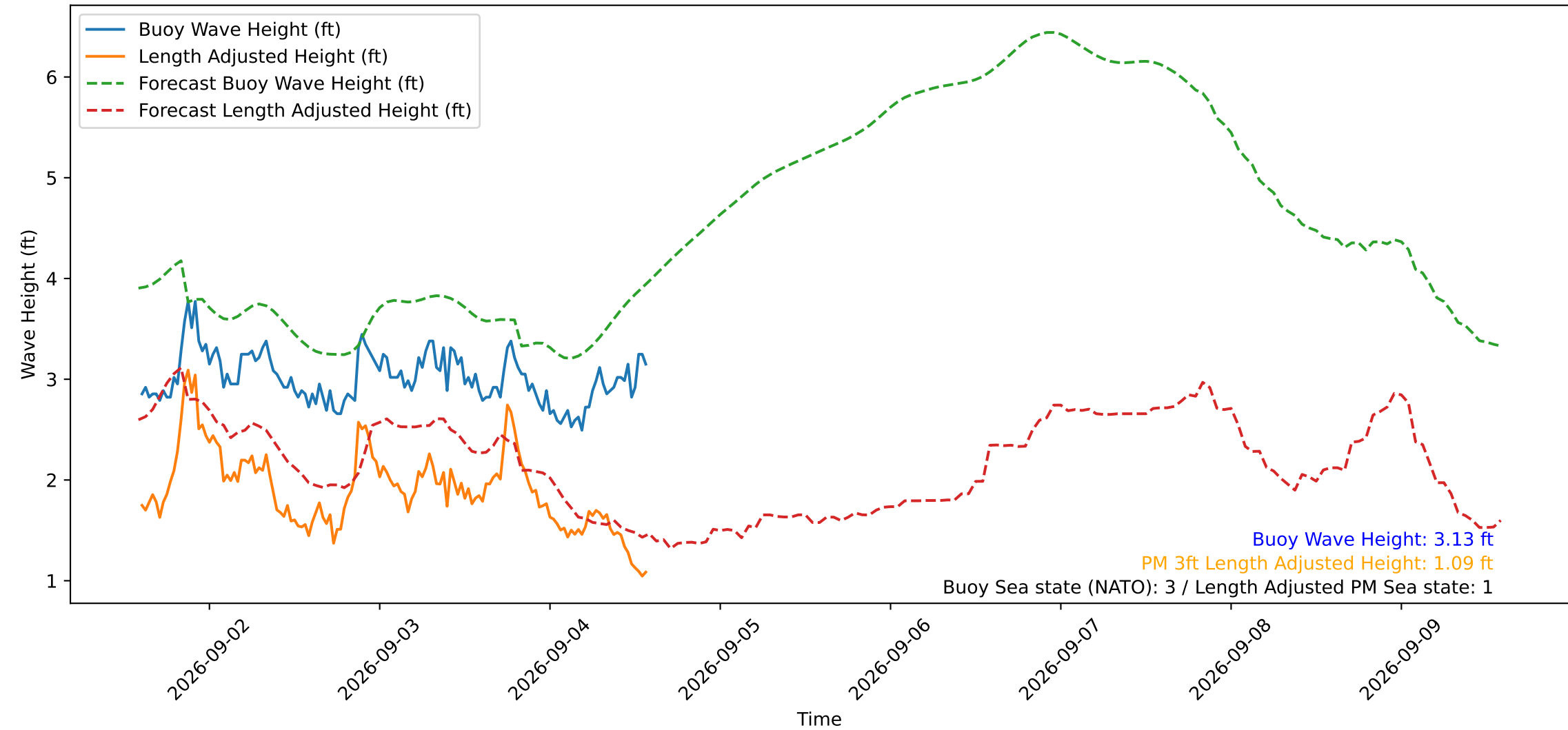
Wave Heights over Time for Green Beach at 2026-09-04 14:21:15
