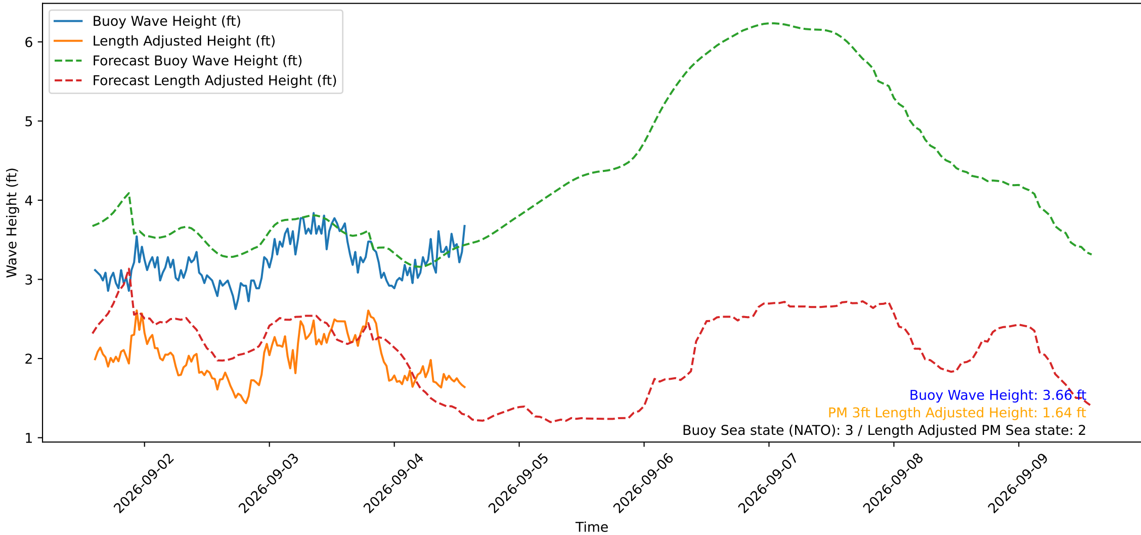
Wave Heights over Time for Oceanside Harbor at 2026-09-04 14:20:30
