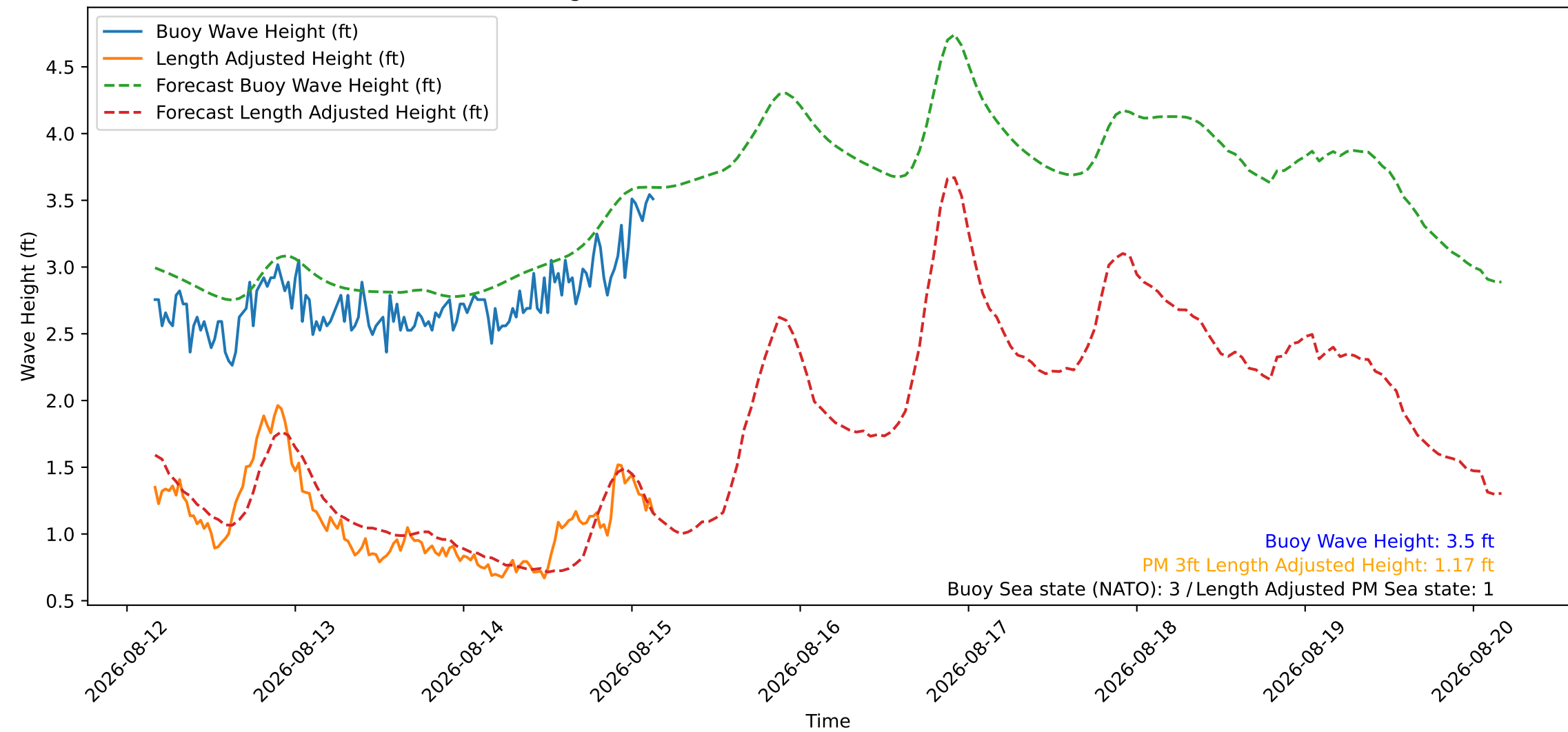
Wave Heights over Time for Green Beach at 2026-08-15 03:51:09
