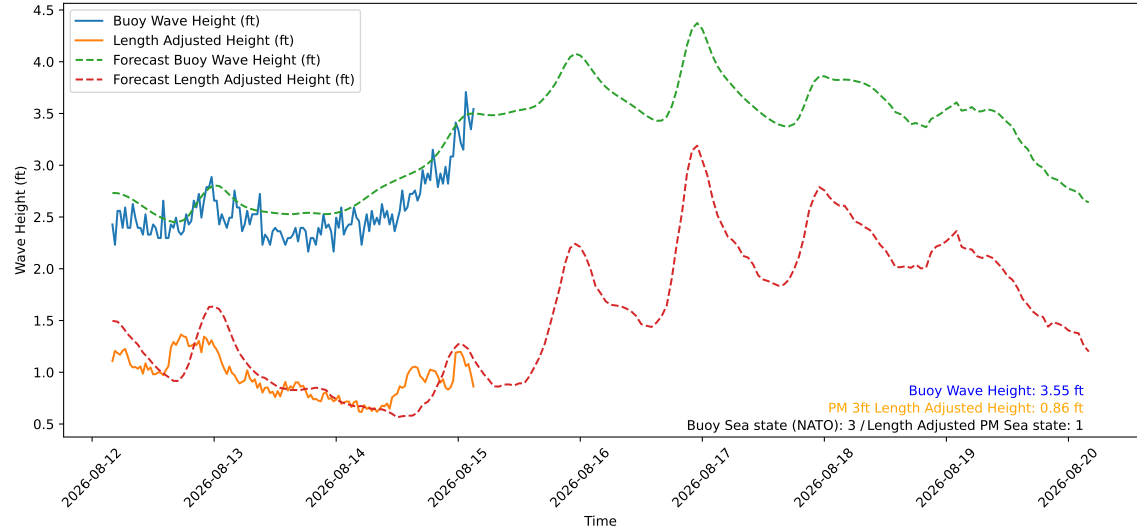
Wave Heights over Time for Red Beach at 2026-08-15 03:50:47
