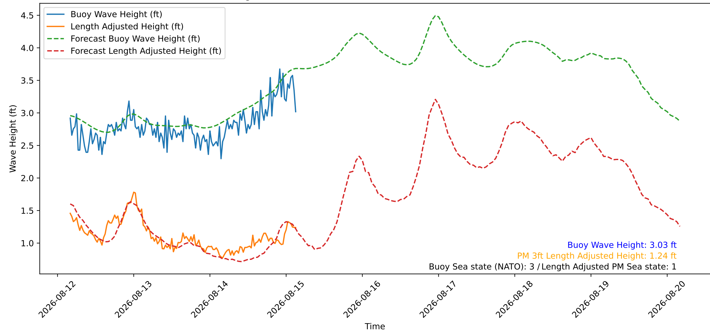
Wave Heights over Time for Oceanside Harbor at 2026-08-15 03:50:26
