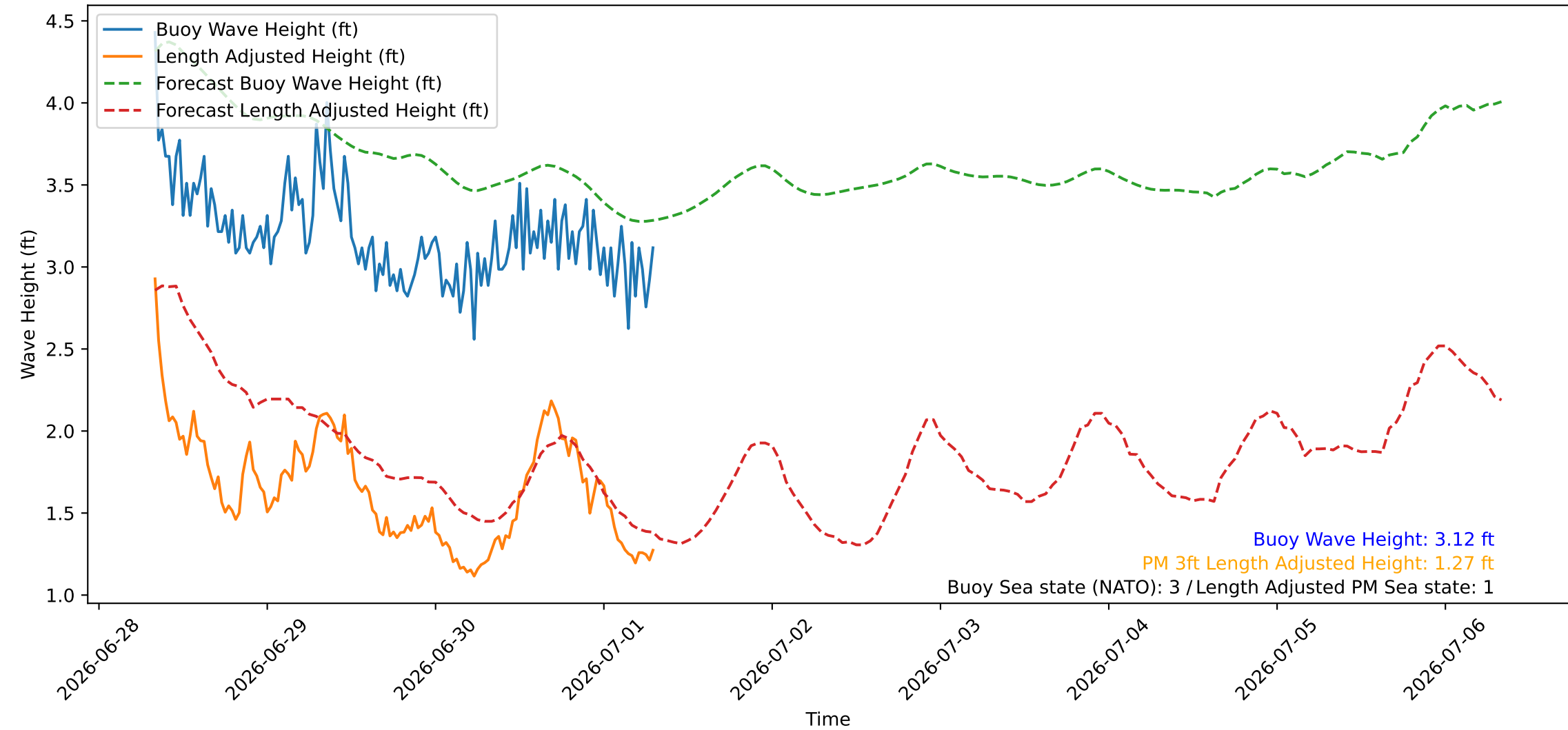
Wave Heights over Time for Oceanside Harbor at 2026-07-01 08:00:27
