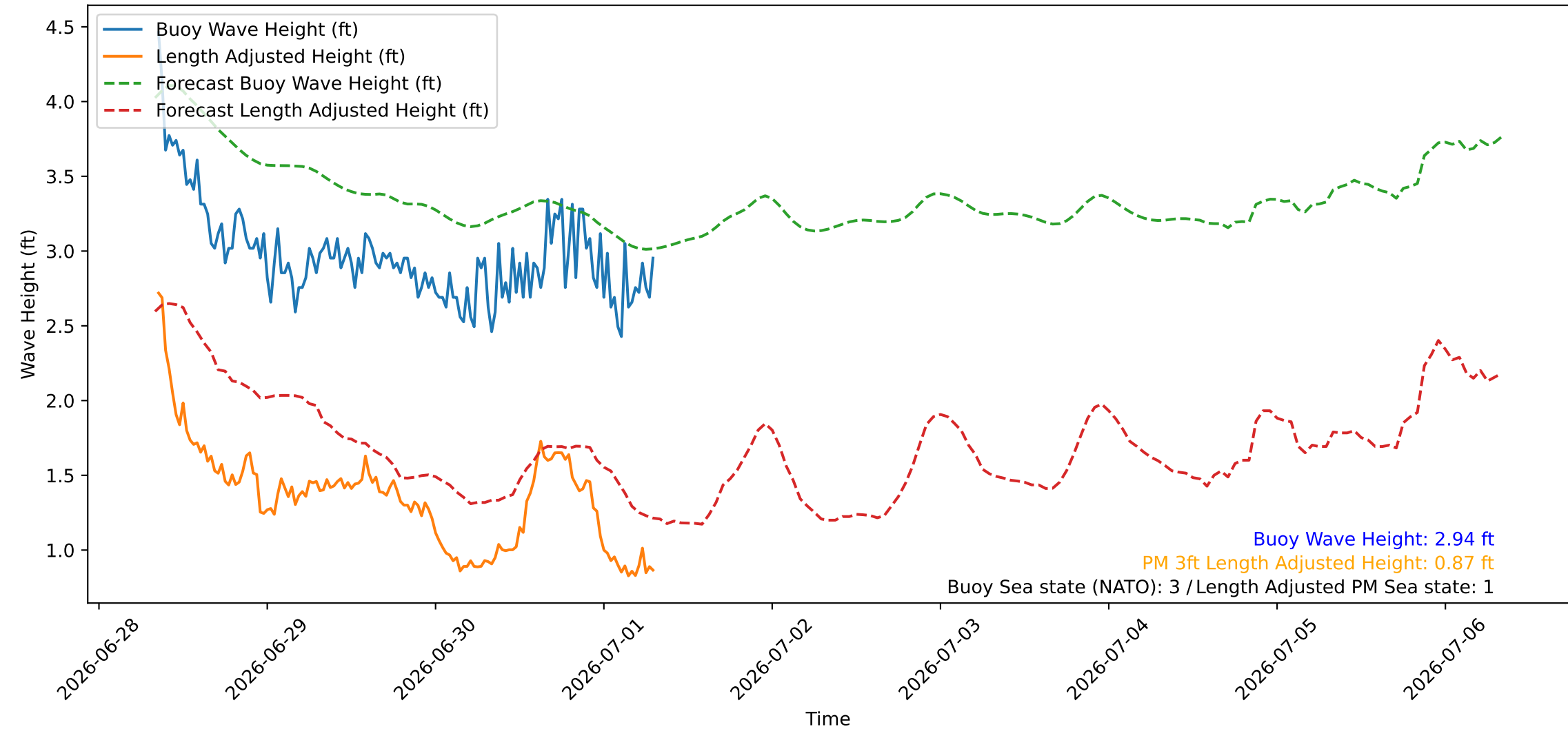
Wave Heights over Time for Red Beach at 2026-07-01 08:00:46
