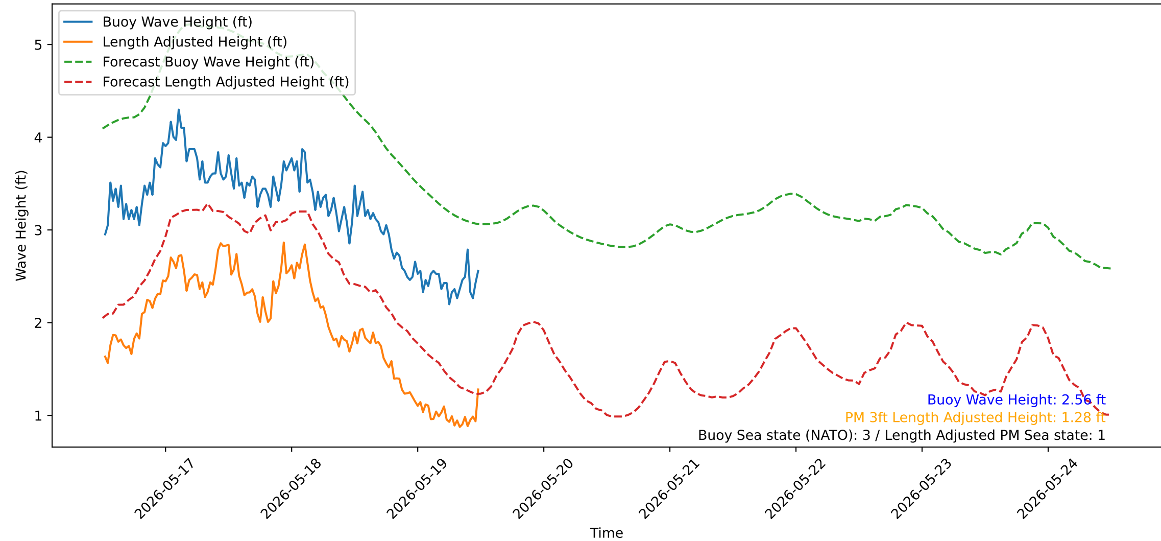
Wave Heights over Time for Oceanside Harbor at 2026-05-19 12:20:31
