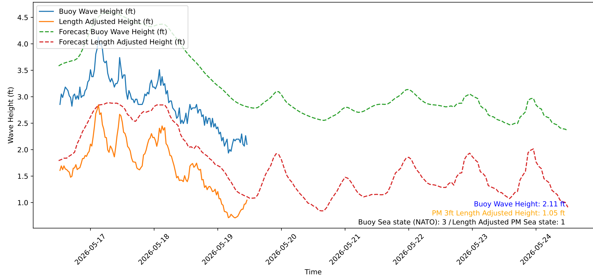
Wave Heights over Time for Red Beach at 2026-05-19 12:20:51
