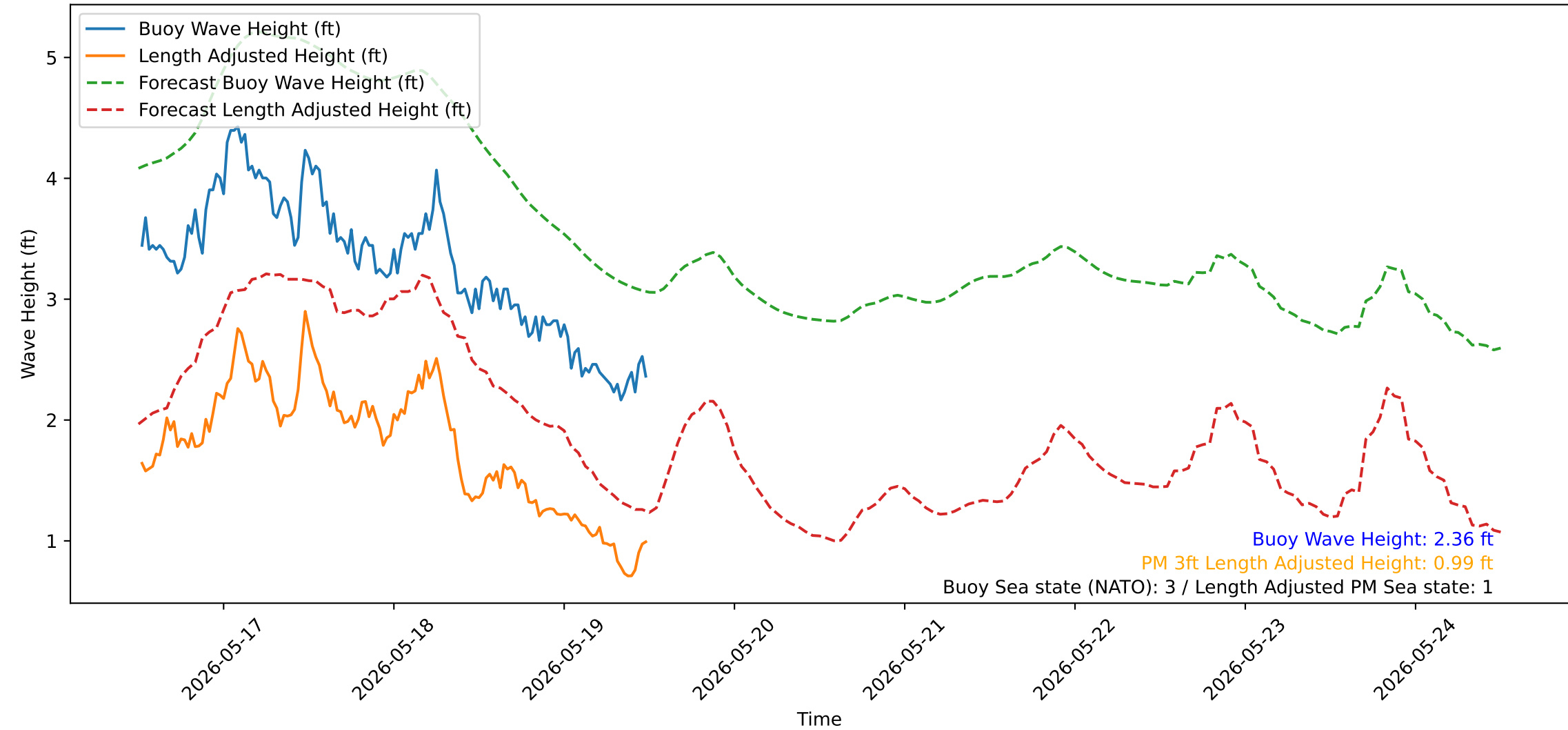
Wave Heights over Time for Green Beach at 2026-05-19 12:21:14
