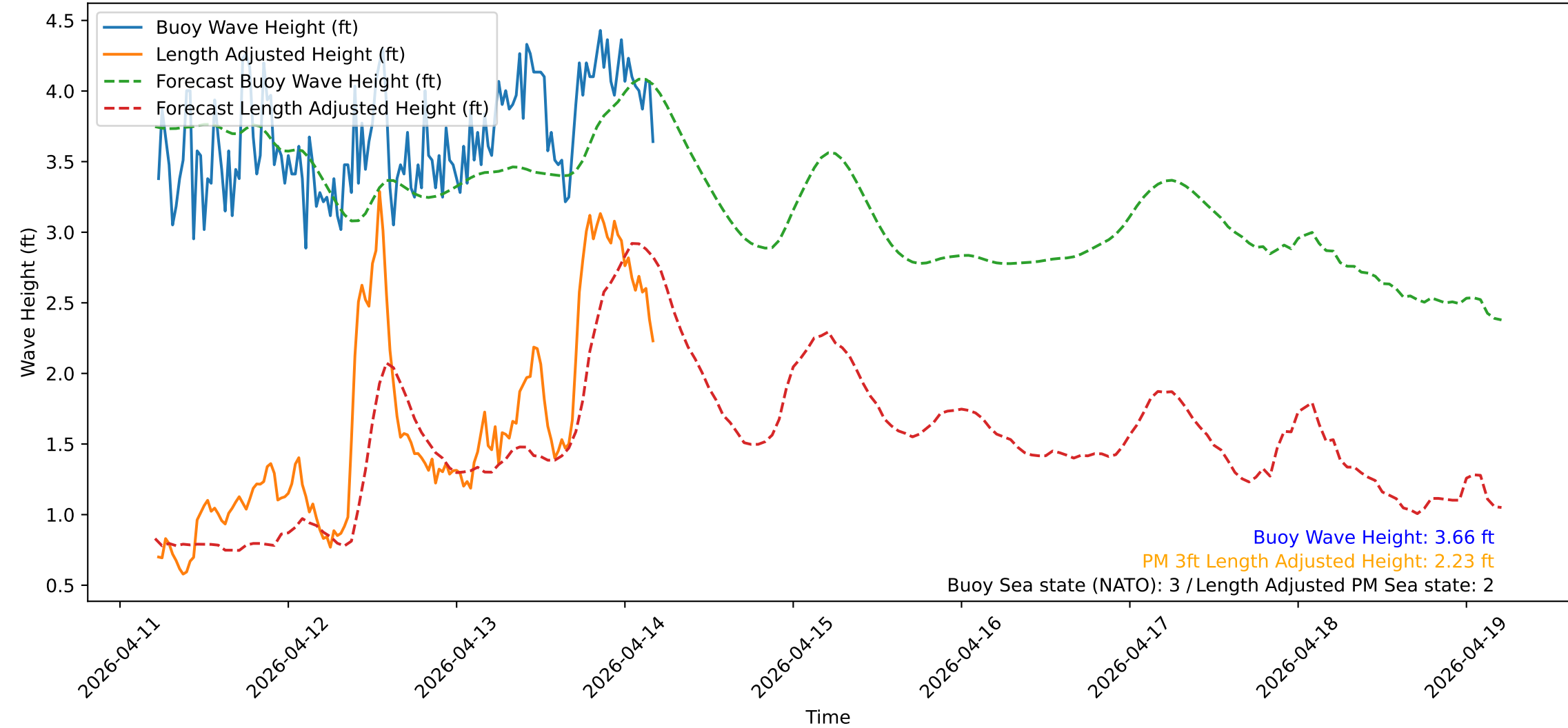
Wave Heights over Time for Red Beach at 2026-04-14 05:00:50
