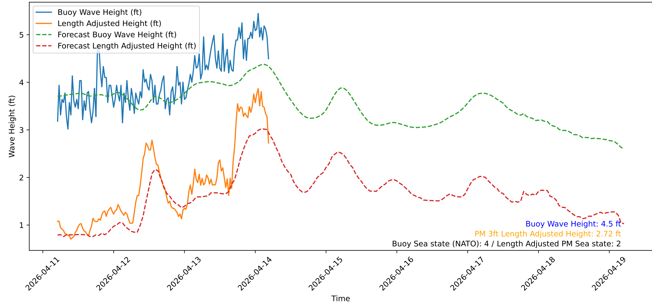
Wave Heights over Time for Oceanside Harbor at 2026-04-14 05:00:31
