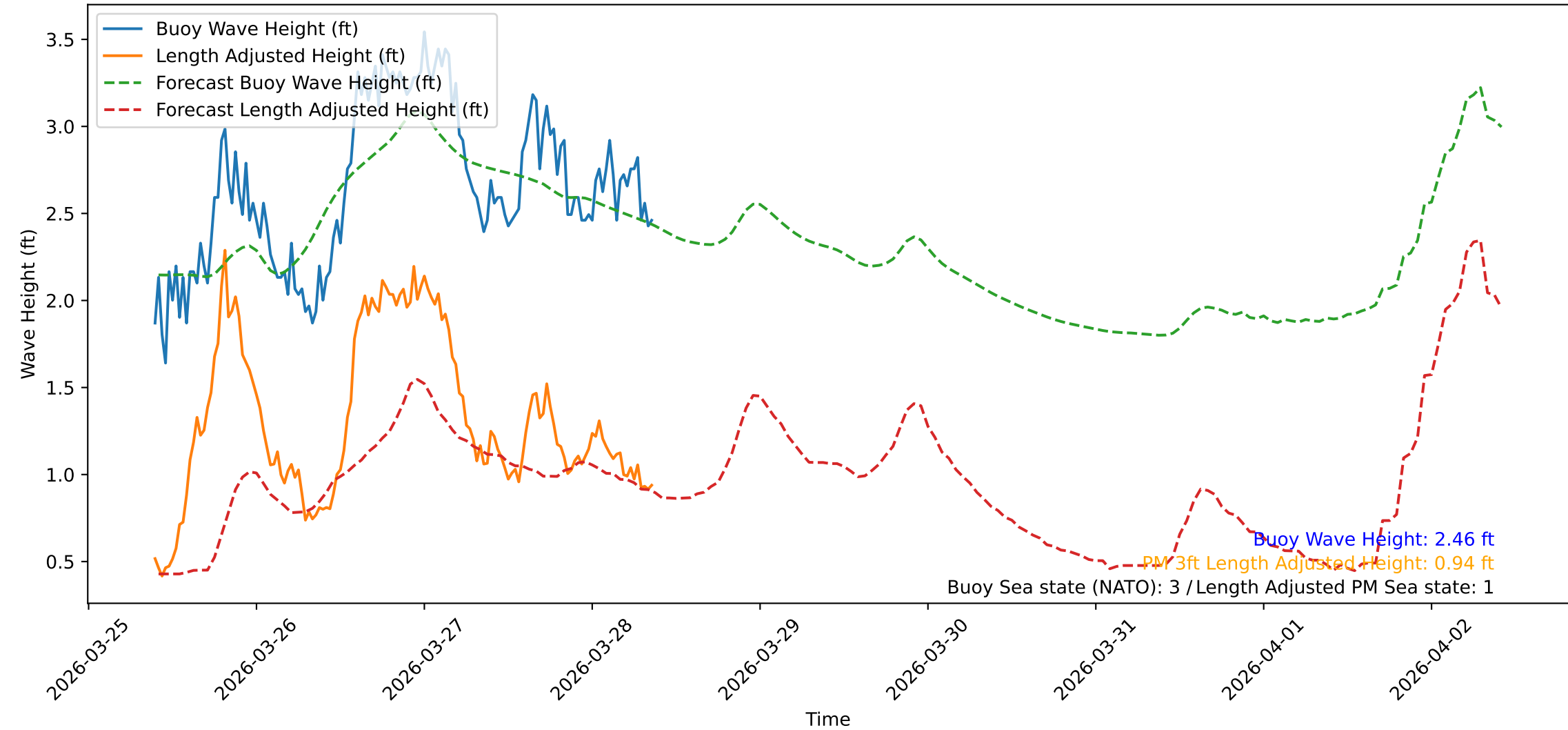
Wave Heights over Time for Green Beach at 2026-03-28 09:31:08
