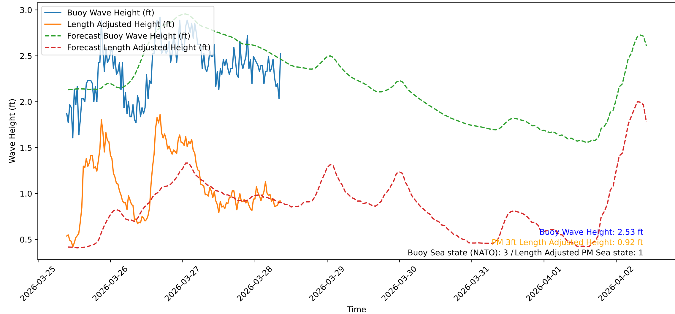
Wave Heights over Time for Oceanside Harbor at 2026-03-28 09:30:31
