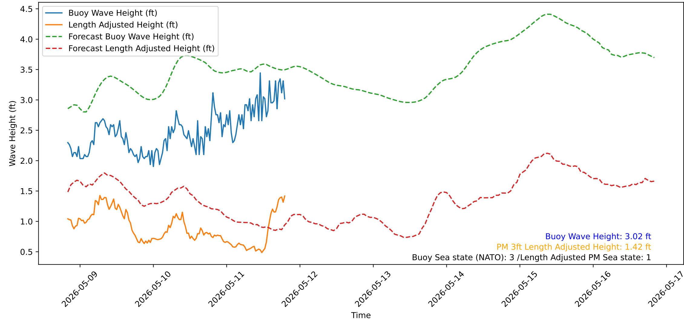
Wave Heights over Time for Green Beach at 2026-05-11 20:01:13
