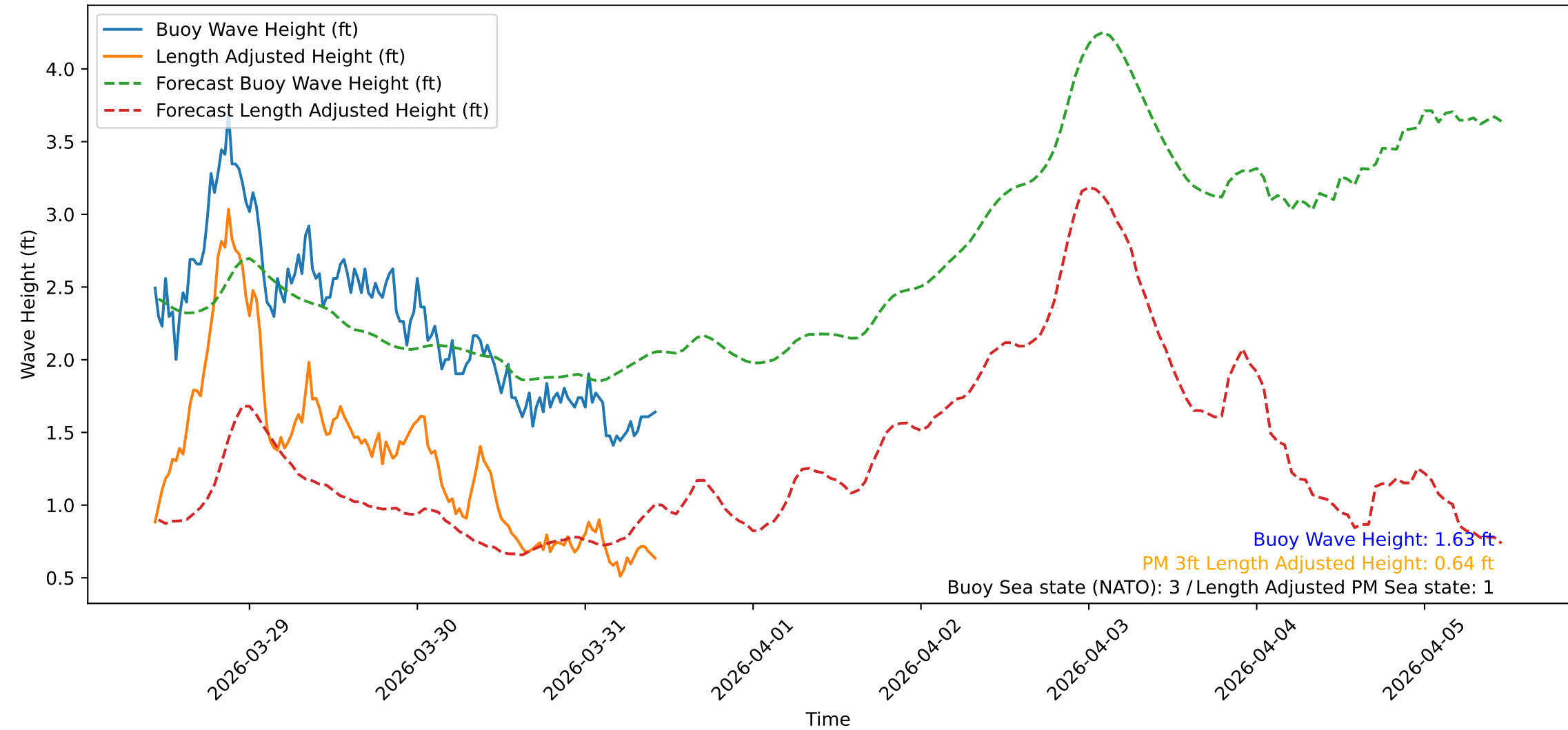
Wave Heights over Time for Green Beach at 2026-03-31 10:41:14
