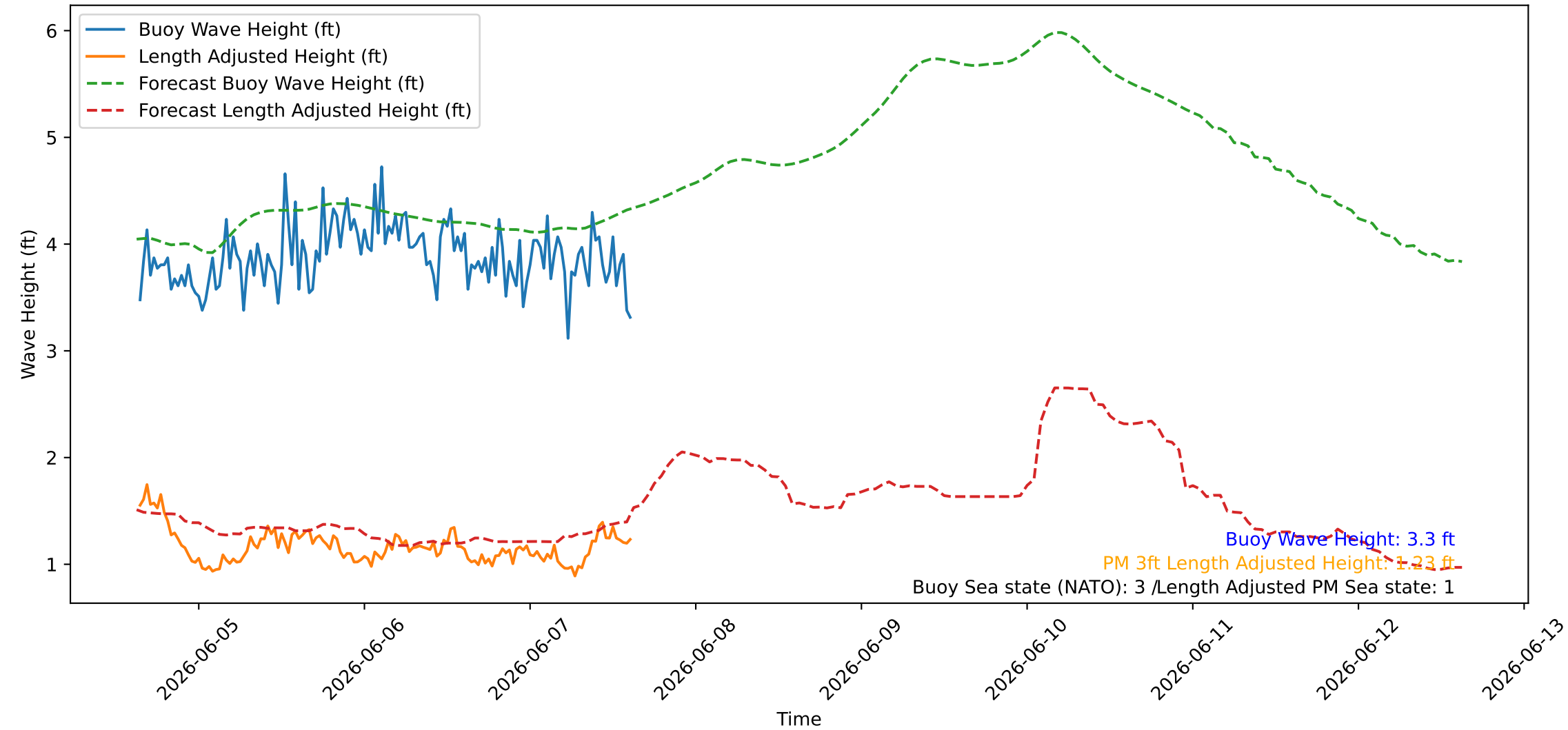
Wave Heights over Time for Green Beach at 2026-06-07 15:21:09
