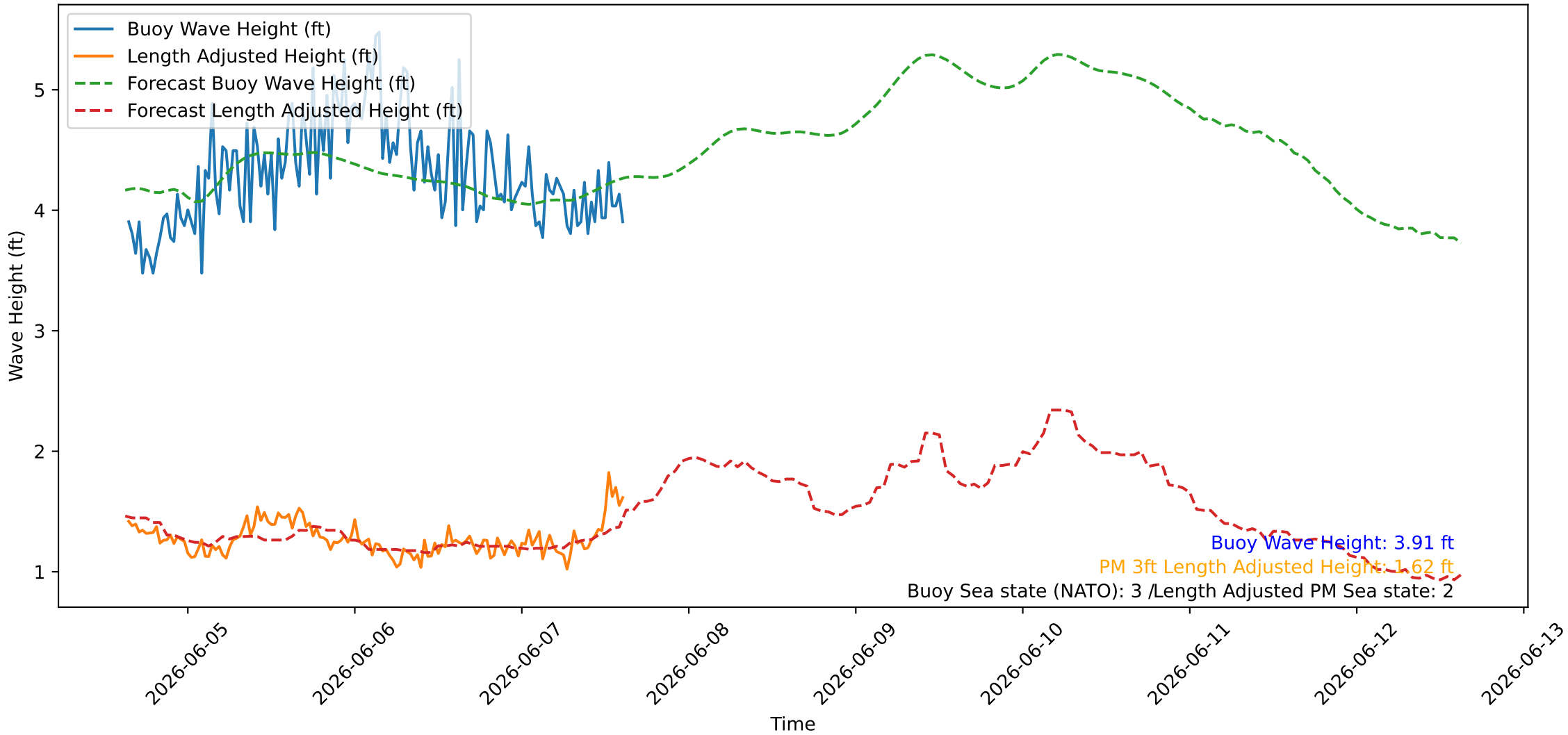
Wave Heights over Time for Oceanside Harbor at 2026-06-07 15:20:26
