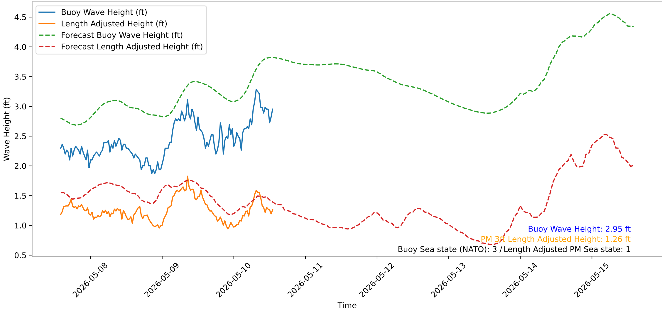
Wave Heights over Time for Oceanside Harbor at 2026-05-10 13:50:32
