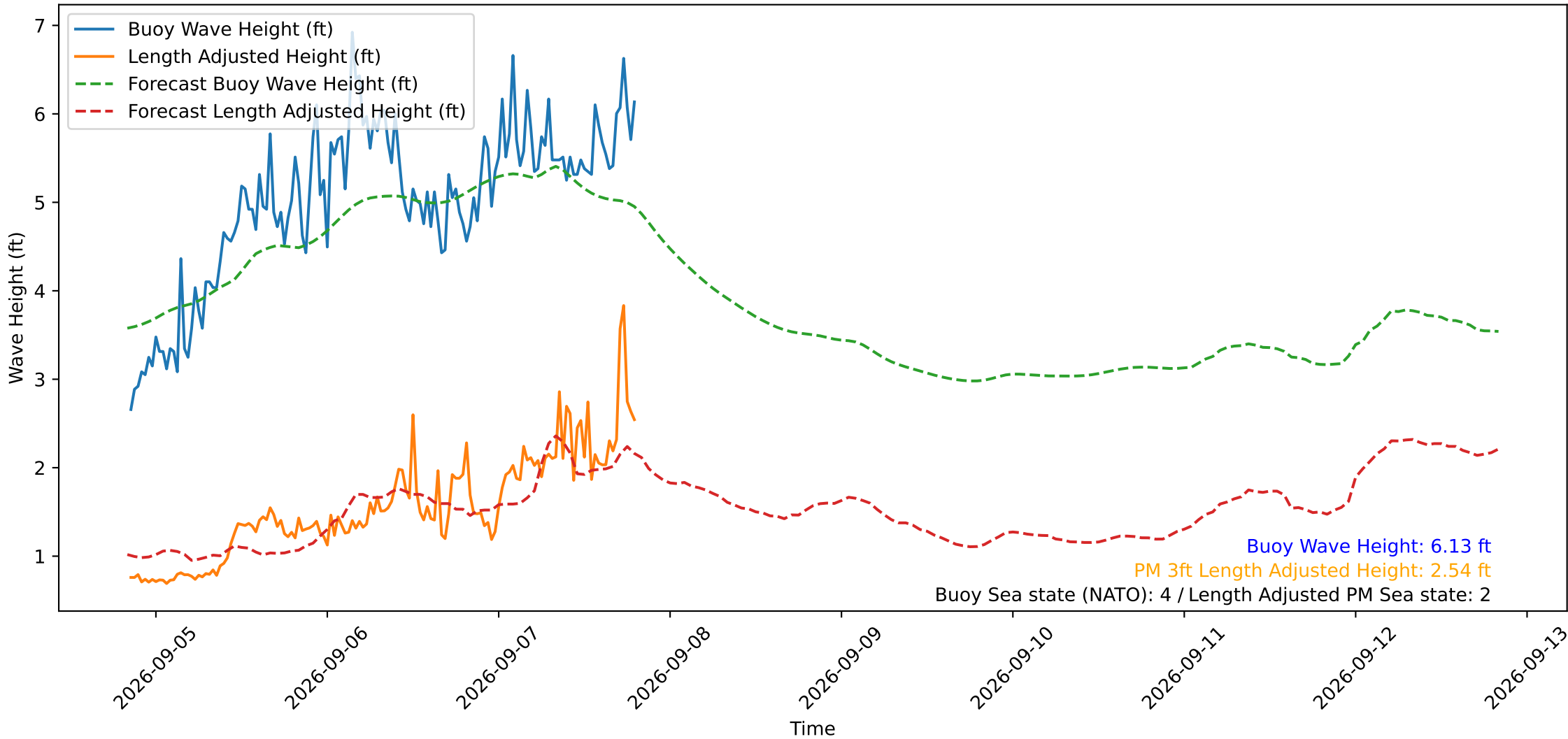
Wave Heights over Time for Red Beach at 2026-09-07 20:00:49
