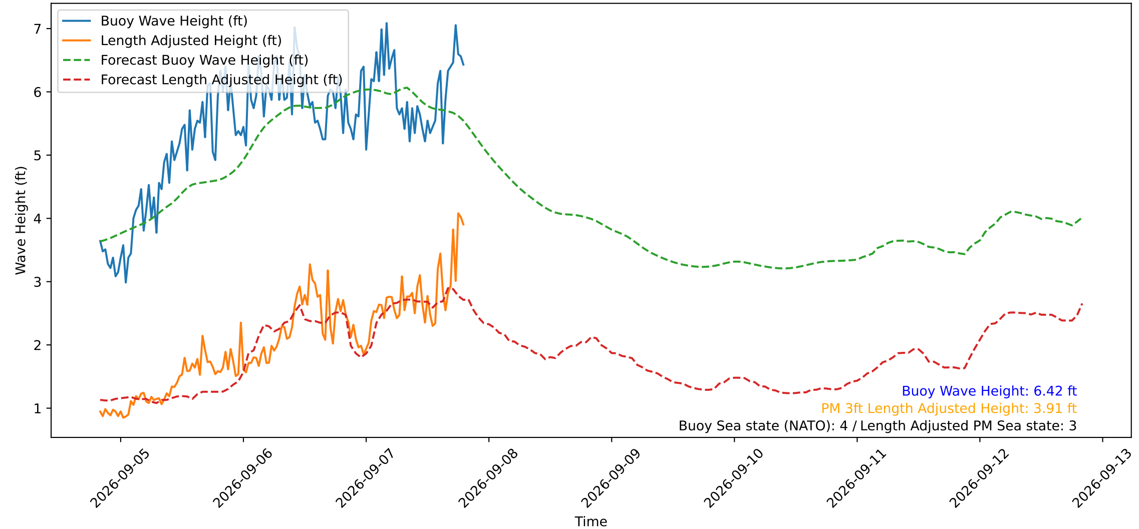
Wave Heights over Time for Oceanside Harbor at 2026-09-07 20:00:29
