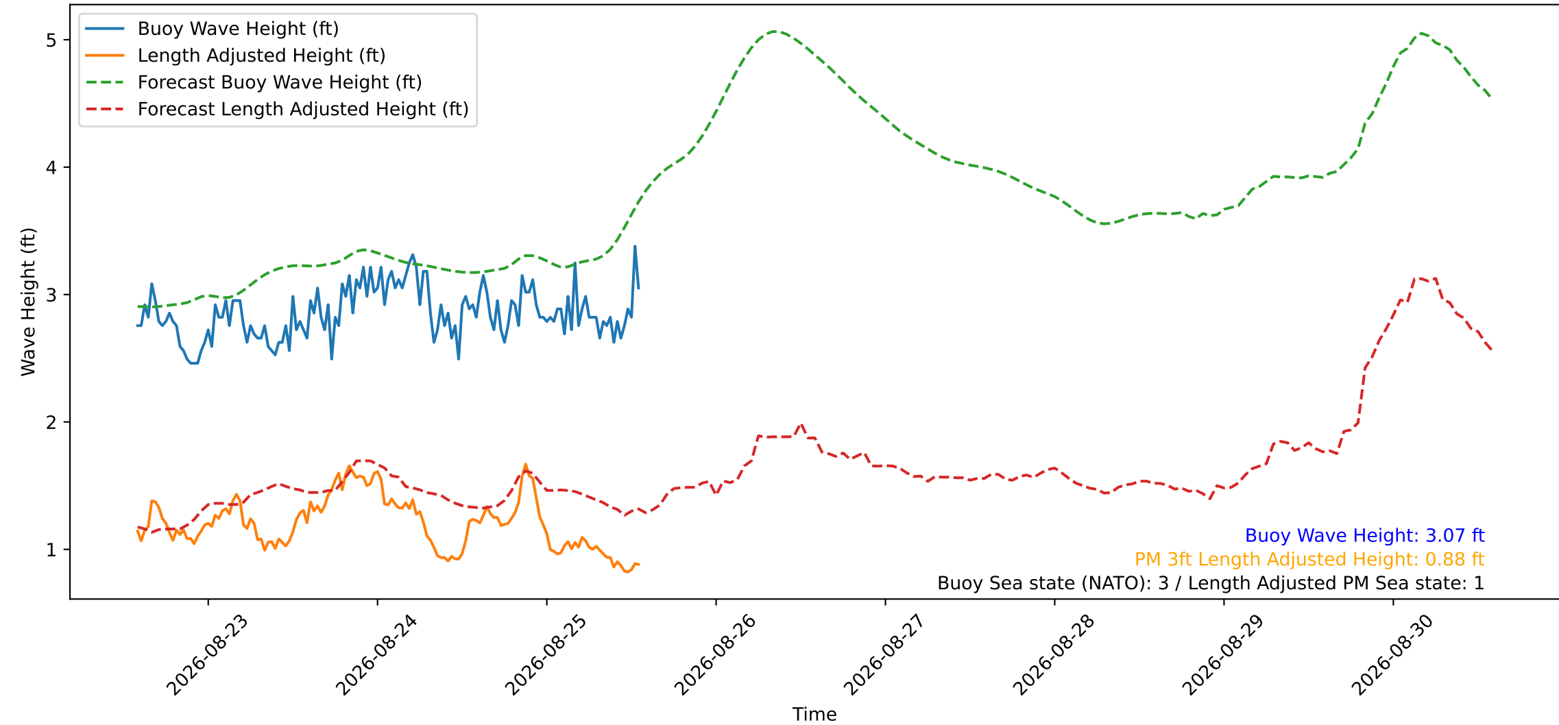
Wave Heights over Time for Green Beach at 2026-08-25 13:51:15
