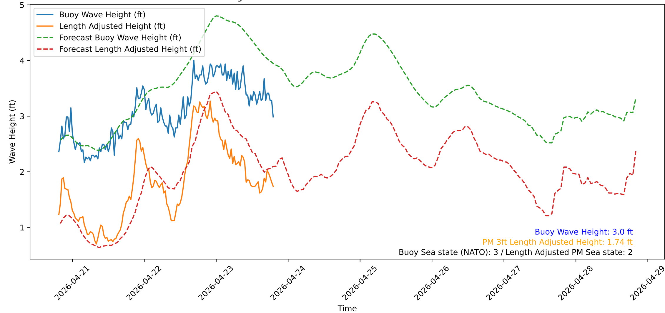
Wave Heights over Time for Green Beach at 2026-04-23 19:41:13
