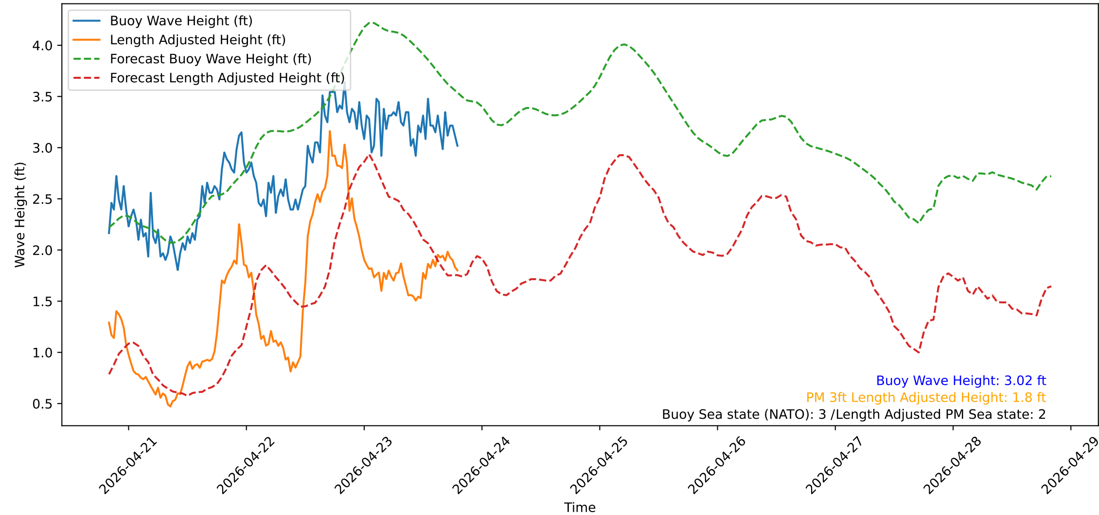
Wave Heights over Time for Red Beach at 2026-04-23 19:40:51
