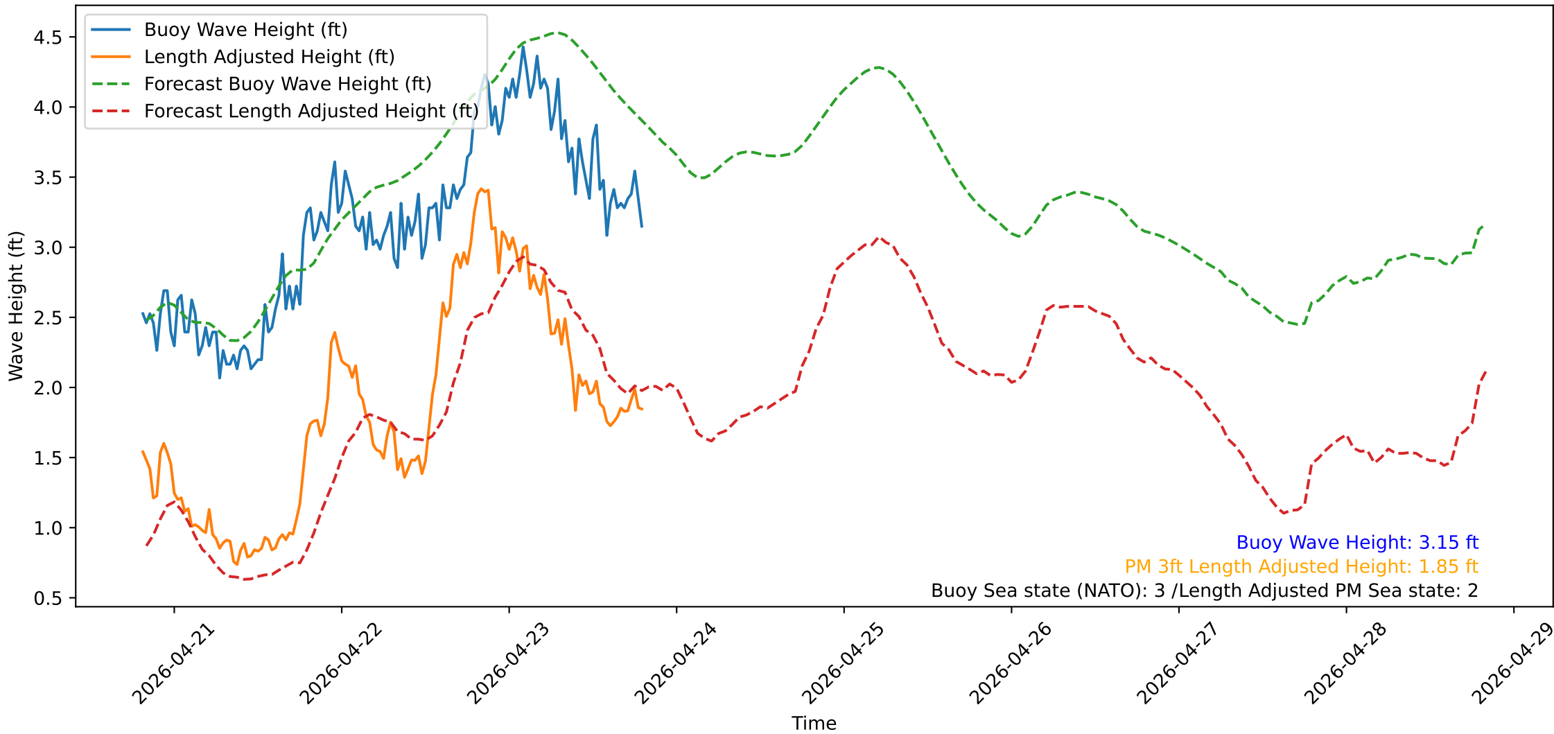
Wave Heights over Time for Oceanside Harbor at 2026-04-23 19:40:32
