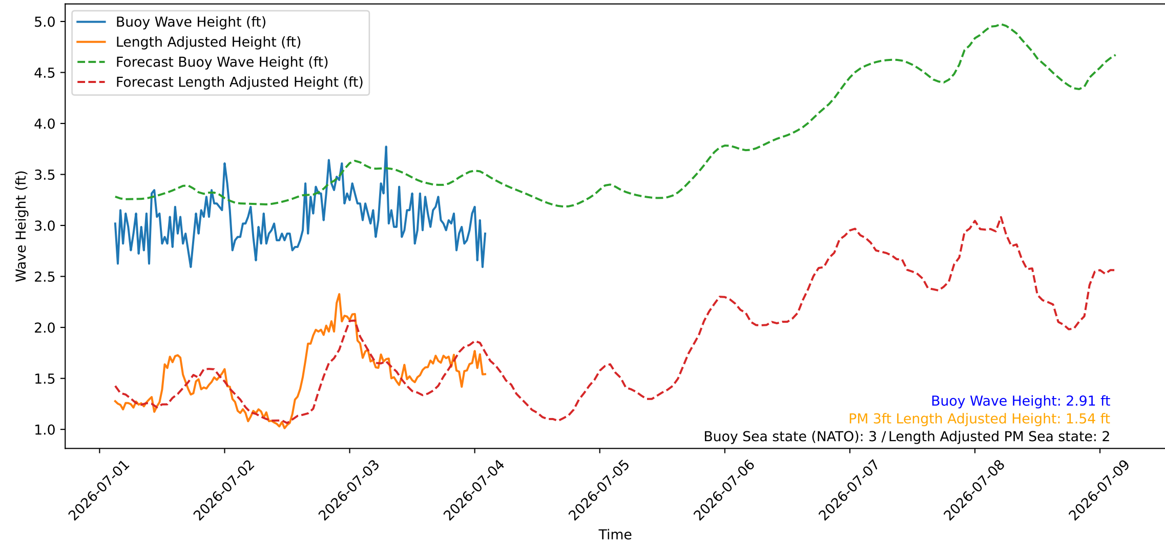
Wave Heights over Time for Oceanside Harbor at 2026-07-04 02:50:26
