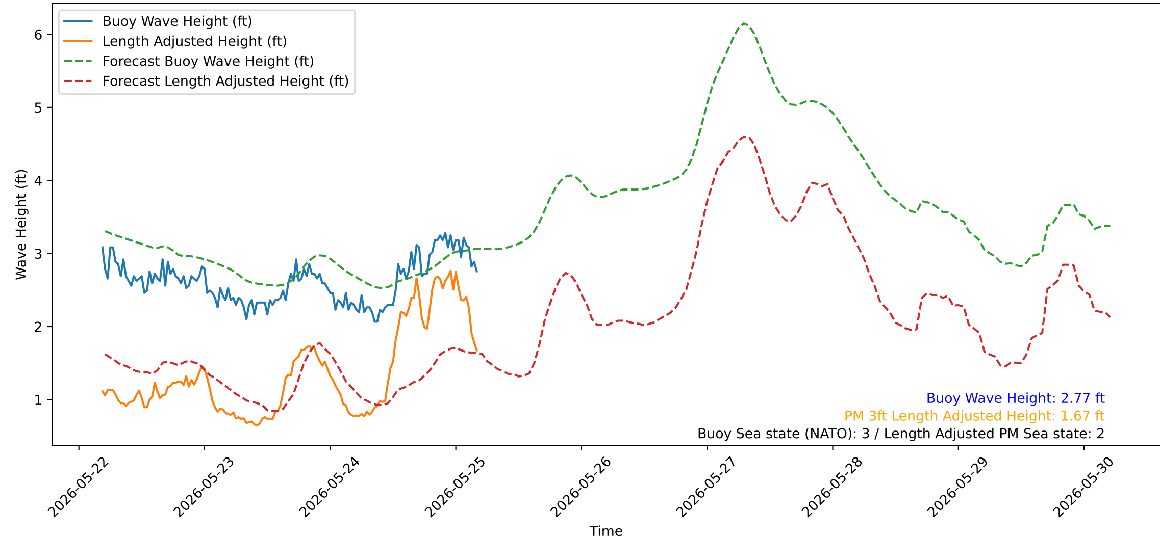
Wave Heights over Time for Green Beach at 2026-05-25 04:41:14
