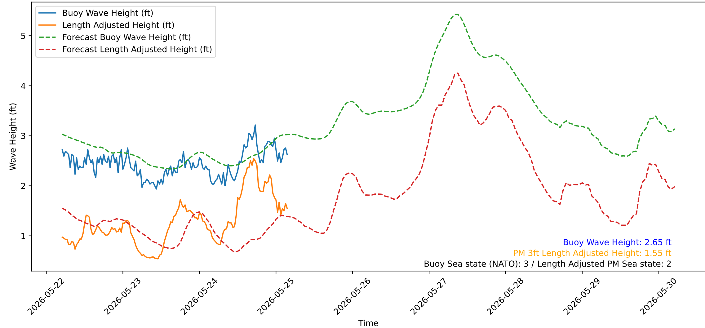
Wave Heights over Time for Red Beach at 2026-05-25 04:40:51
