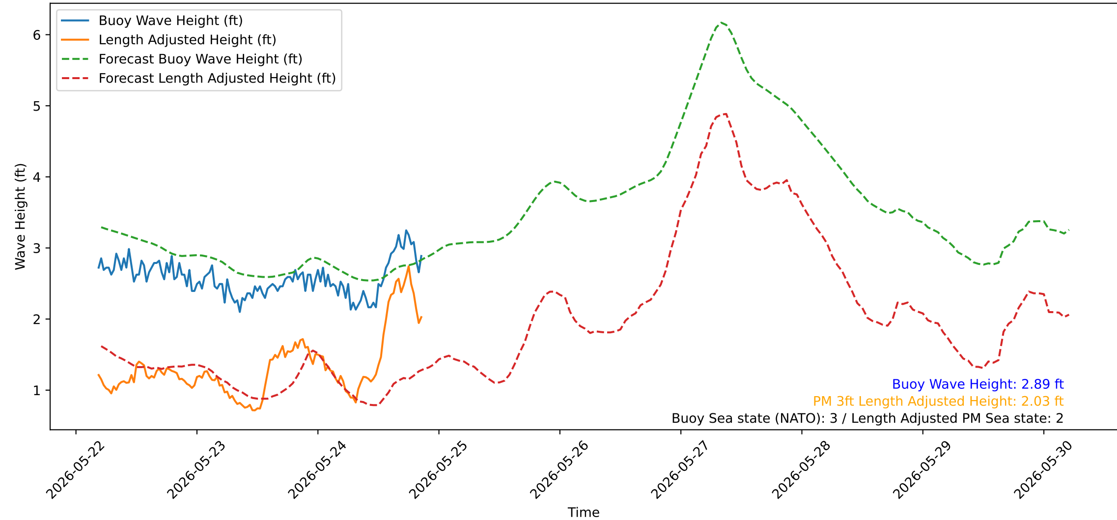
Wave Heights over Time for Oceanside Harbor at 2026-05-25 04:40:32
