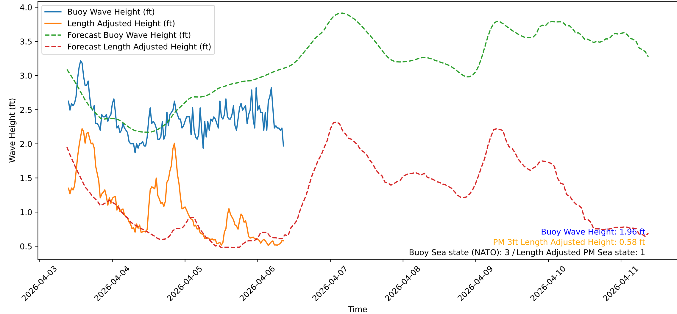
Wave Heights over Time for Red Beach at 2026-04-06 09:10:54
