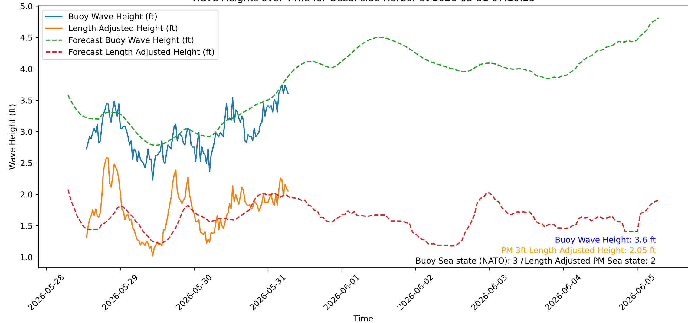
Wave Heights over Time for Oceanside Harbor at 2026-05-31 07:10:25
