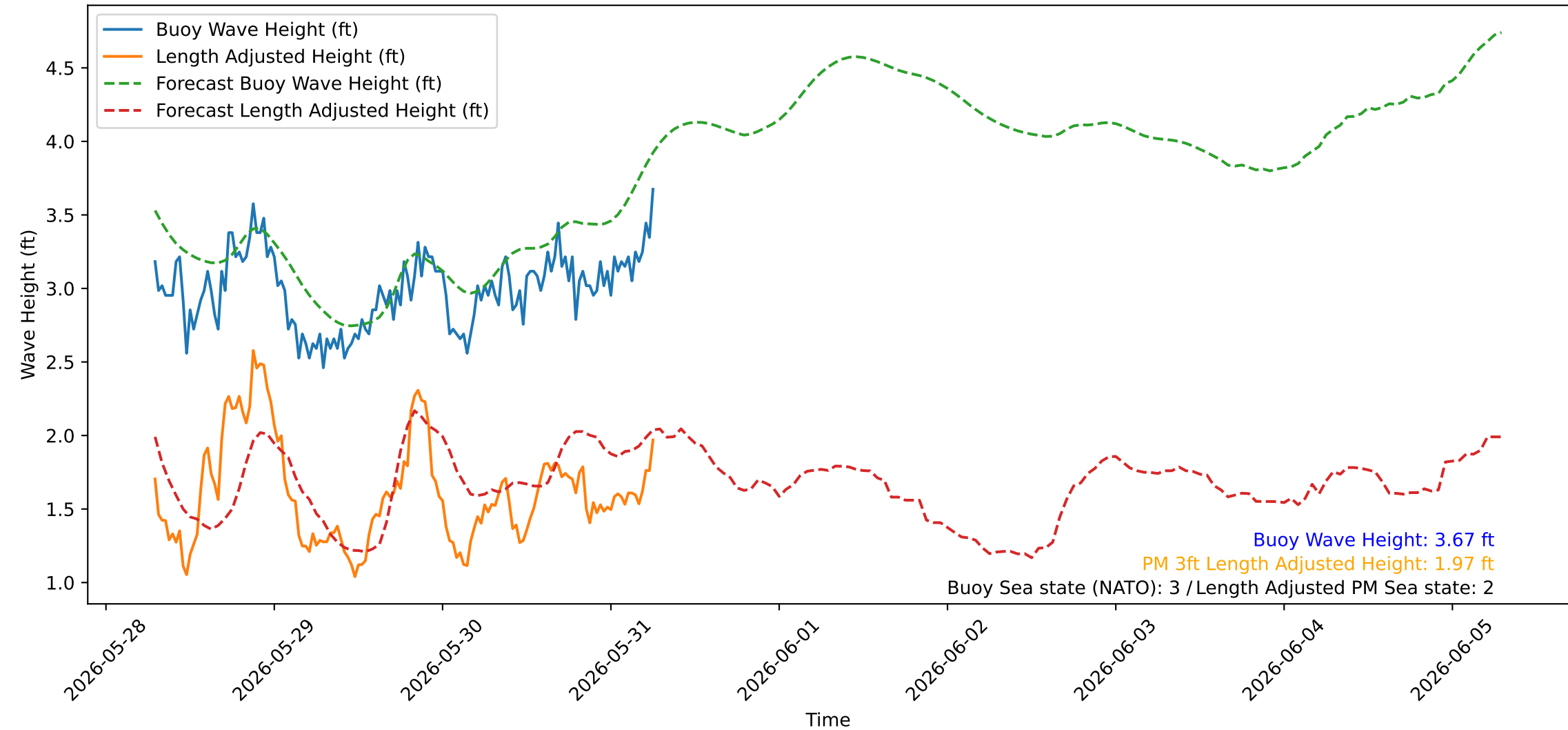
Wave Heights over Time for Green Beach at 2026-05-31 07:11:07
