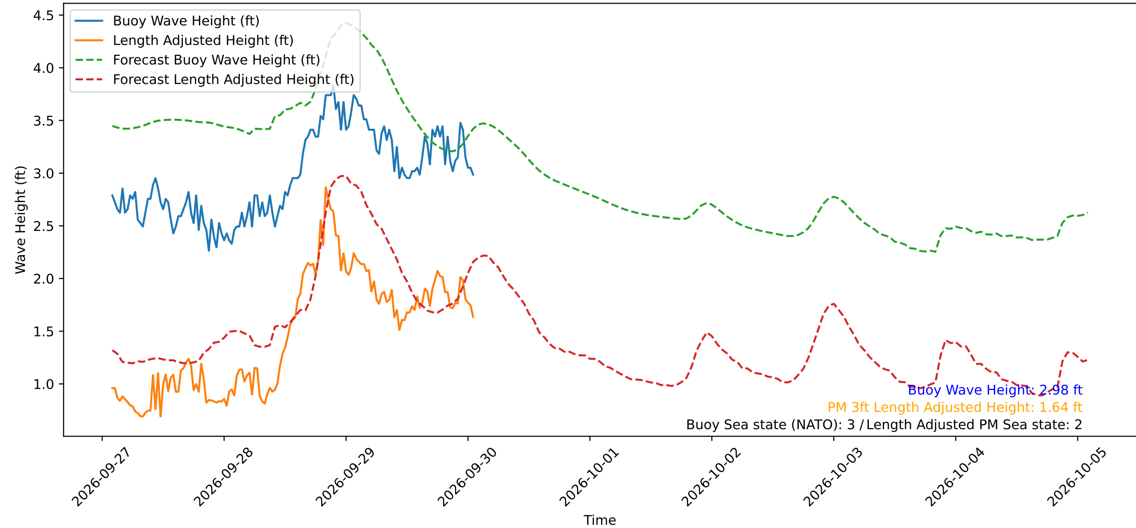
Wave Heights over Time for Red Beach at 2026-09-30 01:50:50
