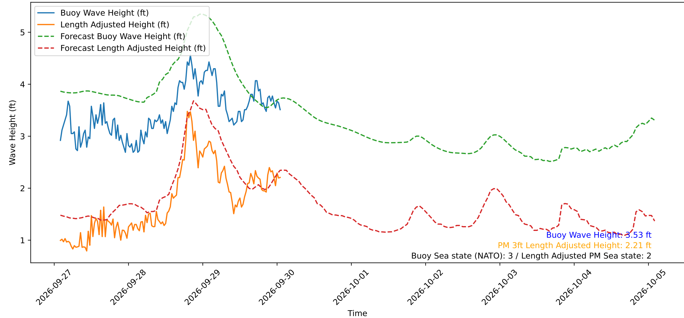
Wave Heights over Time for Green Beach at 2026-09-30 01:51:15
