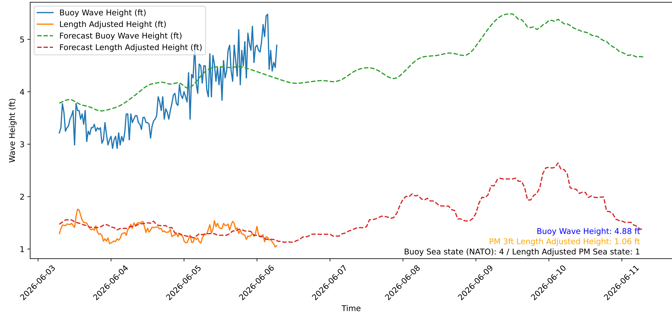
Wave Heights over Time for Oceanside Harbor at 2026-06-06 07:00:26
