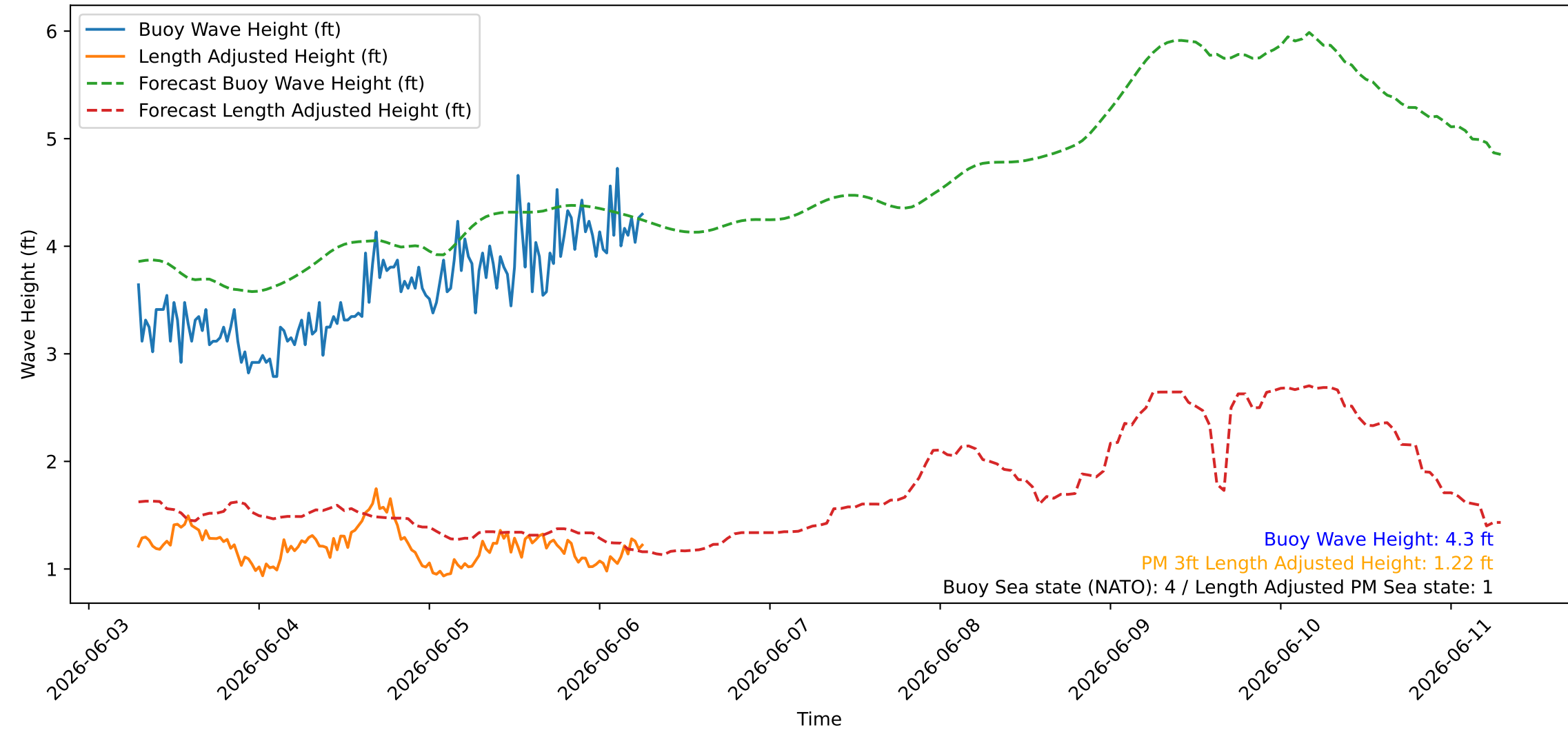
Wave Heights over Time for Green Beach at 2026-06-06 07:01:08
