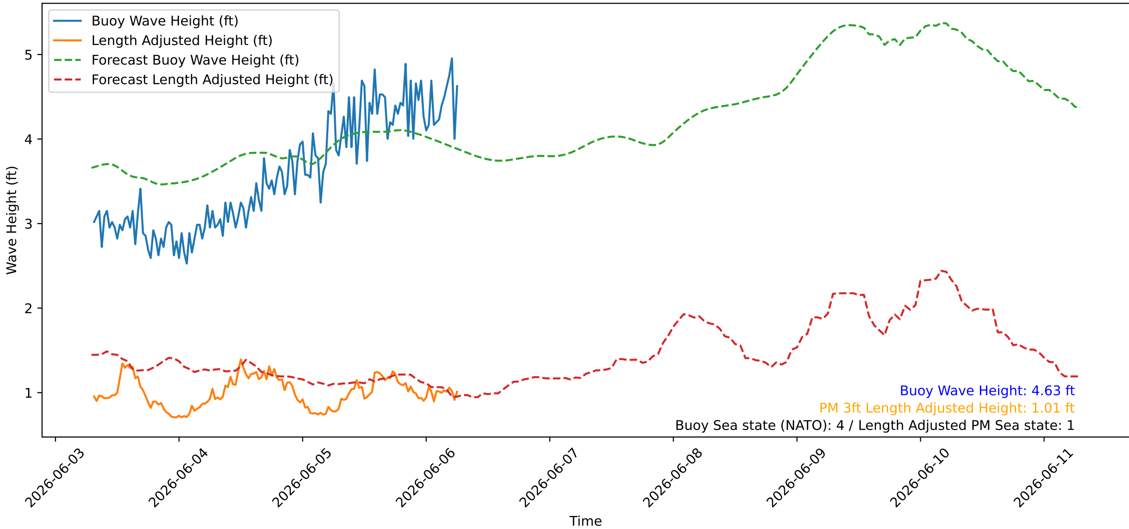
Wave Heights over Time for Red Beach at 2026-06-06 07:00:45
