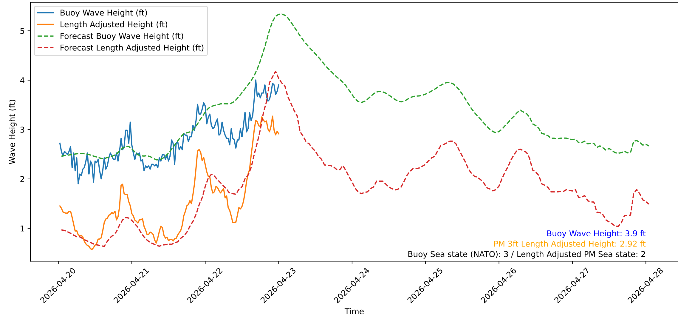
Wave Heights over Time for Green Beach at 2026-04-23 00:41:13
