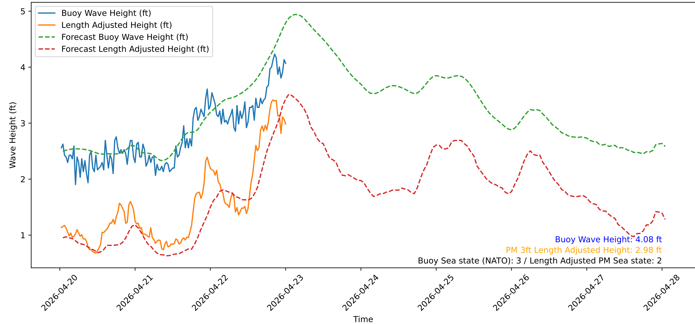
Wave Heights over Time for Oceanside Harbor at 2026-04-23 00:40:32
