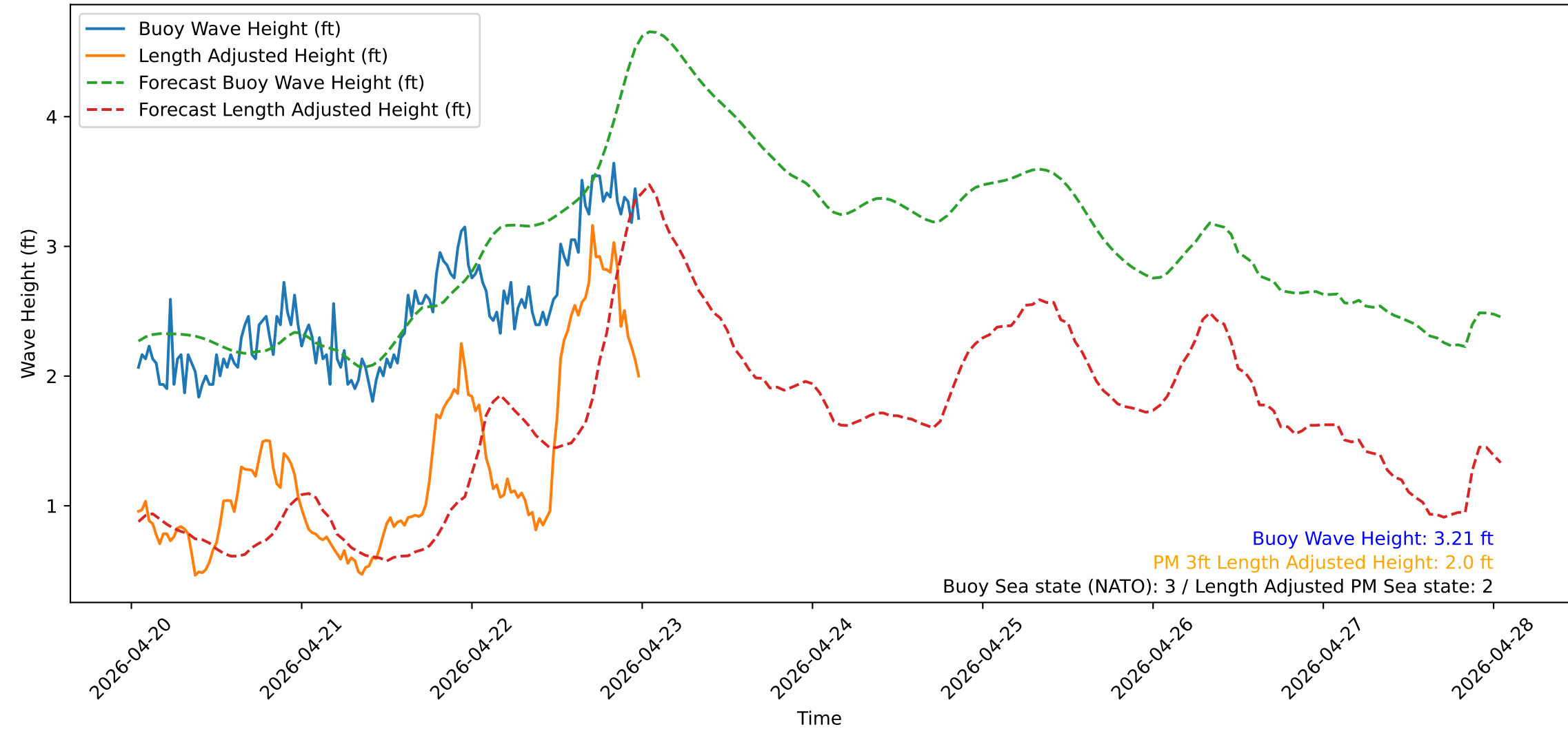
Wave Heights over Time for Red Beach at 2026-04-23 00:40:51
