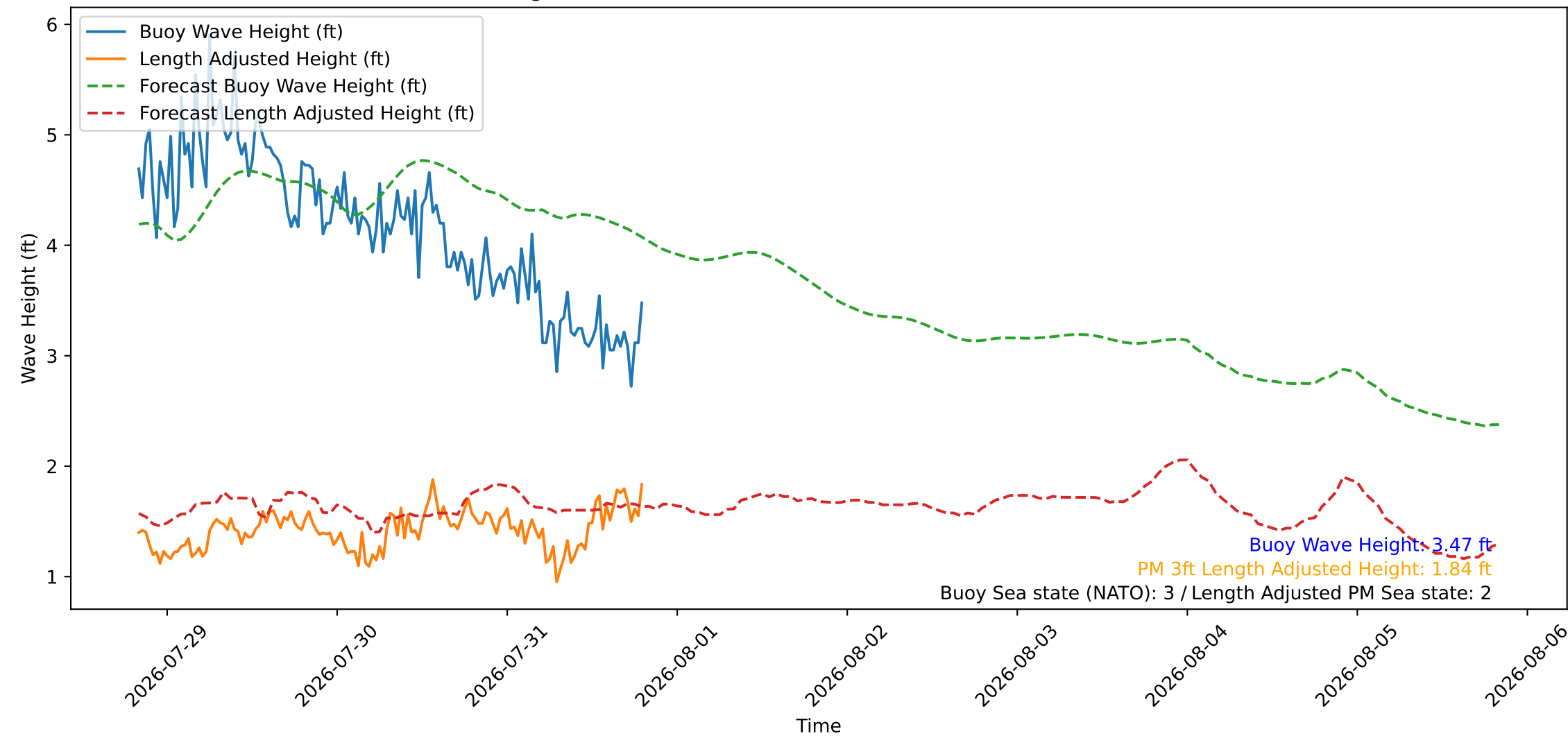
Wave Heights over Time for Oceanside Harbor at 2026-07-31 20:00:26
