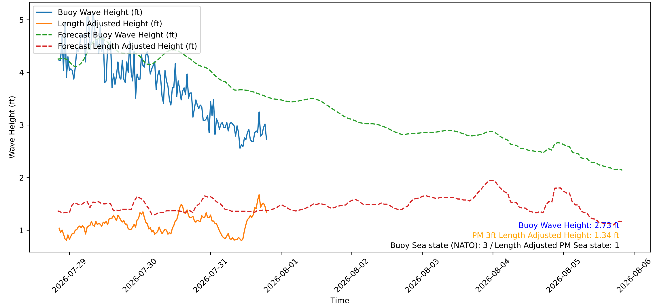
Wave Heights over Time for Red Beach at 2026-07-31 20:00:46
