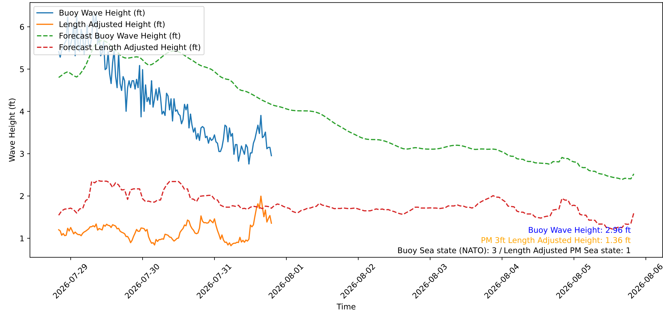
Wave Heights over Time for Green Beach at 2026-07-31 20:01:10
