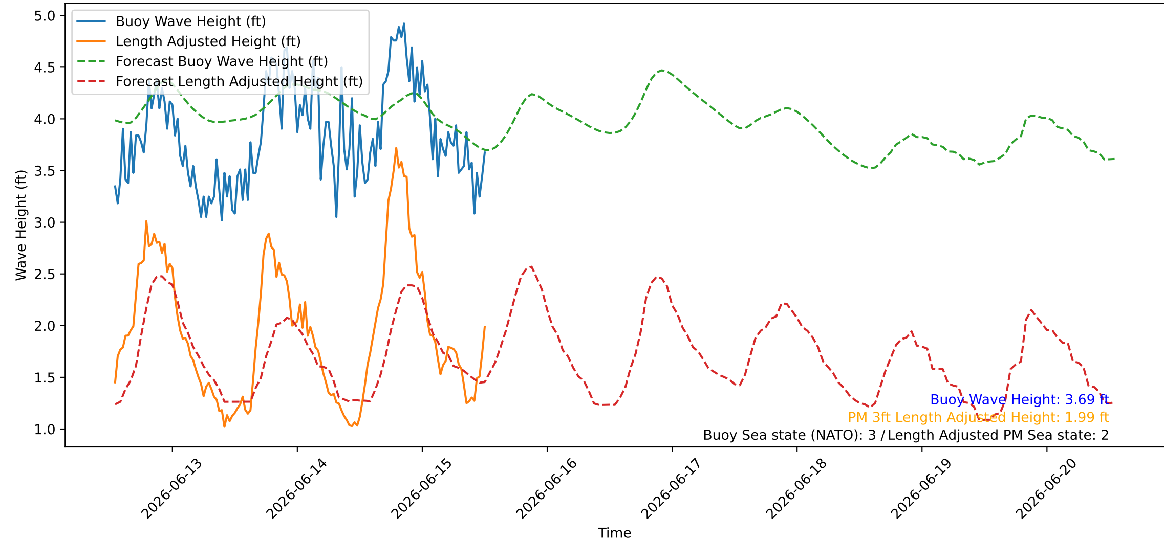
Wave Heights over Time for Green Beach at 2026-06-15 12:51:09
