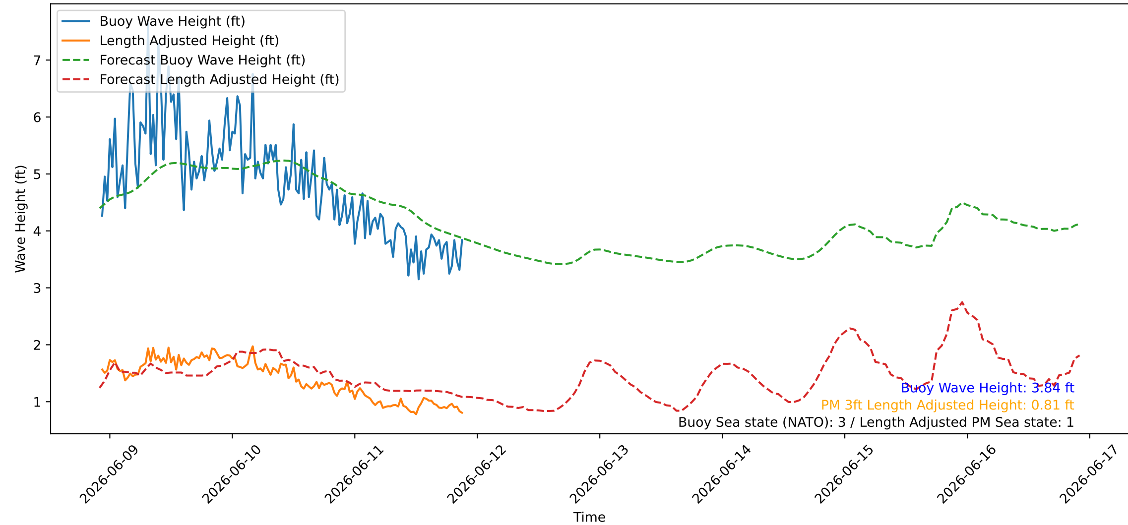
Wave Heights over Time for Red Beach at 2026-06-11 22:00:46
