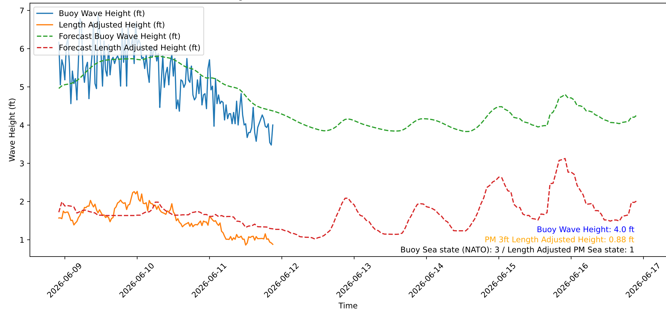
Wave Heights over Time for Green Beach at 2026-06-11 22:01:08
