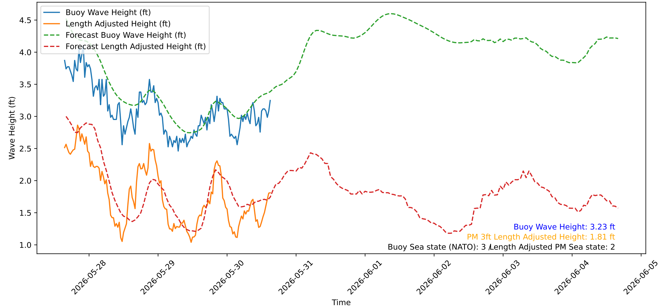
Wave Heights over Time for Green Beach at 2026-05-30 15:41:06
