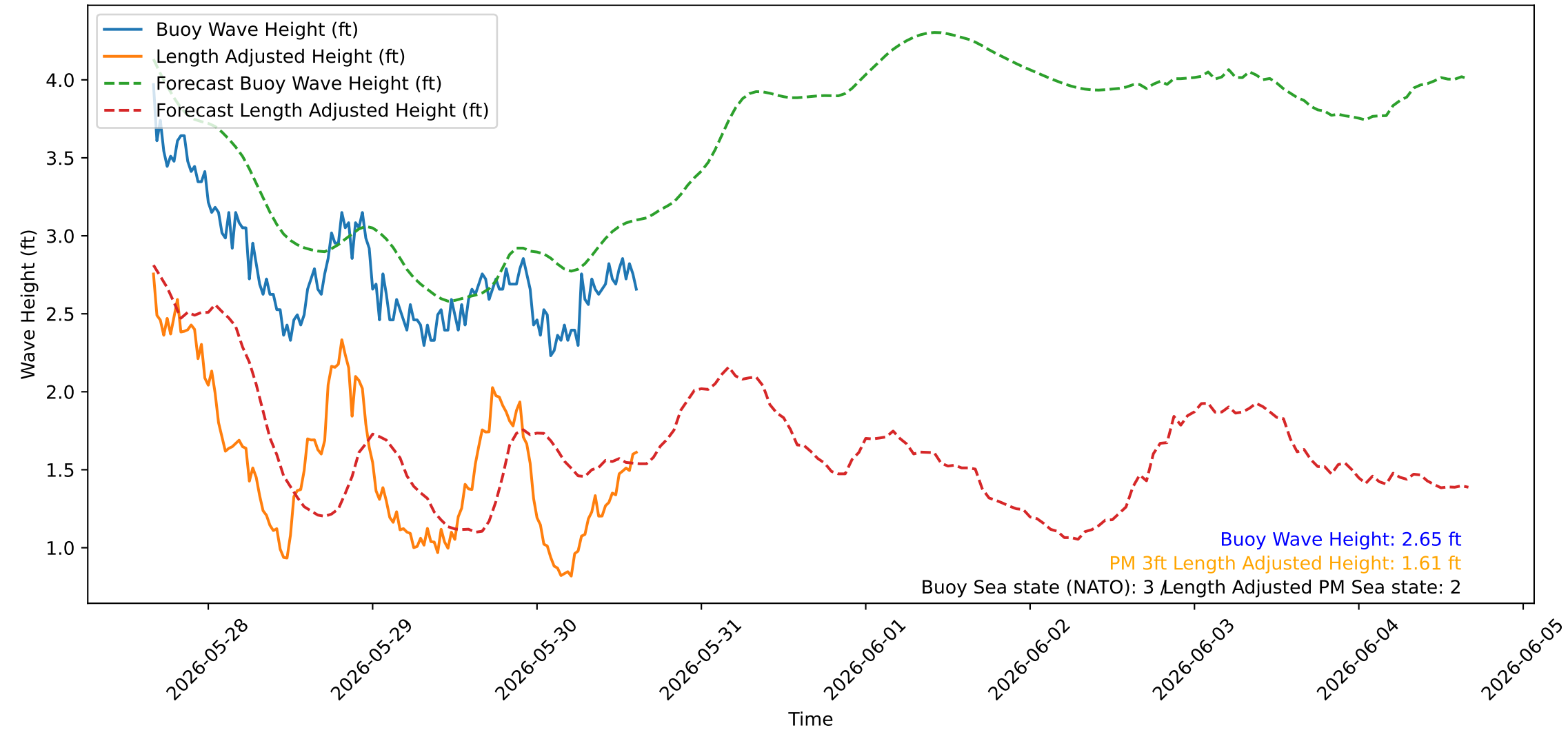
Wave Heights over Time for Red Beach at 2026-05-30 15:40:43
