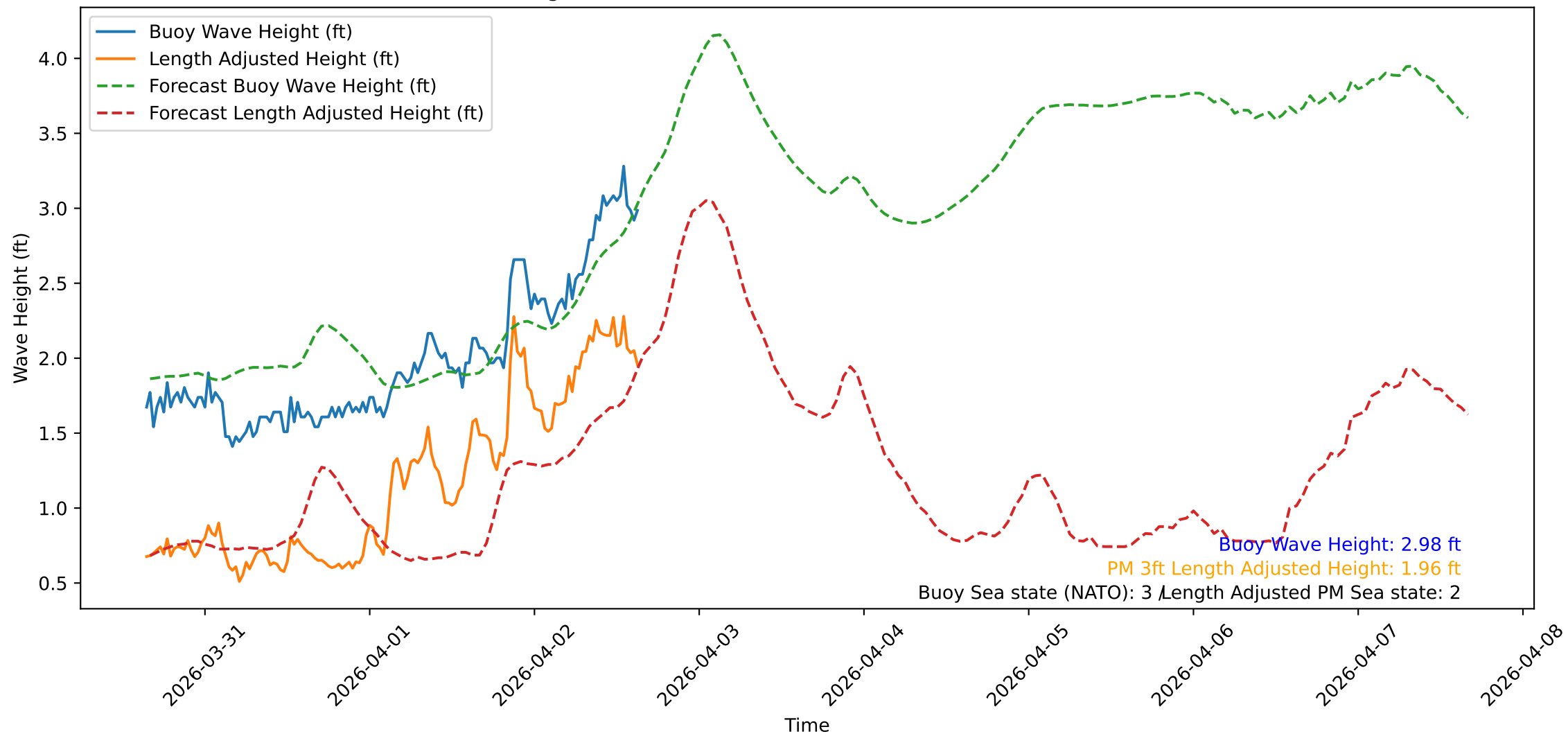
Wave Heights over Time for Green Beach at 2026-04-02 15:41:11
