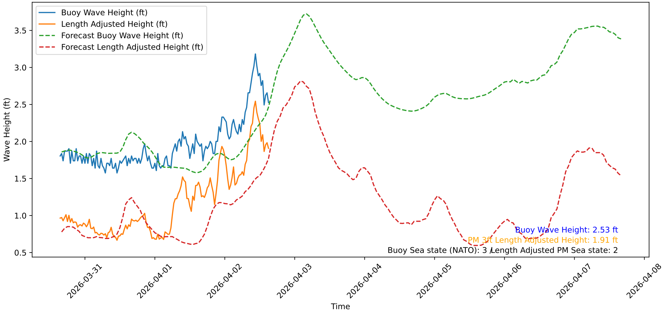
Wave Heights over Time for Oceanside Harbor at 2026-04-02 15:40:32
