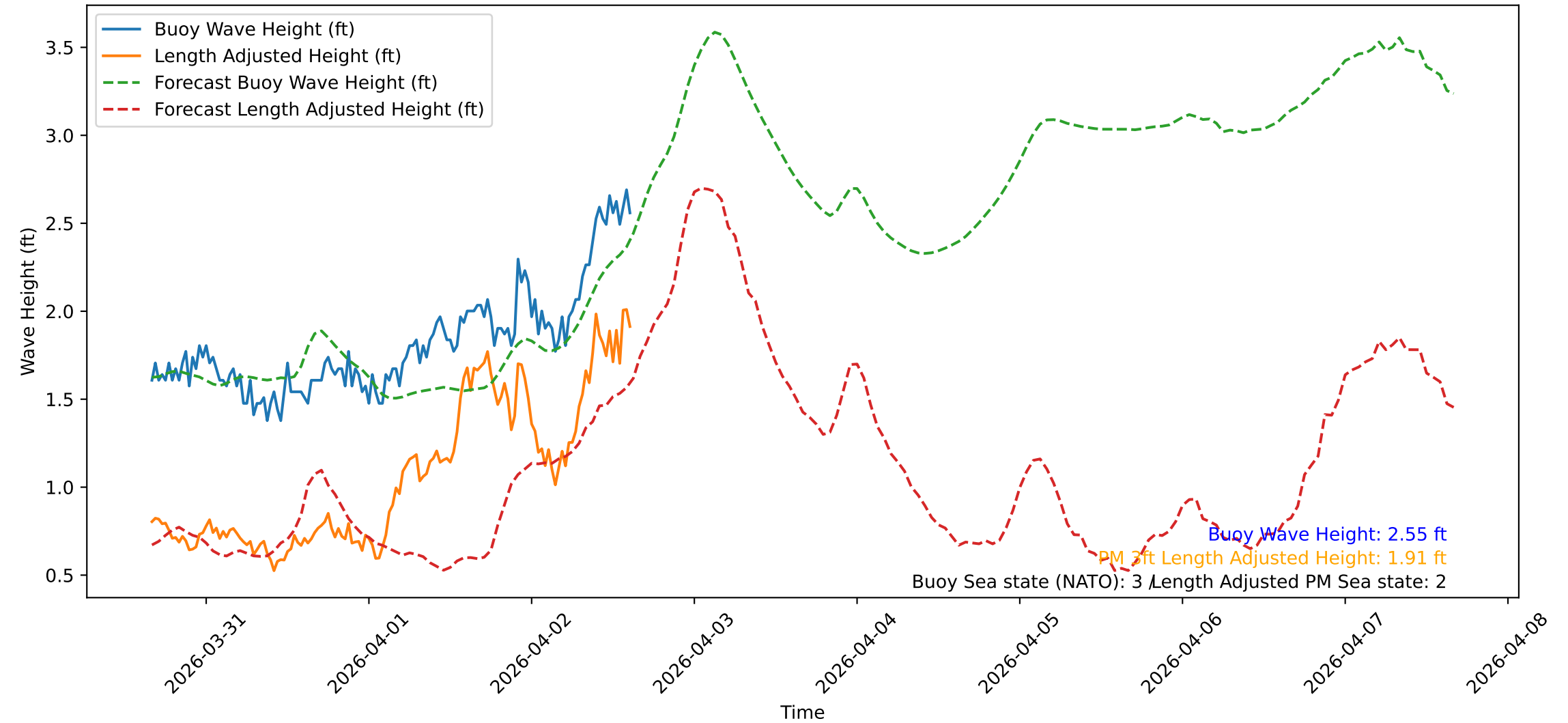
Wave Heights over Time for Red Beach at 2026-04-02 15:40:48
