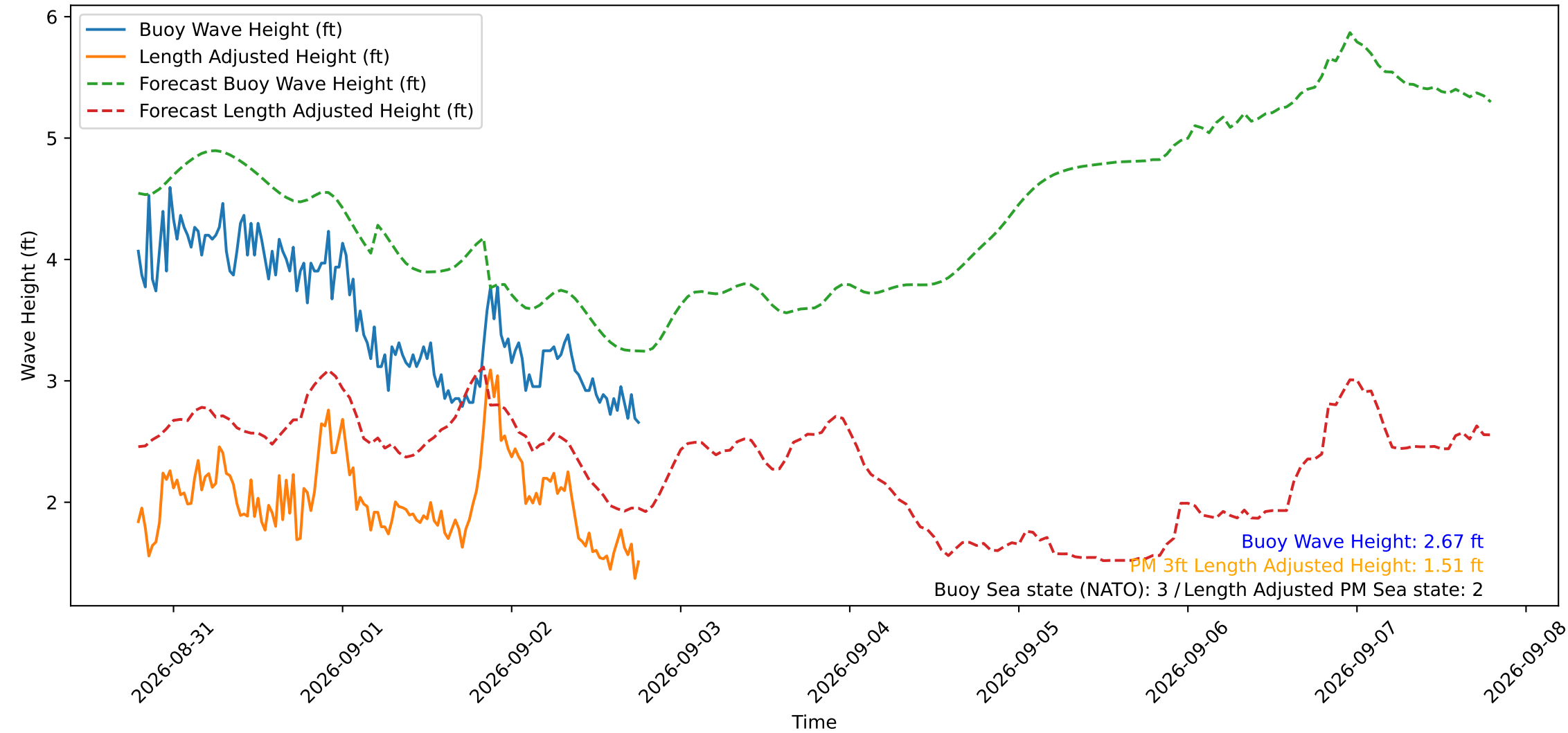
Wave Heights over Time for Green Beach at 2026-09-02 18:51:15
