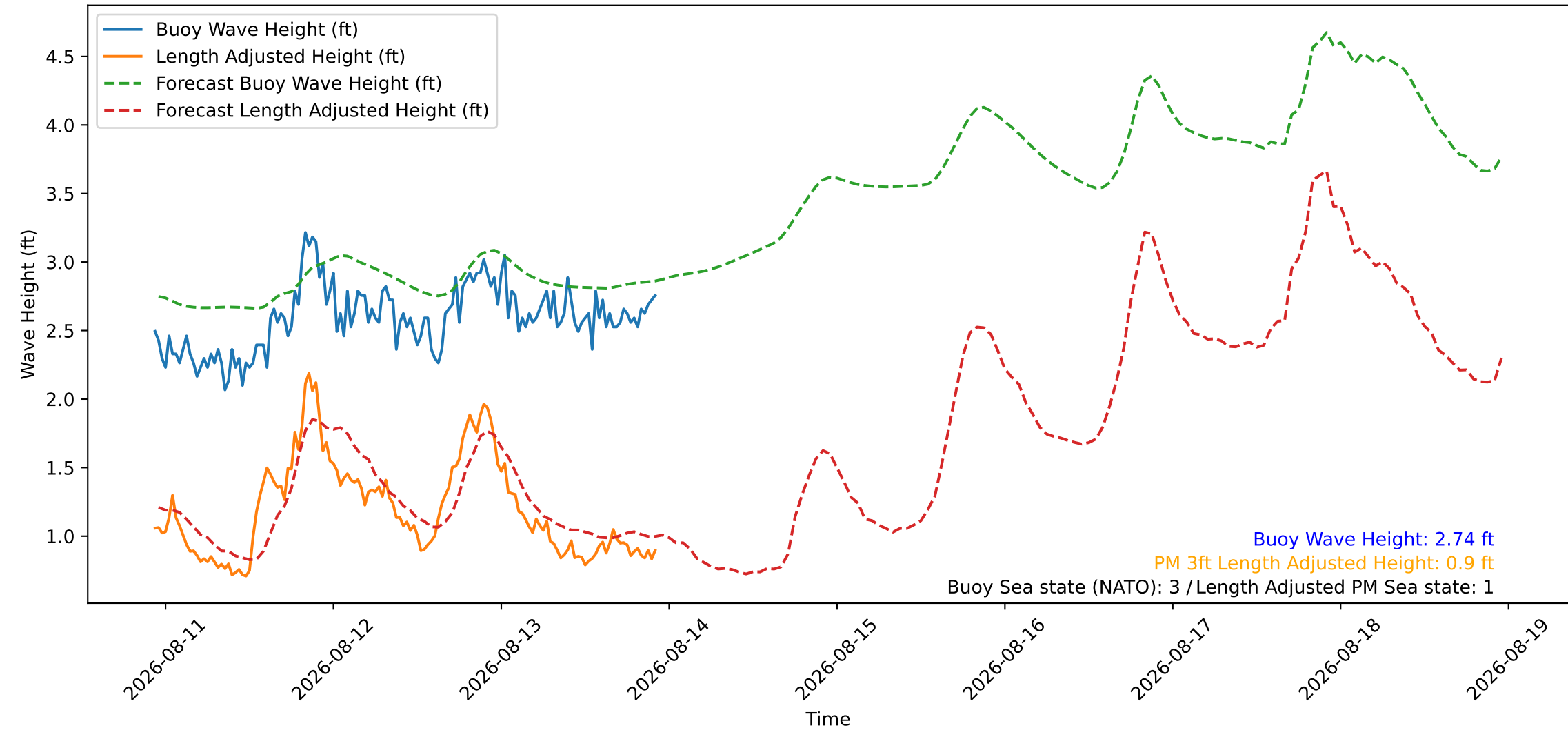
Wave Heights over Time for Green Beach at 2026-08-13 22:41:09
