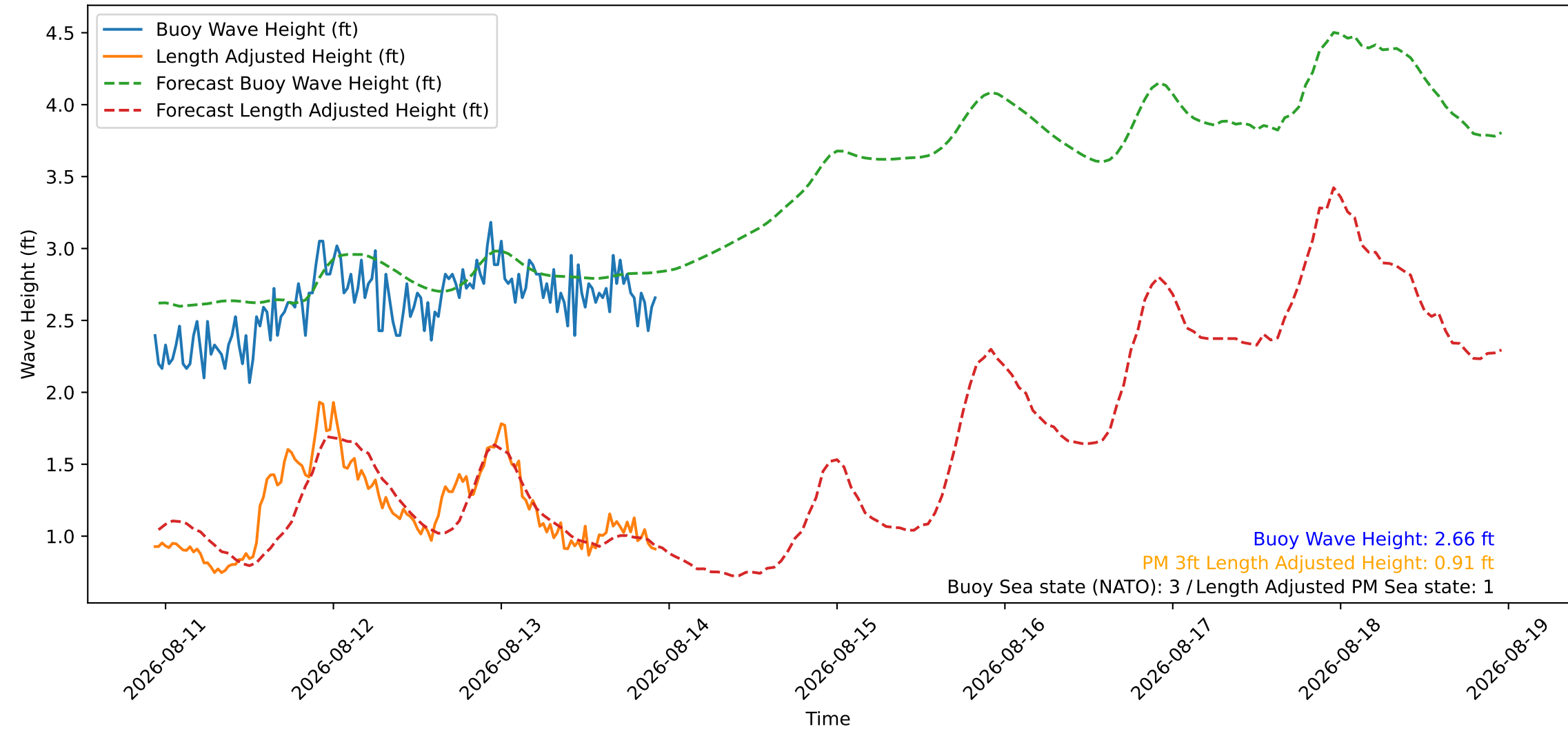
Wave Heights over Time for Oceanside Harbor at 2026-08-13 22:40:27
