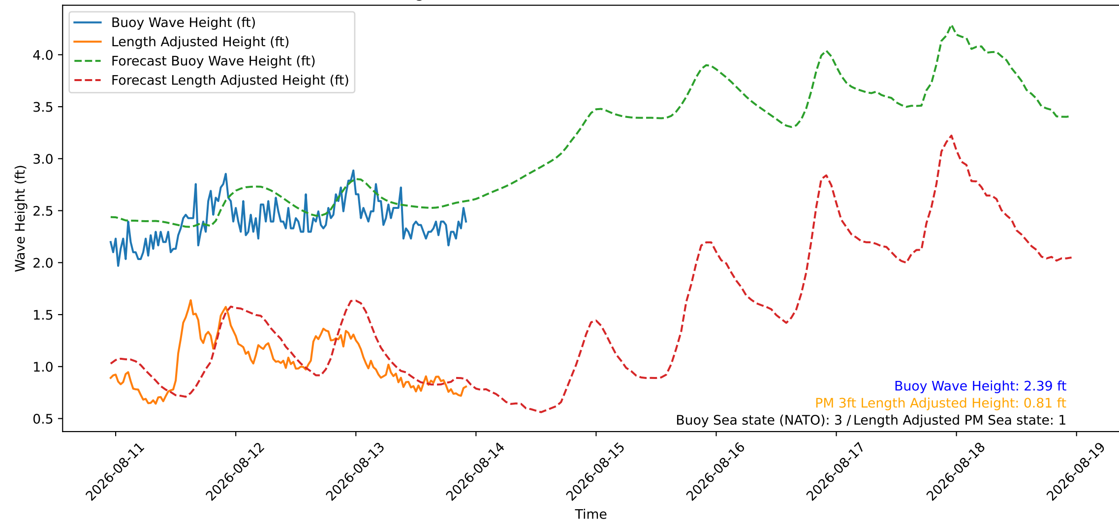
Wave Heights over Time for Red Beach at 2026-08-13 22:40:46
