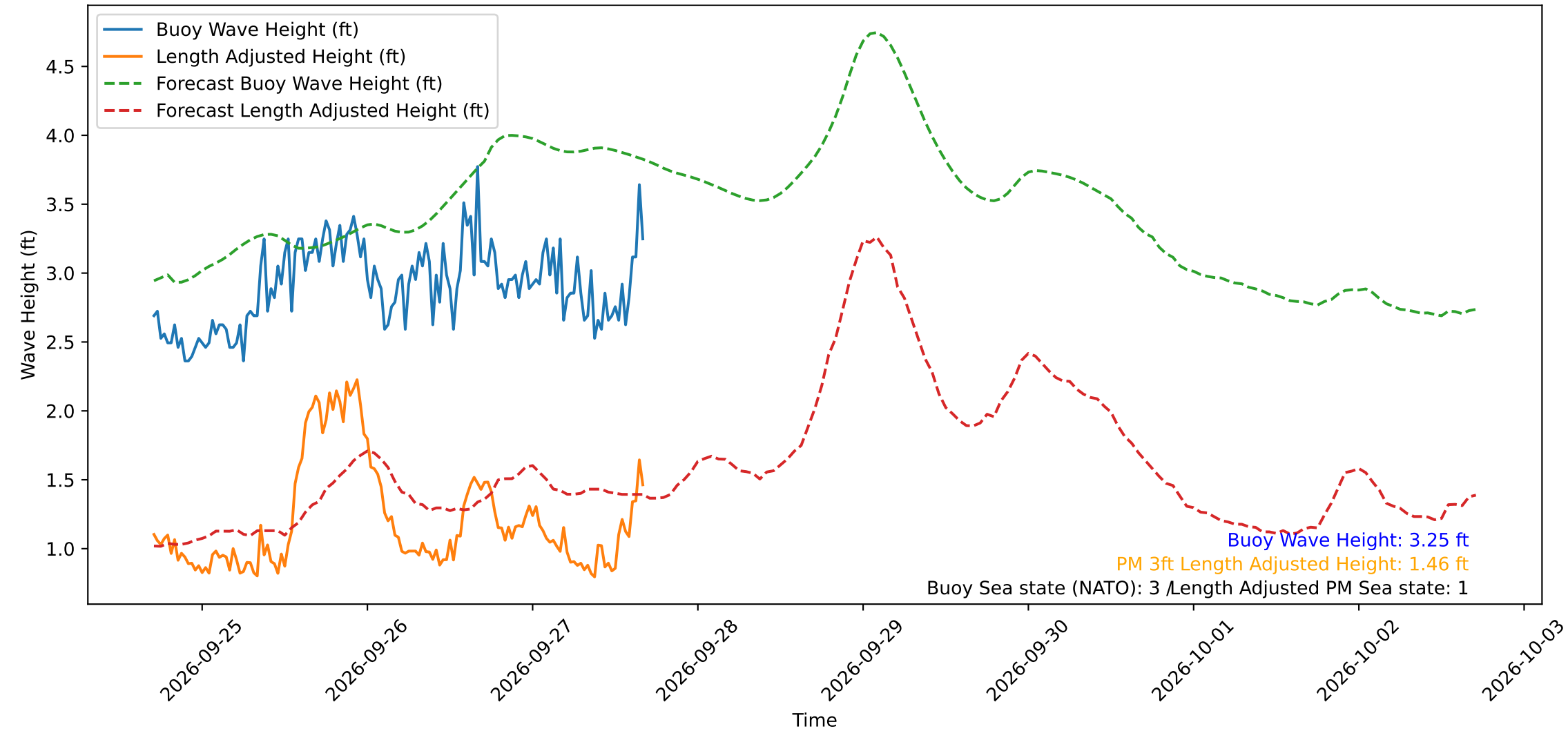
Wave Heights over Time for Oceanside Harbor at 2026-09-27 17:00:30
