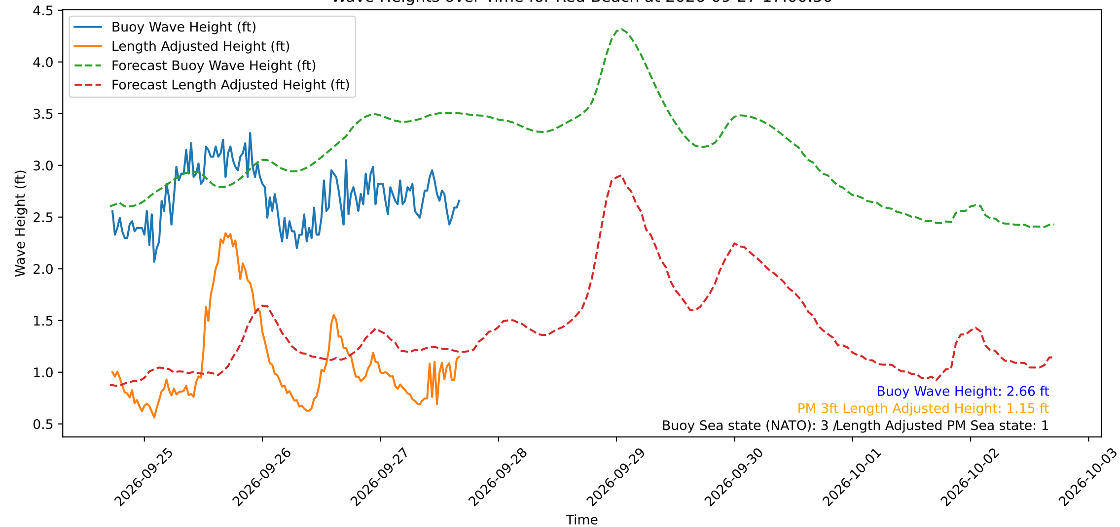
Wave Heights over Time for Red Beach at 2026-09-27 17:00:50
