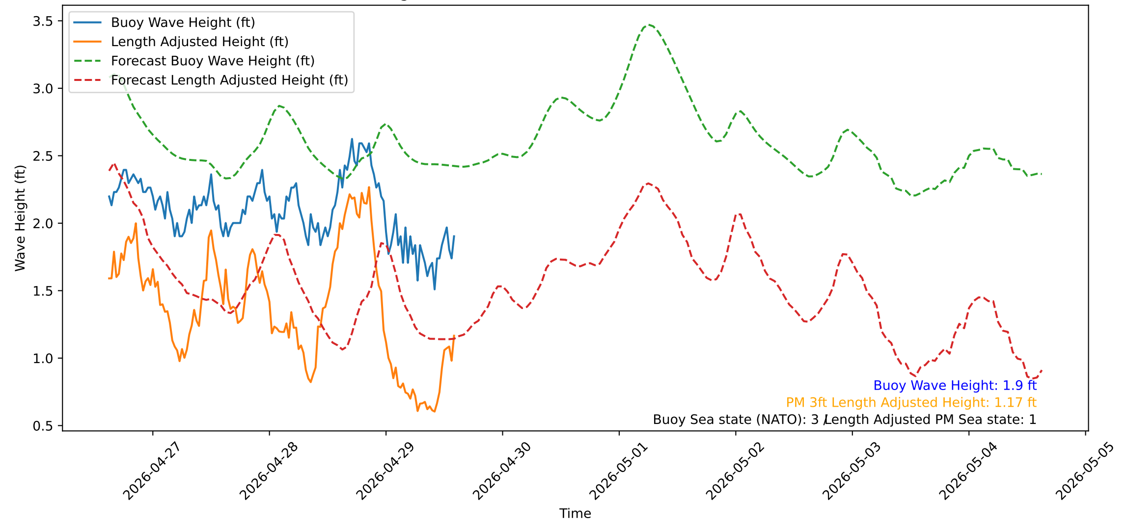
Wave Heights over Time for Red Beach at 2026-04-29 14:50:51
