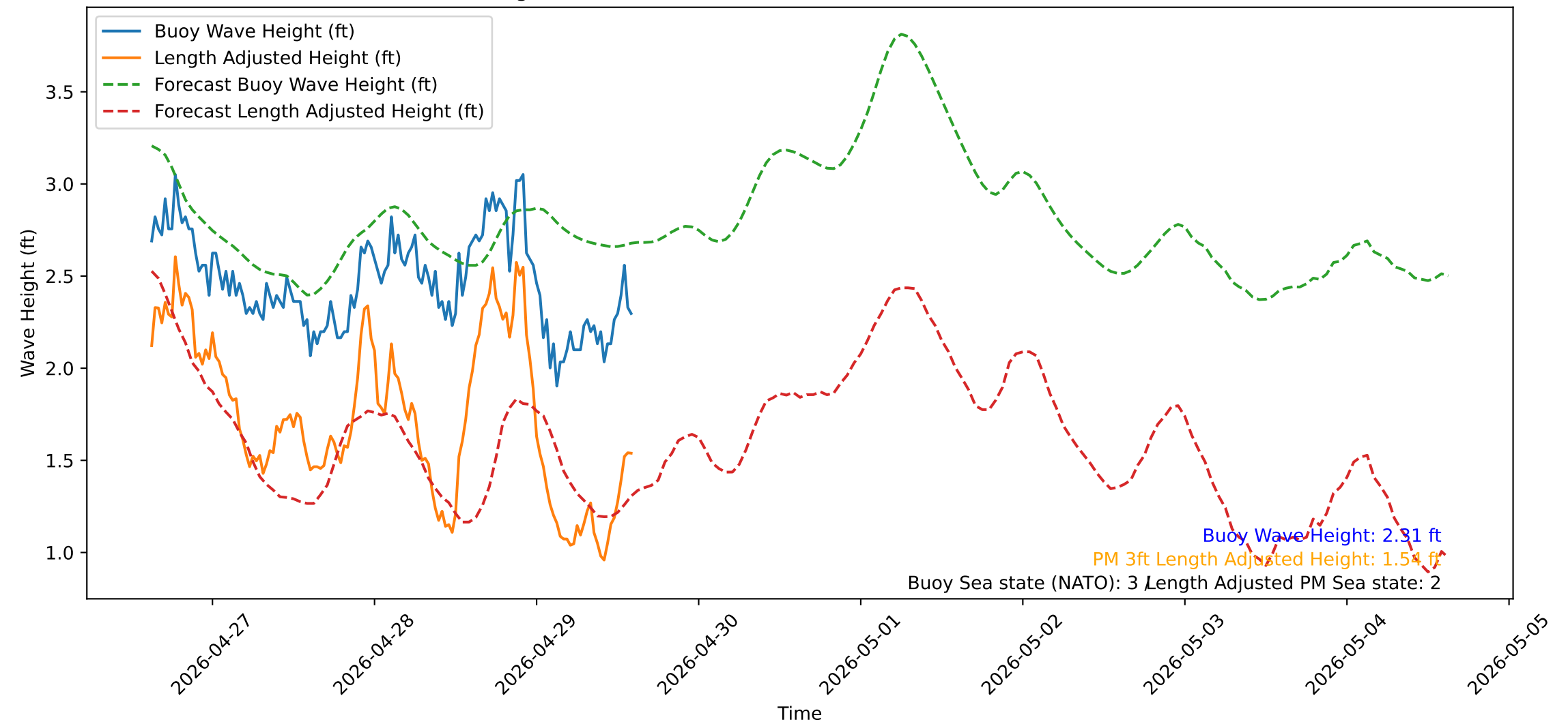
Wave Heights over Time for Oceanside Harbor at 2026-04-29 14:50:31
