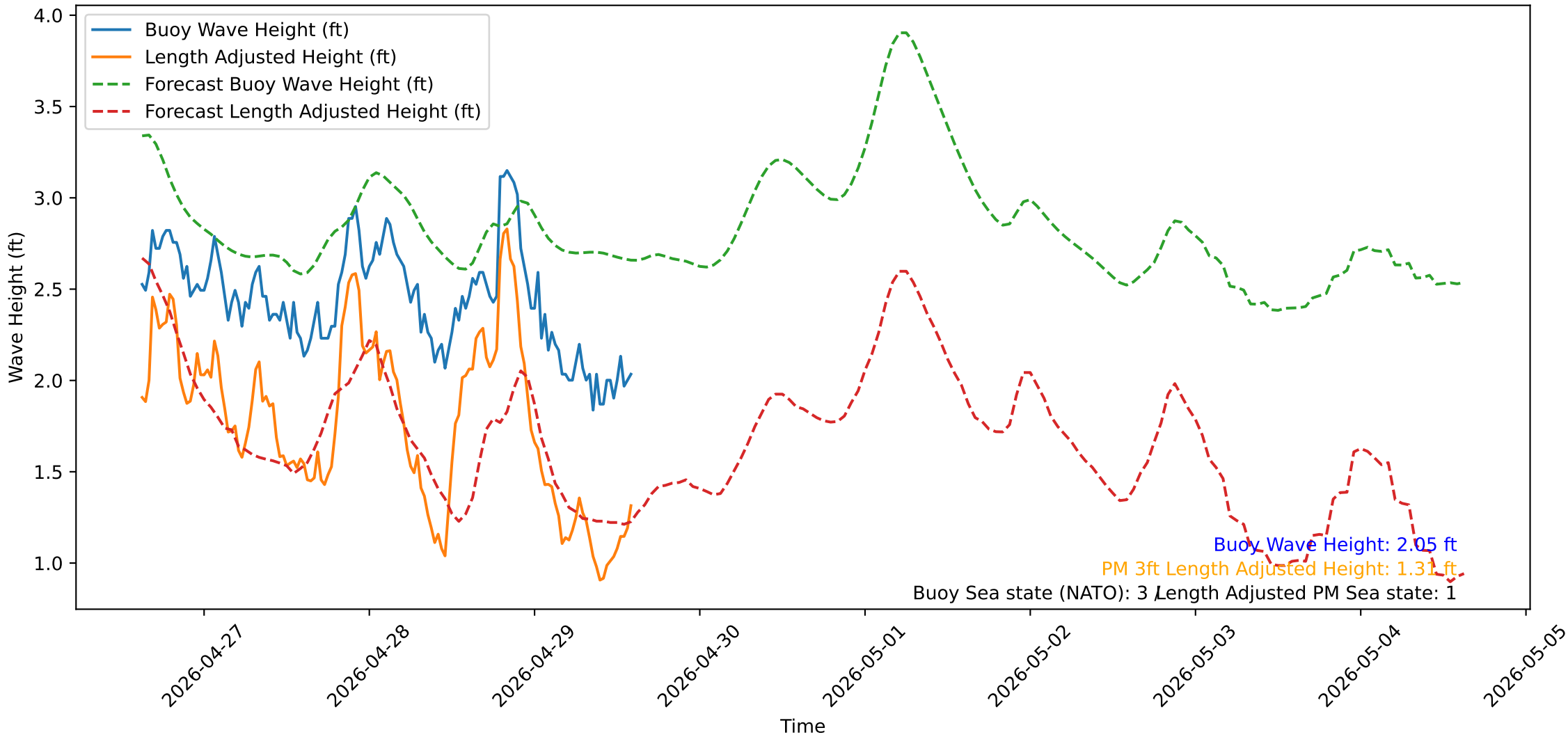
Wave Heights over Time for Green Beach at 2026-04-29 14:51:14
