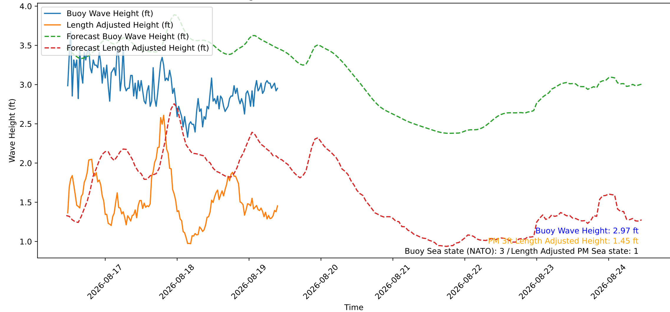
Wave Heights over Time for Red Beach at 2026-08-19 11:00:46
