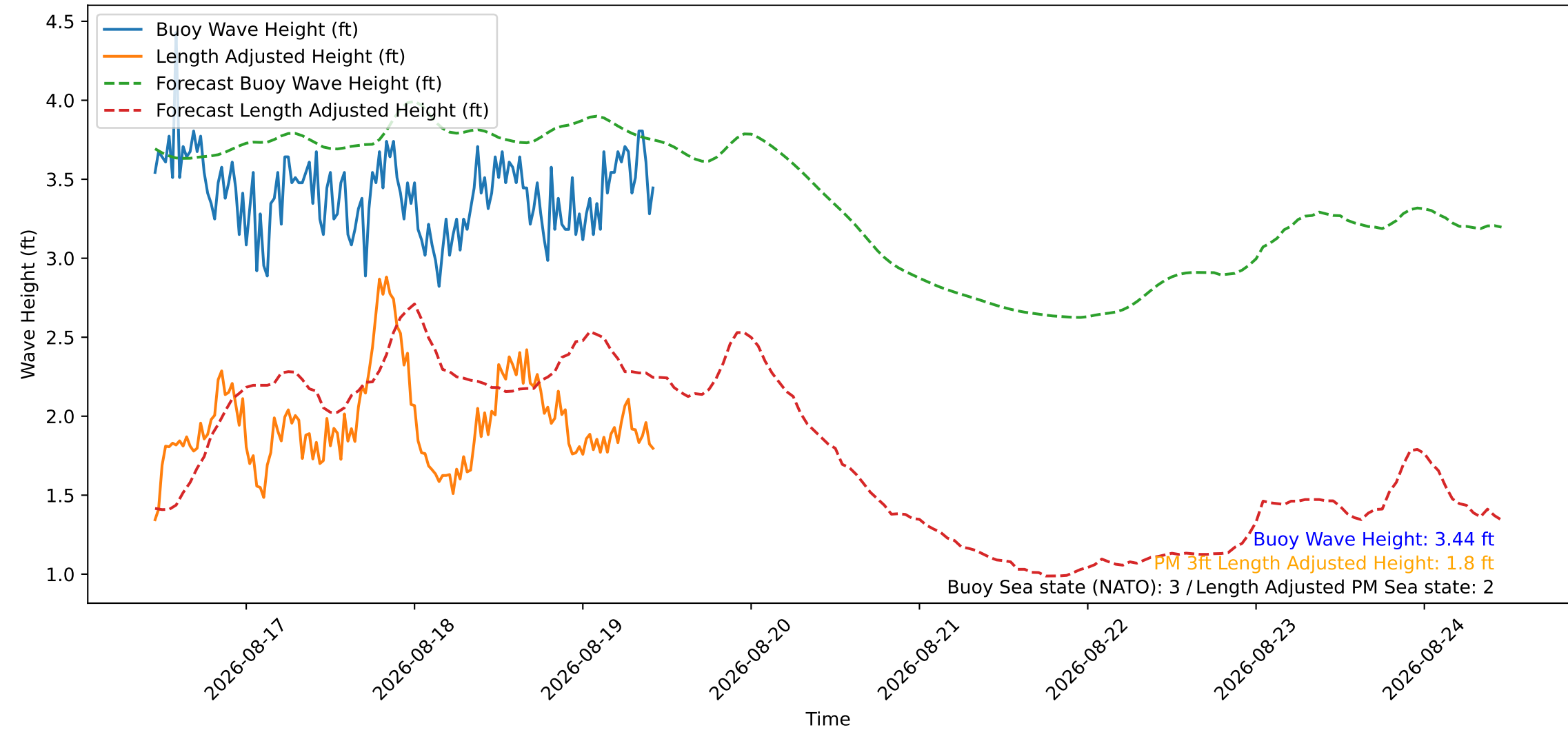
Wave Heights over Time for Oceanside Harbor at 2026-08-19 11:00:26
