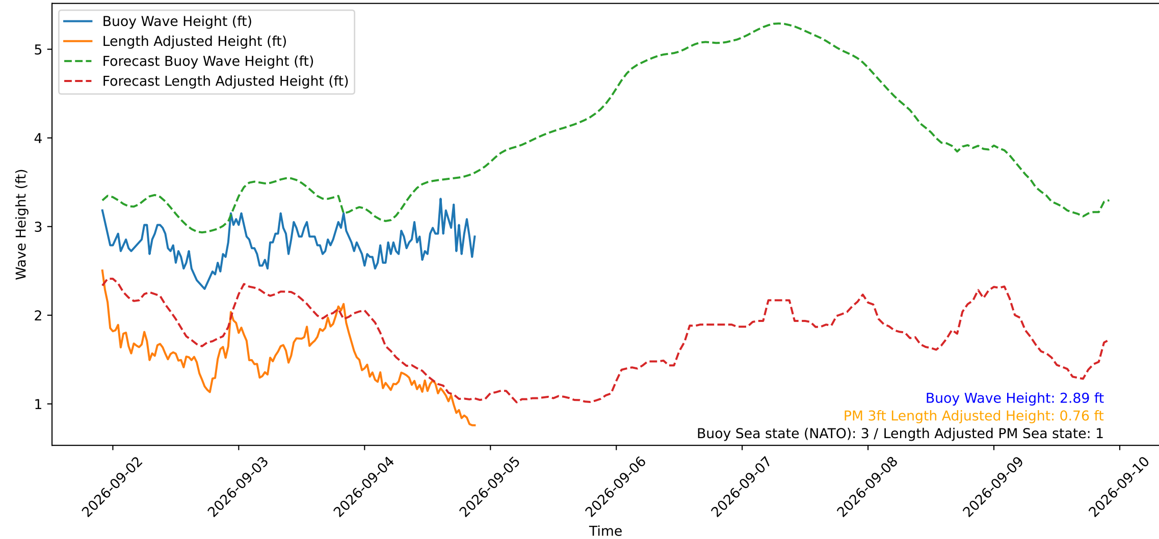
Wave Heights over Time for Red Beach at 2026-09-04 21:40:50
