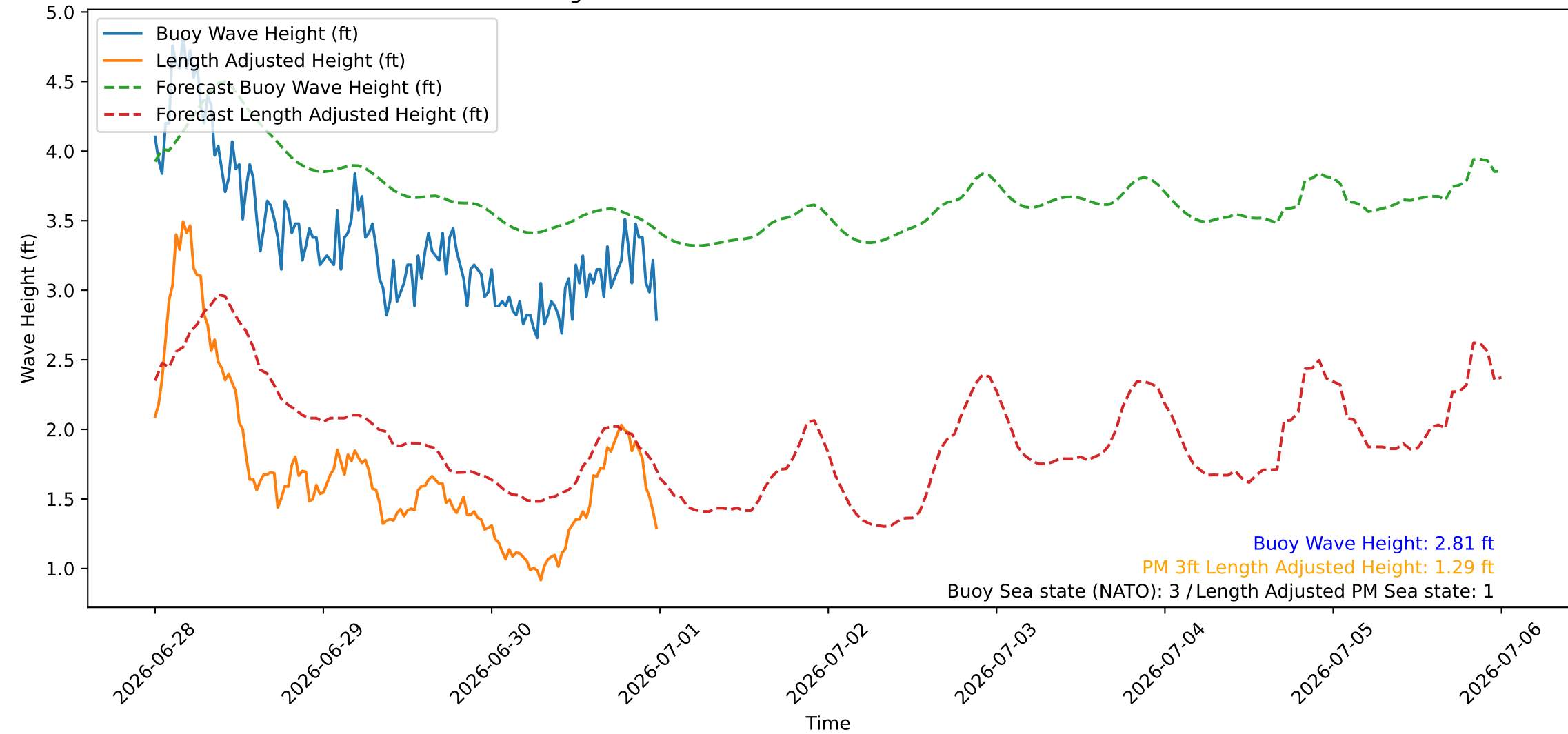
Wave Heights over Time for Green Beach at 2026-07-01 00:11:08
