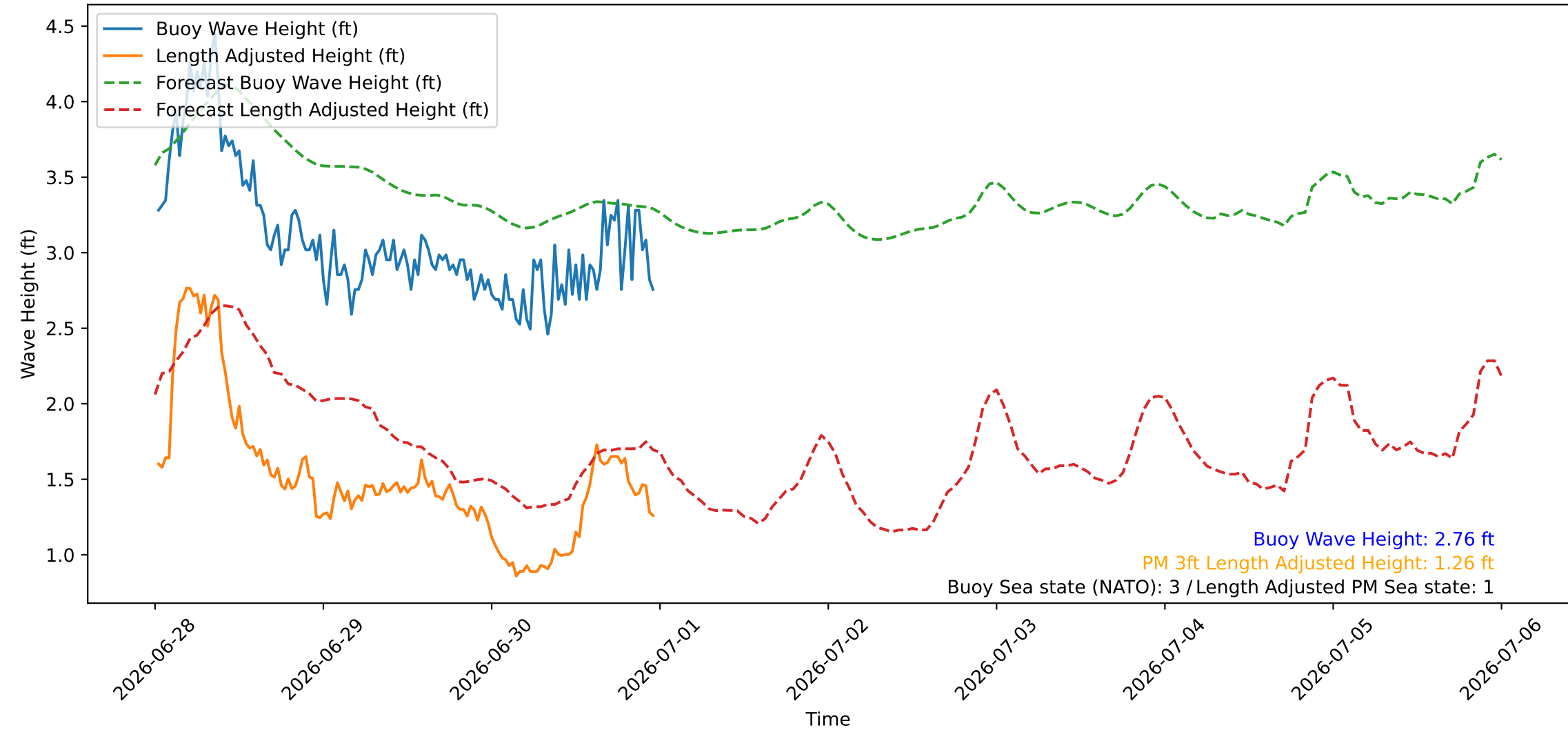
Wave Heights over Time for Red Beach at 2026-07-01 00:10:45
