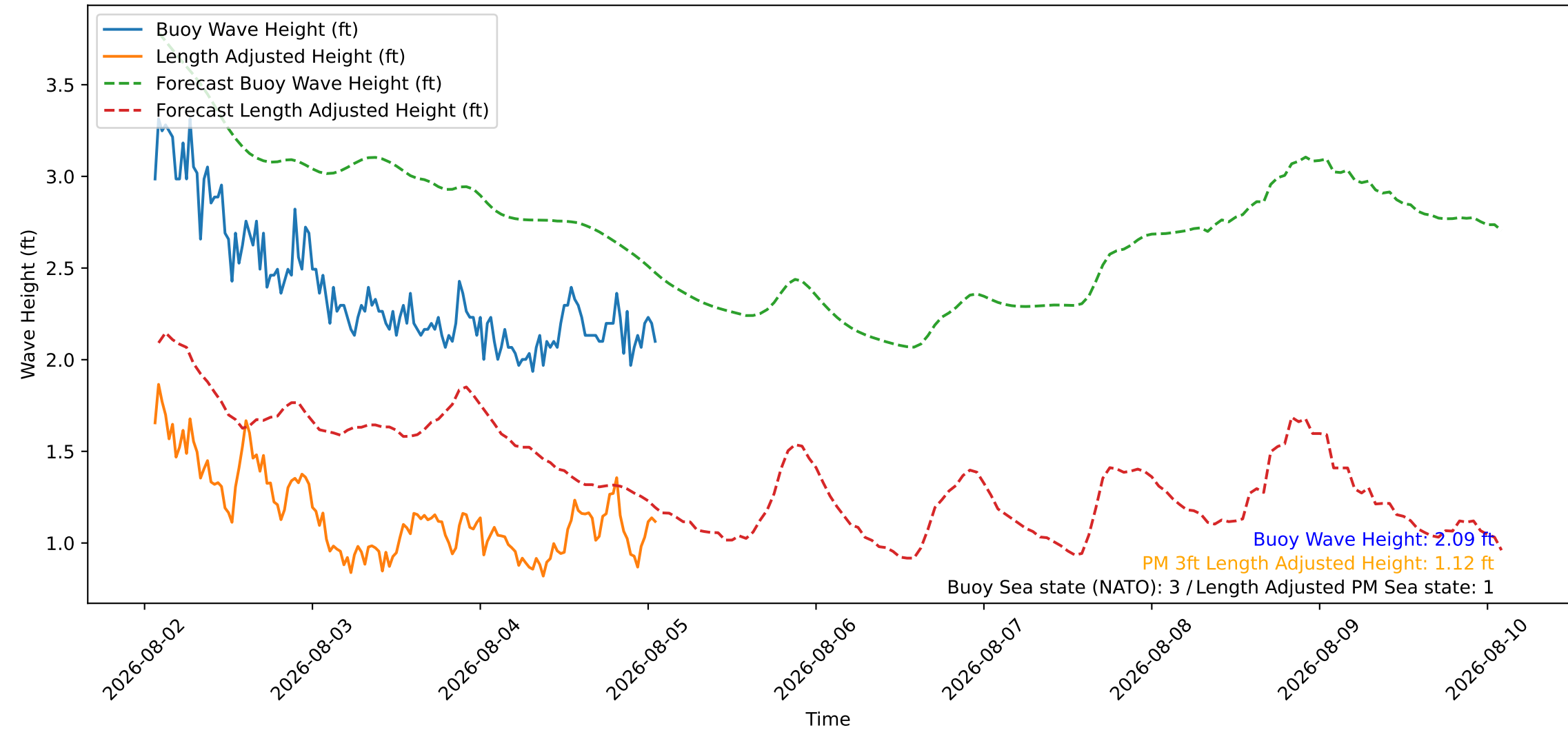
Wave Heights over Time for Green Beach at 2026-08-05 01:41:09
