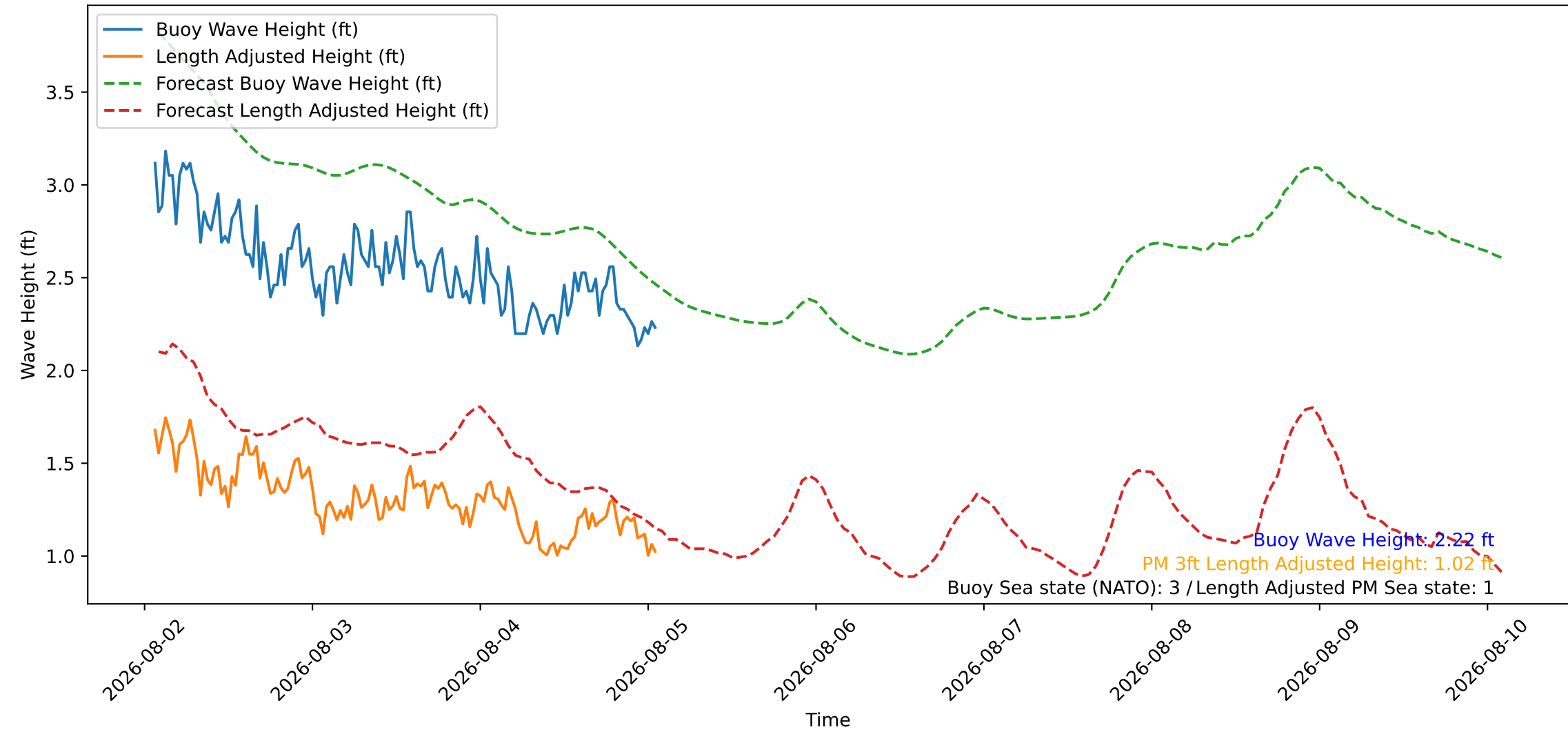
Wave Heights over Time for Oceanside Harbor at 2026-08-05 01:40:27
