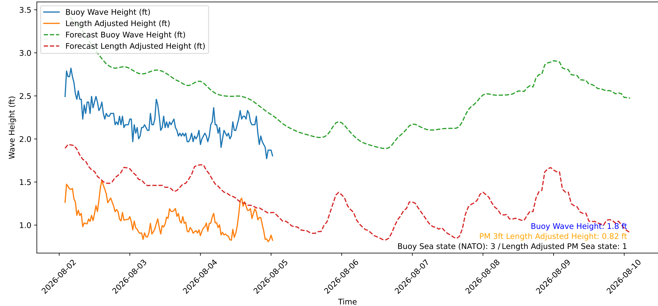
Wave Heights over Time for Red Beach at 2026-08-05 01:40:46
