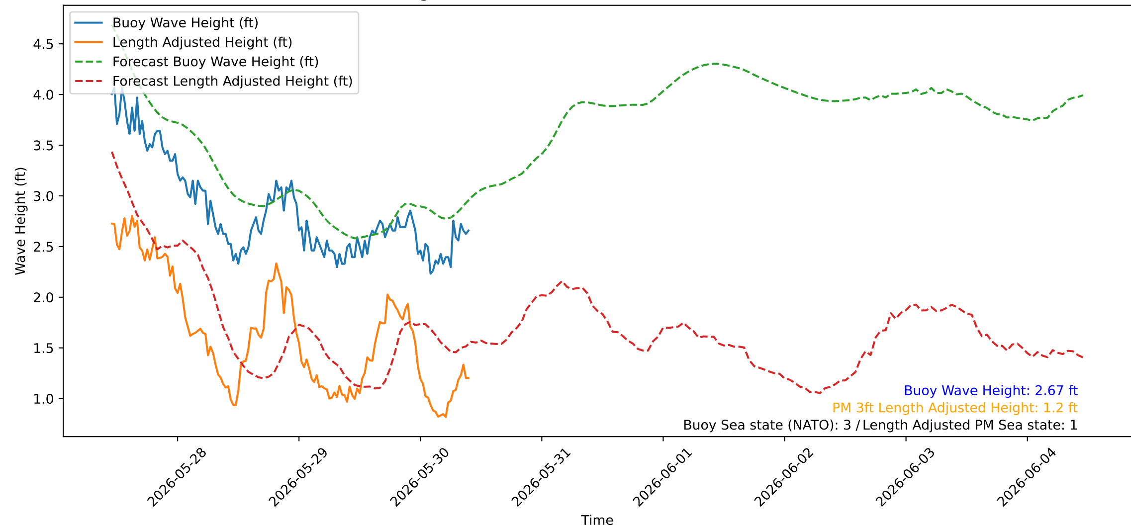
Wave Heights over Time for Red Beach at 2026-05-30 10:40:43
