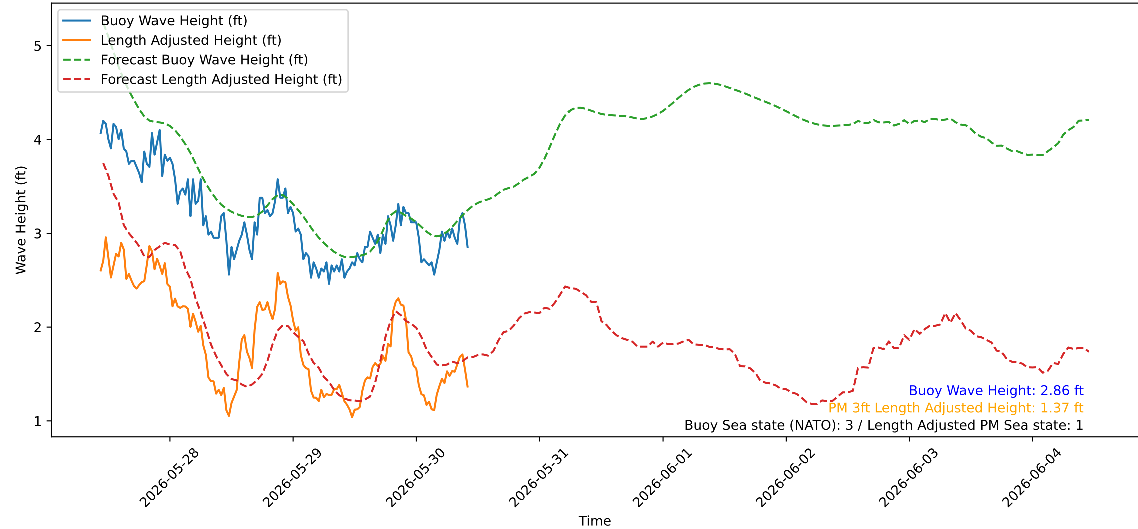
Wave Heights over Time for Green Beach at 2026-05-30 10:41:06
