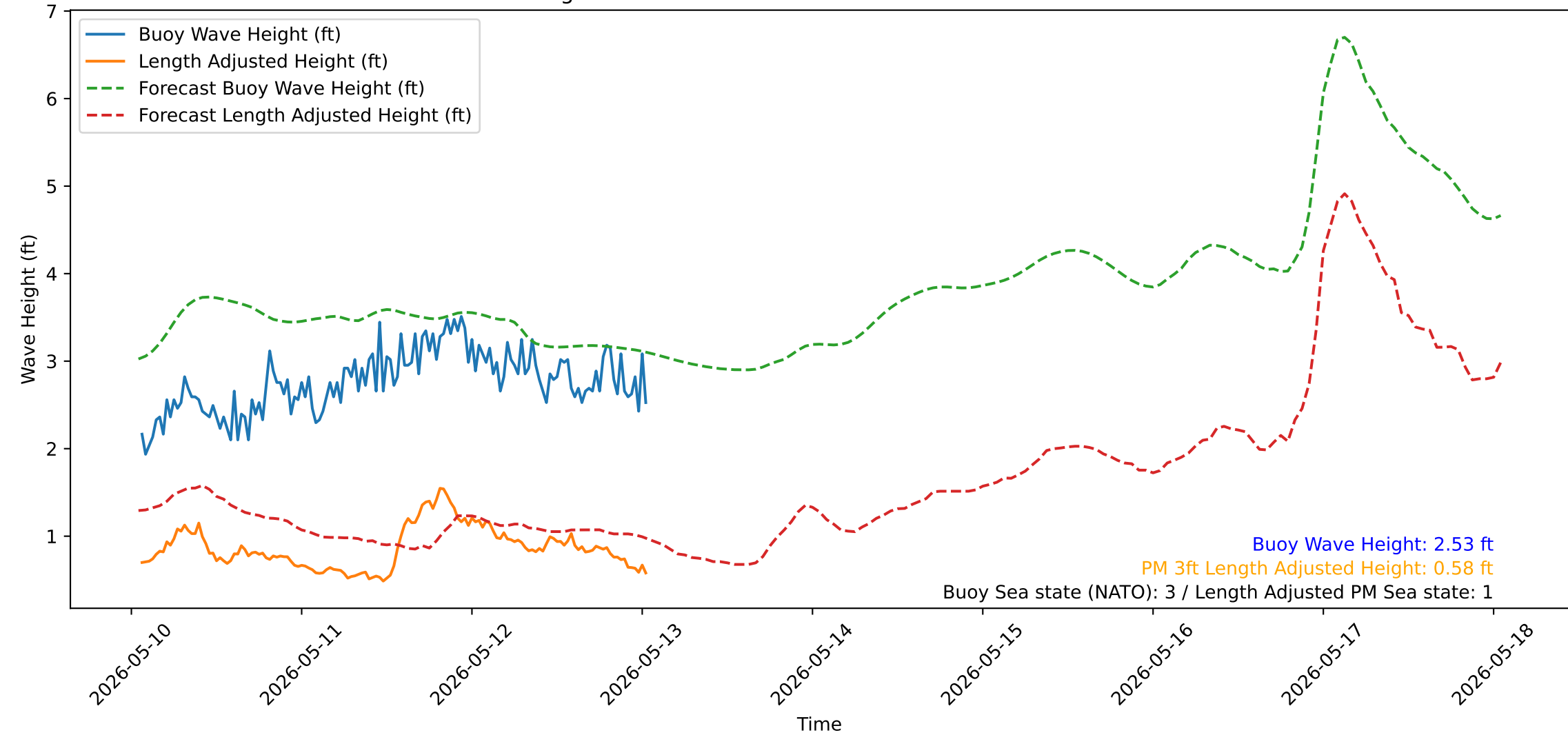
Wave Heights over Time for Green Beach at 2026-05-13 01:21:14
