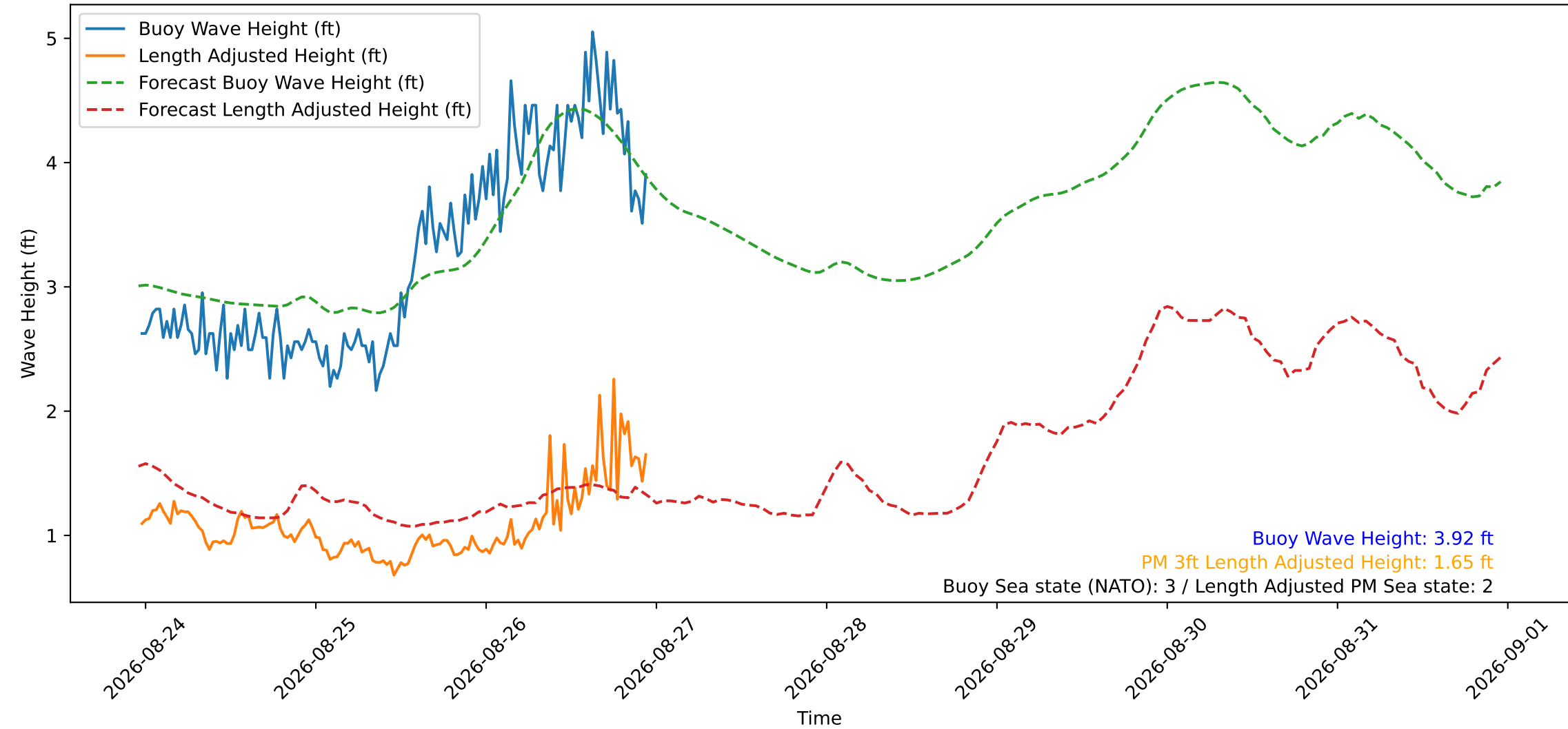
Wave Heights over Time for Red Beach at 2026-08-26 23:20:50
