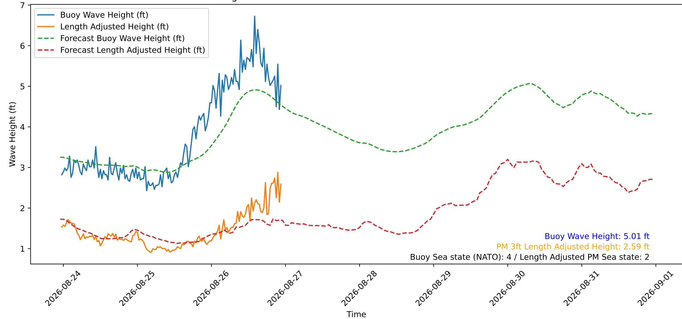
Wave Heights over Time for Oceanside Harbor at 2026-08-26 23:20:29
