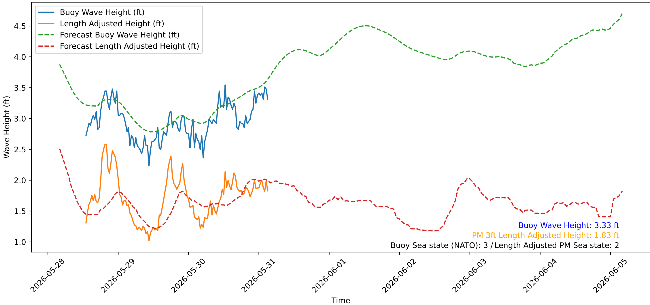
Wave Heights over Time for Oceanside Harbor at 2026-05-31 03:50:25
