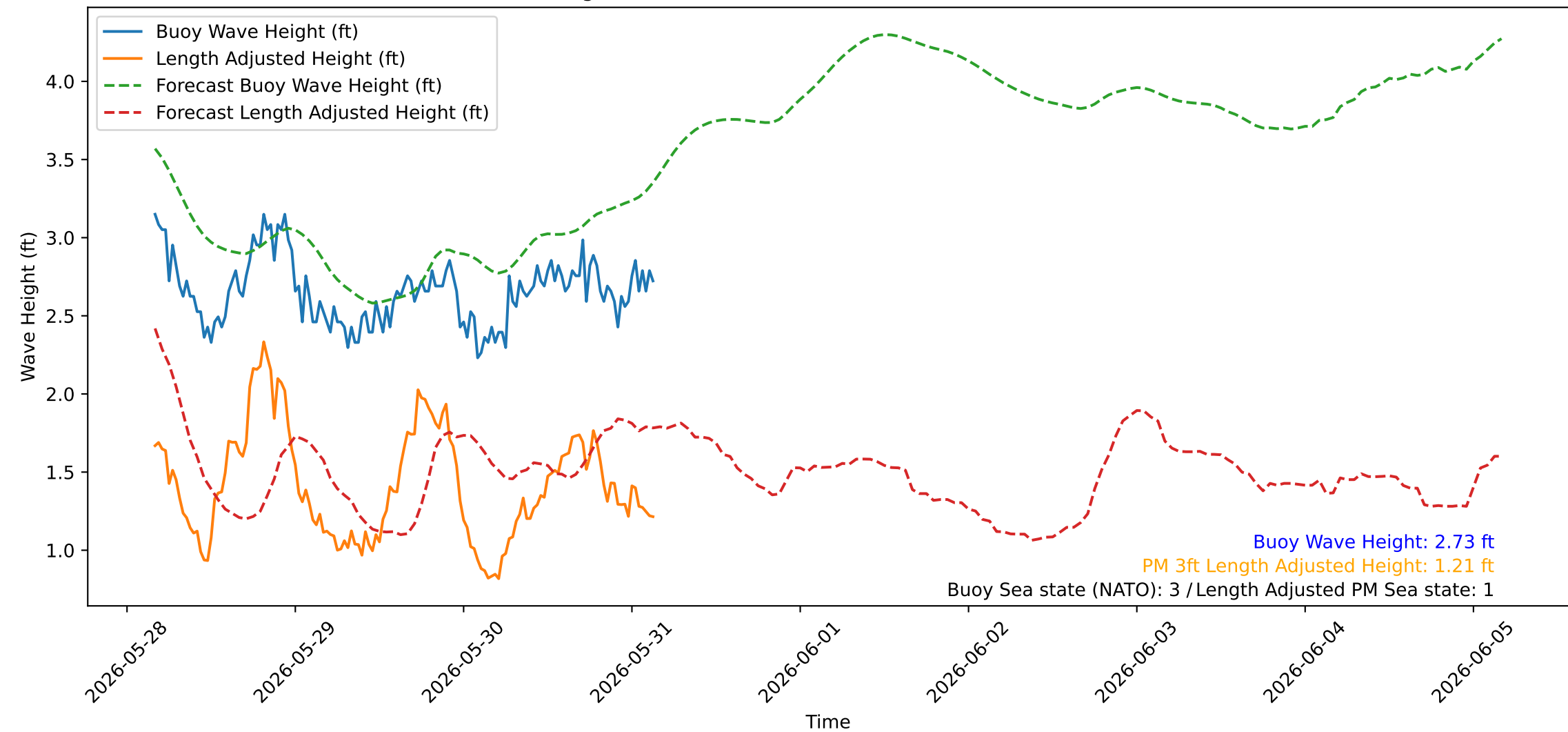
Wave Heights over Time for Red Beach at 2026-05-31 03:50:45
