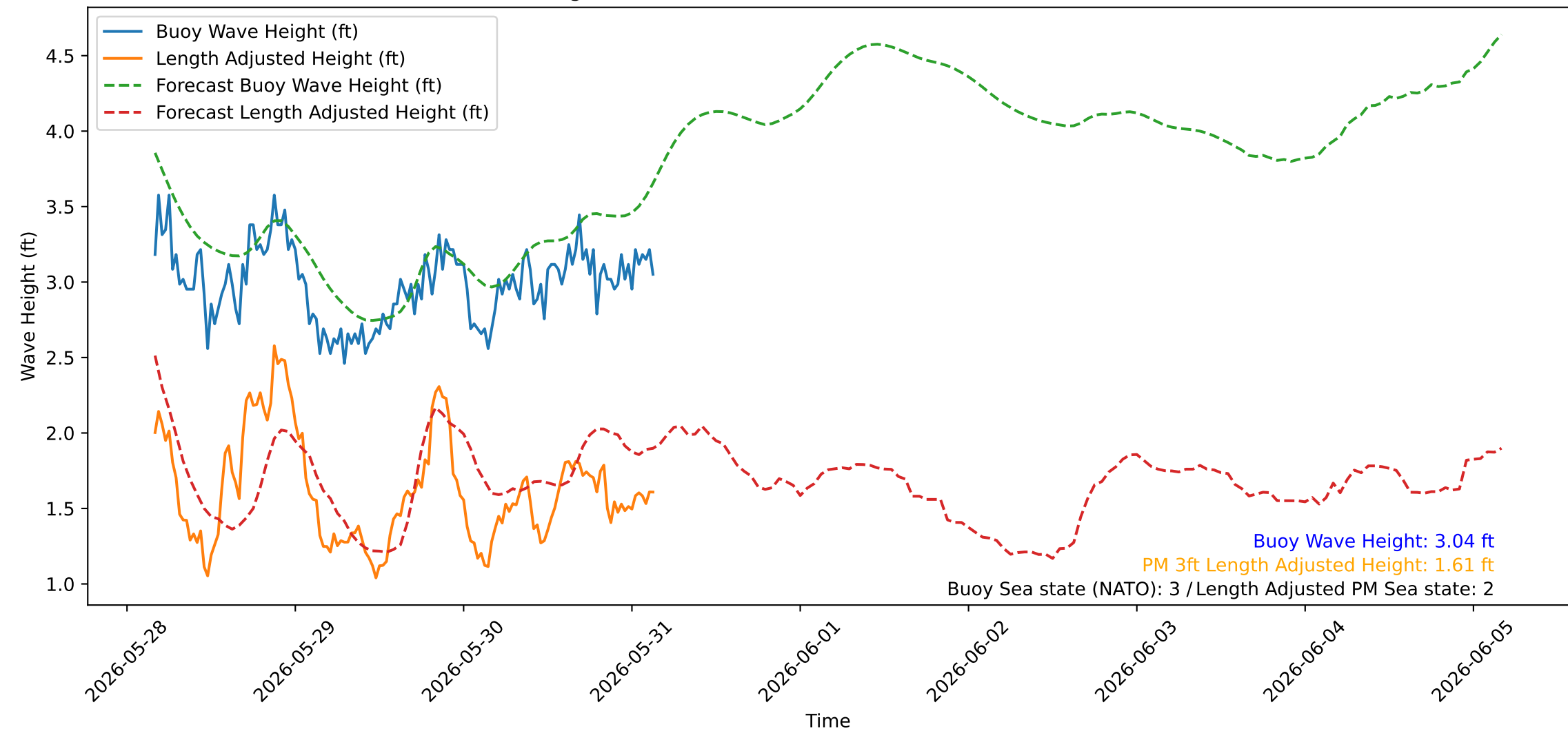
Wave Heights over Time for Green Beach at 2026-05-31 03:51:08
