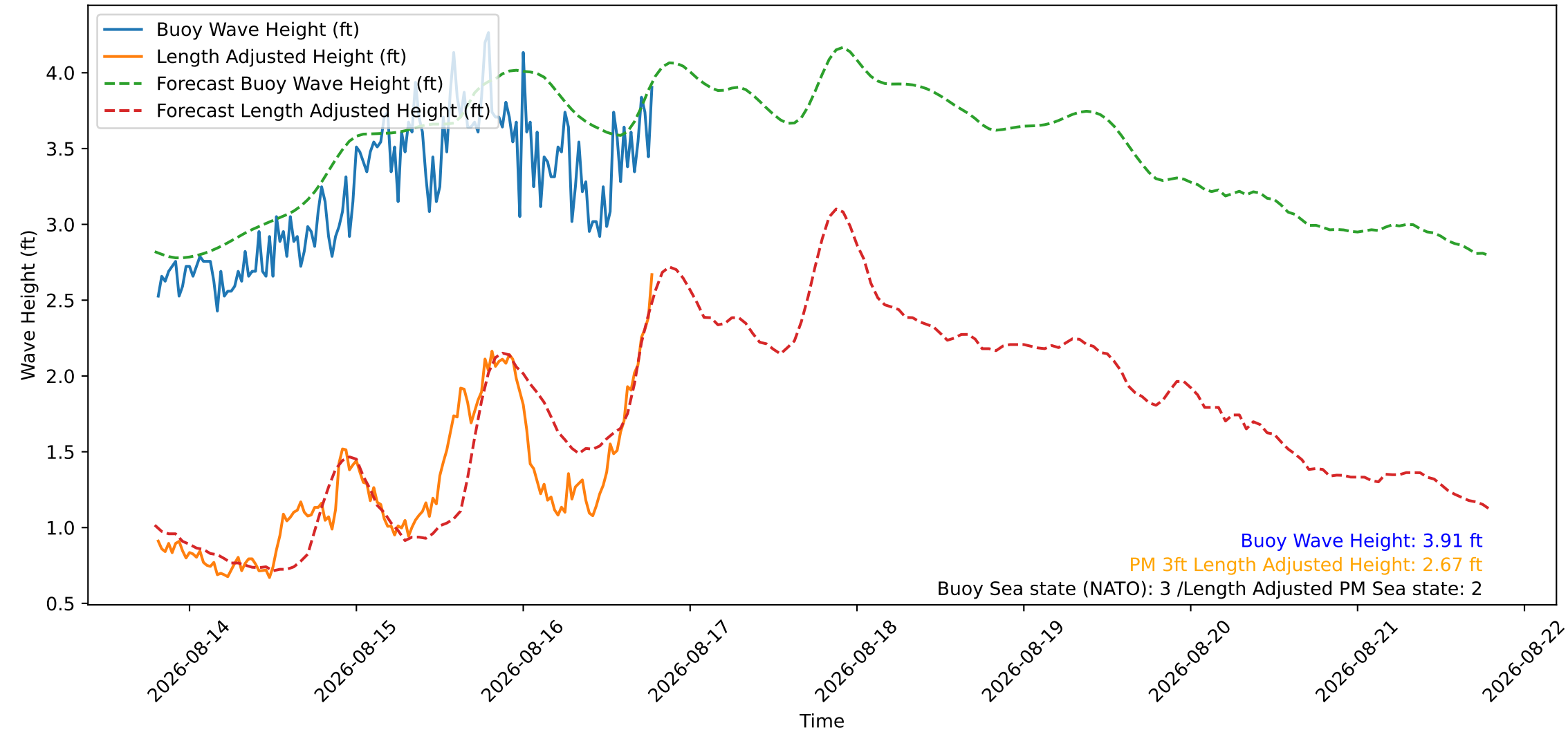
Wave Heights over Time for Green Beach at 2026-08-16 19:21:10
