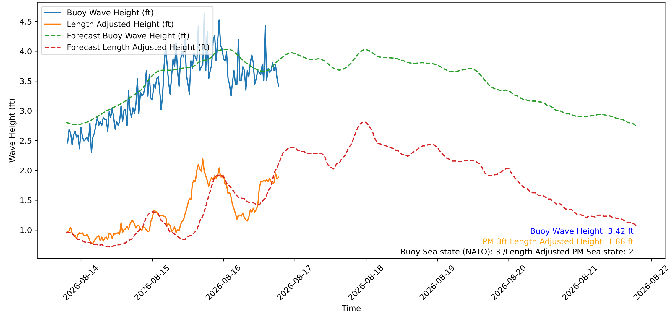
Wave Heights over Time for Oceanside Harbor at 2026-08-16 19:20:26
