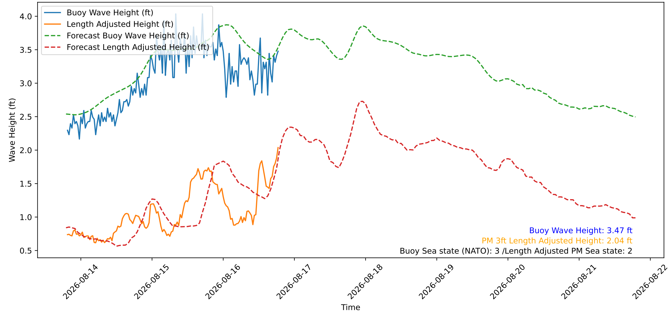
Wave Heights over Time for Red Beach at 2026-08-16 19:20:46
