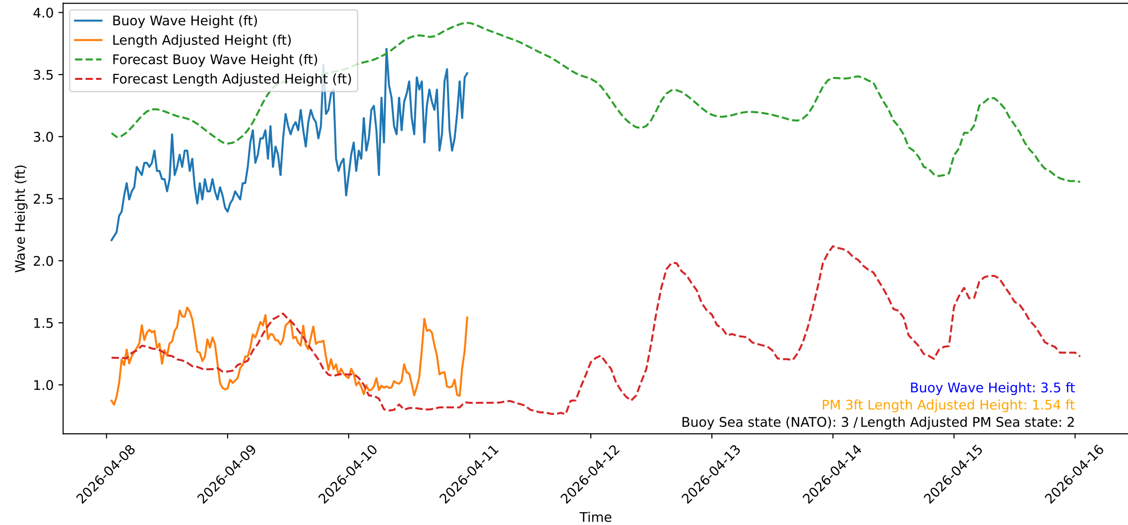
Wave Heights over Time for Red Beach at 2026-04-11 00:30:51
