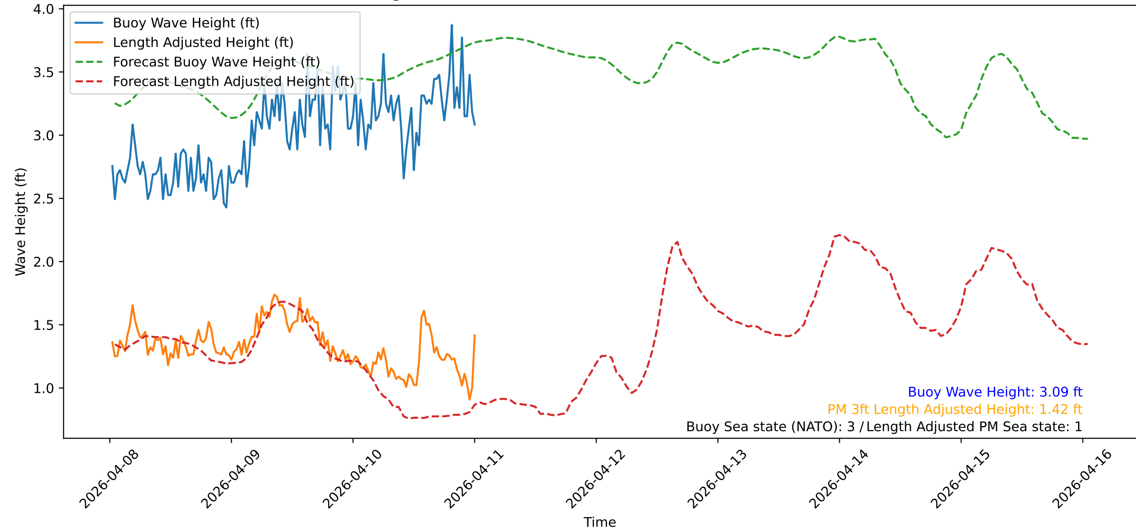
Wave Heights over Time for Oceanside Harbor at 2026-04-11 00:30:32
