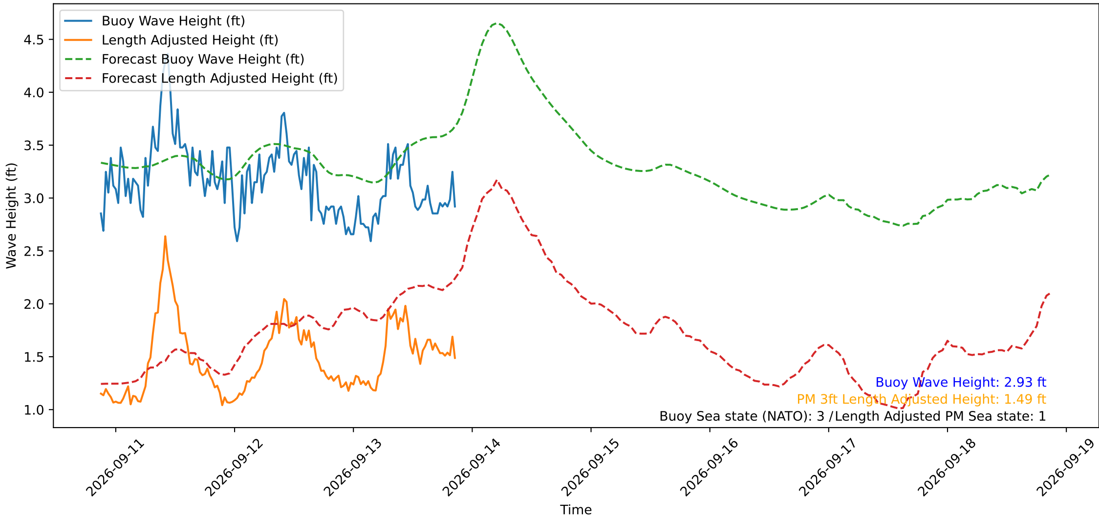
Wave Heights over Time for Oceanside Harbor at 2026-09-13 21:10:30
