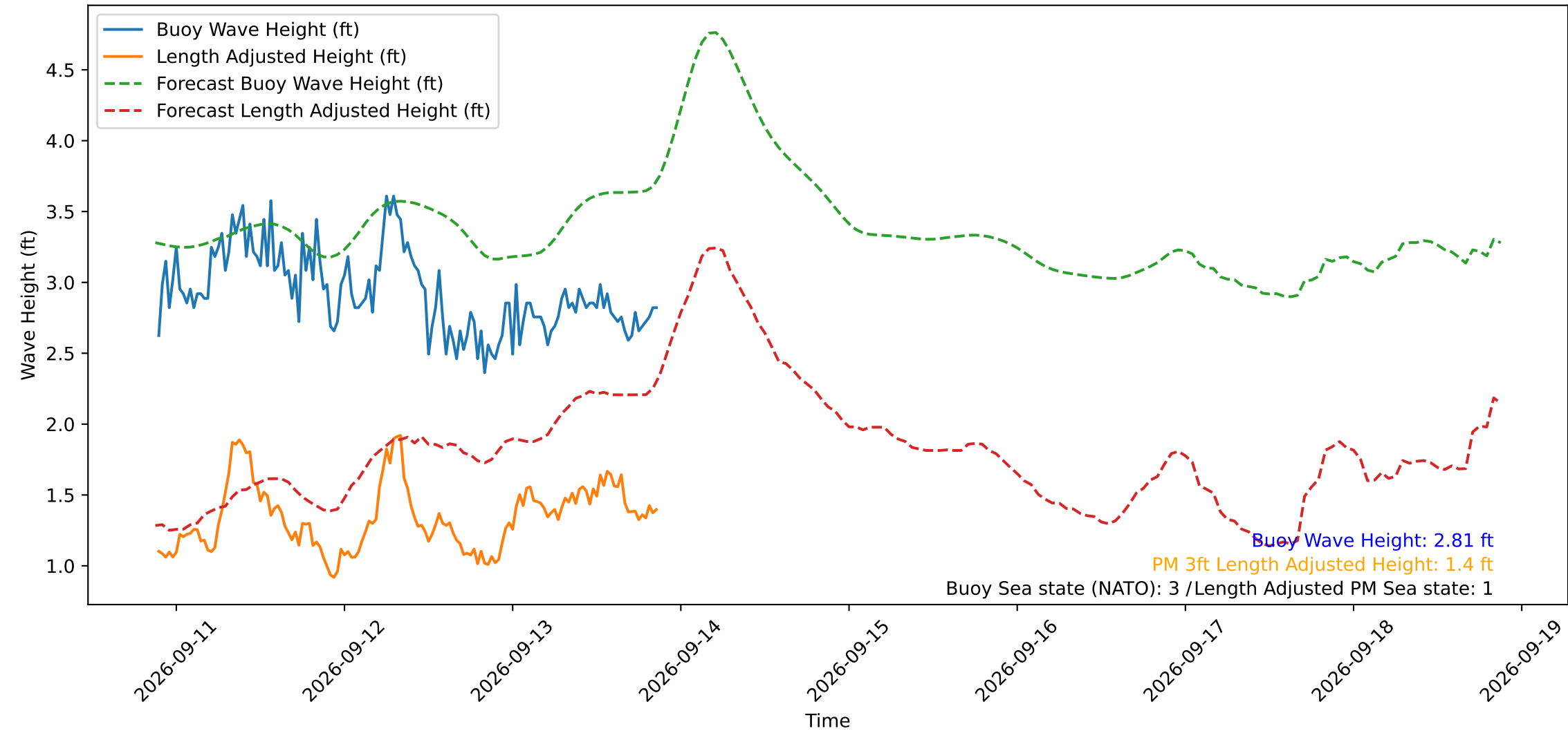
Wave Heights over Time for Green Beach at 2026-09-13 21:11:12
