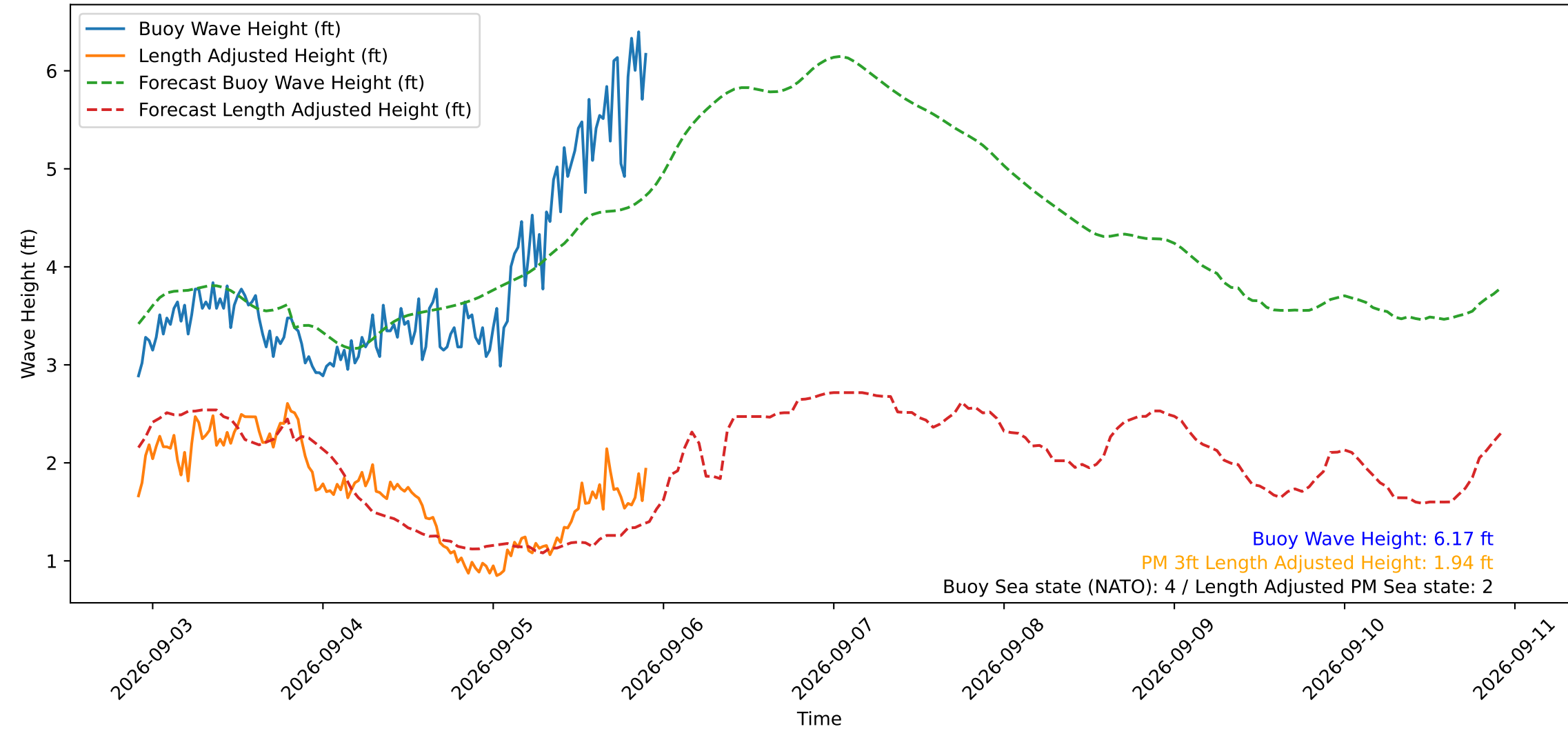
Wave Heights over Time for Oceanside Harbor at 2026-09-05 22:00:30
