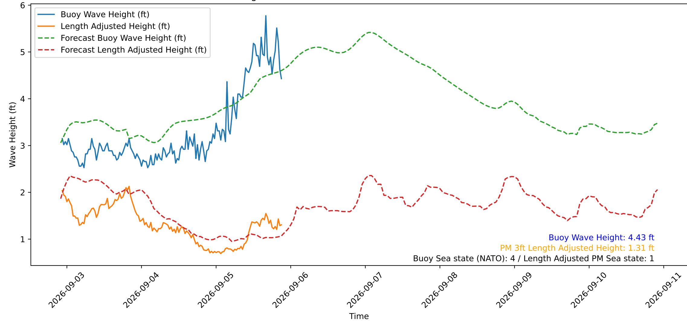
Wave Heights over Time for Red Beach at 2026-09-05 22:00:49
