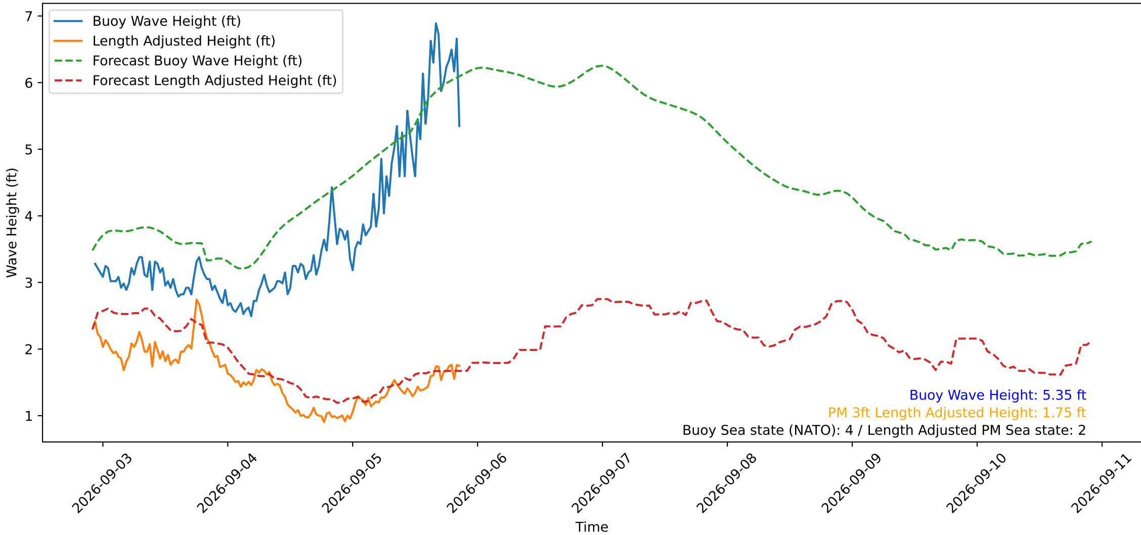
Wave Heights over Time for Green Beach at 2026-09-05 22:01:12
