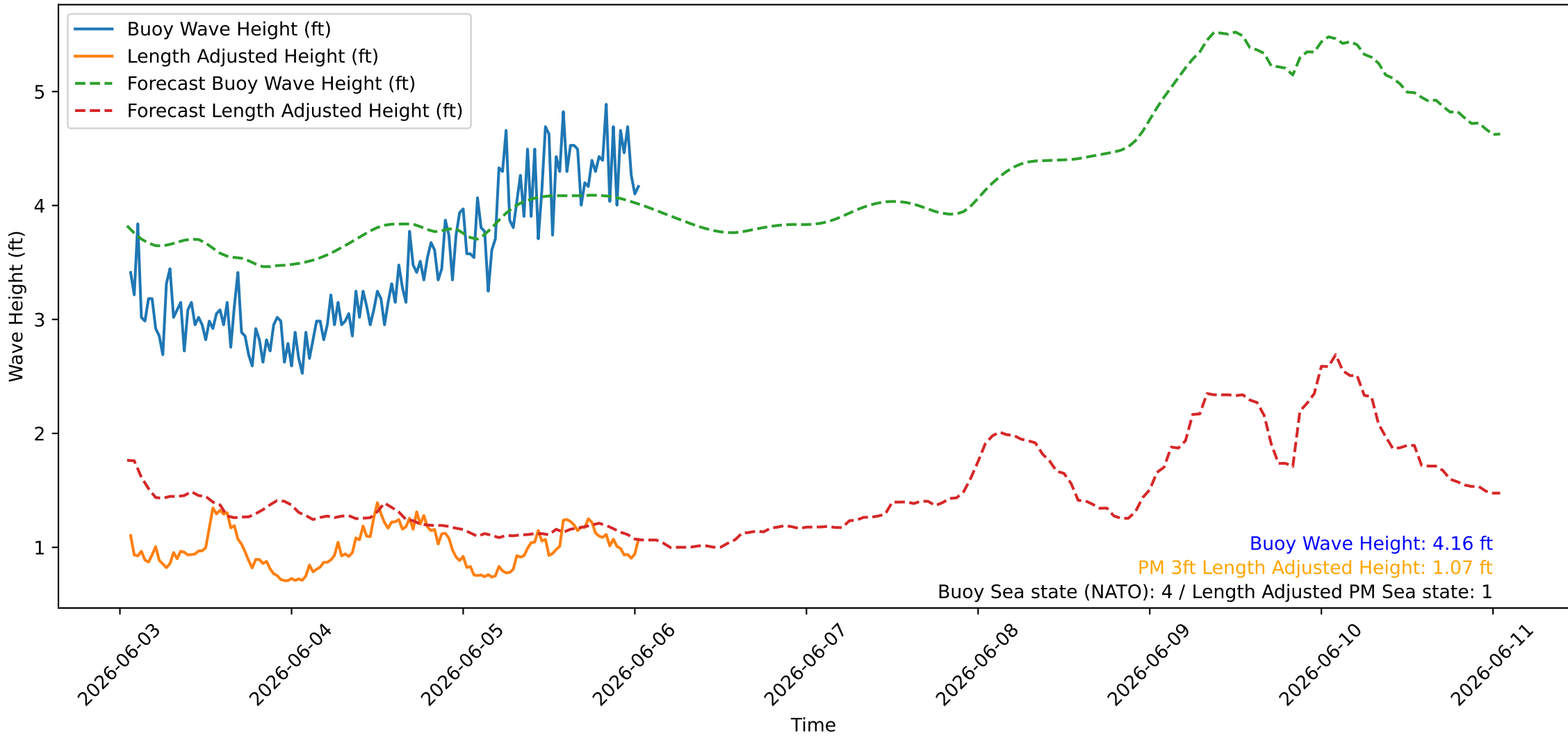
Wave Heights over Time for Red Beach at 2026-06-06 01:10:45
