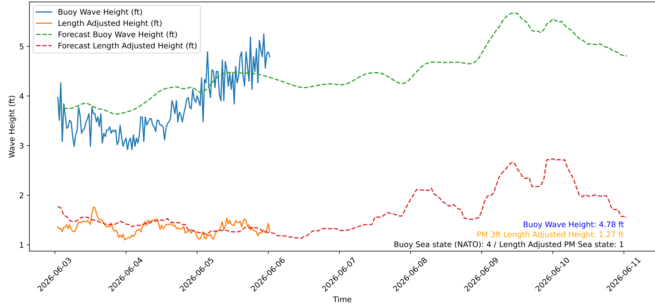
Wave Heights over Time for Oceanside Harbor at 2026-06-06 01:10:26
