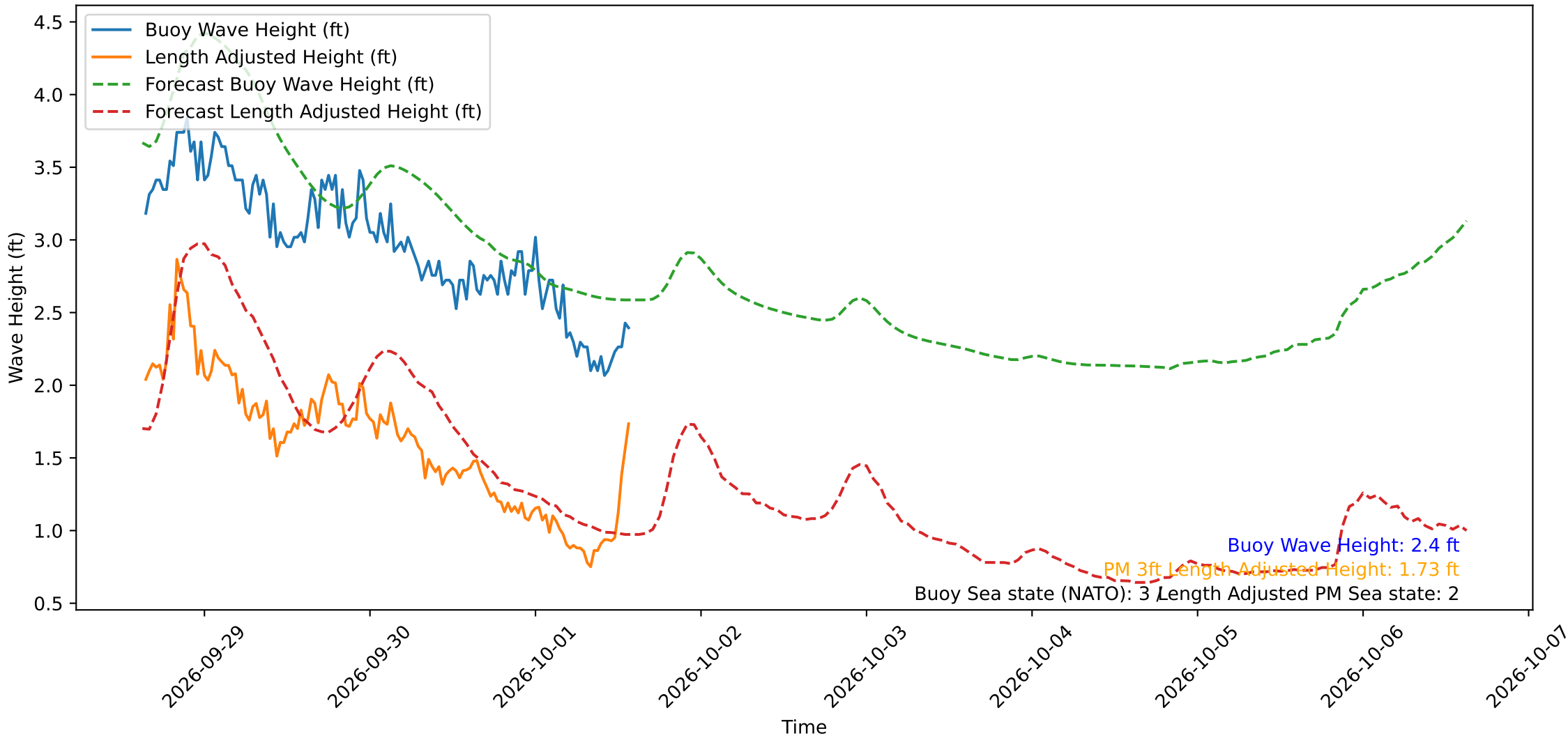
Wave Heights over Time for Red Beach at 2026-10-01 15:00:49
