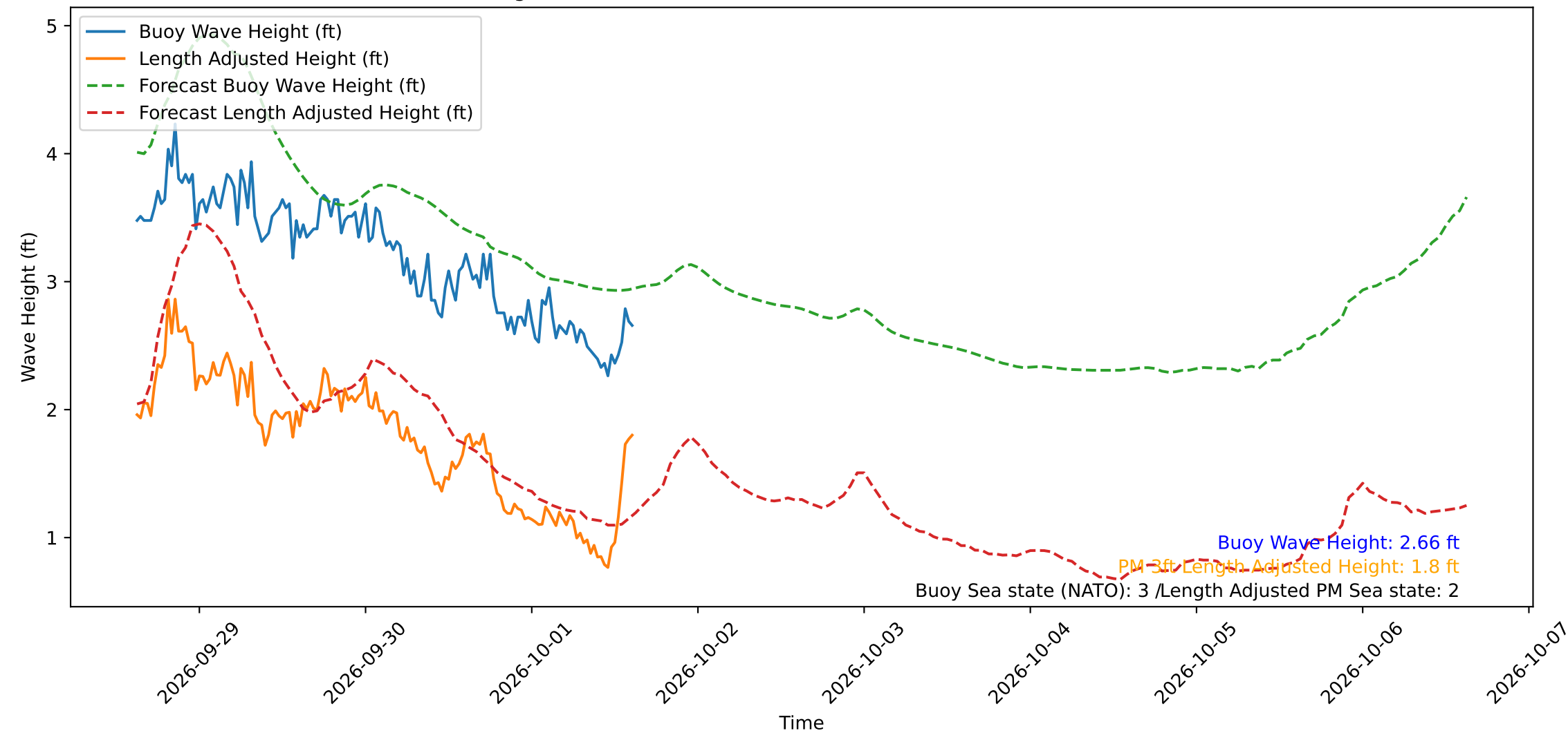
Wave Heights over Time for Oceanside Harbor at 2026-10-01 15:00:29
