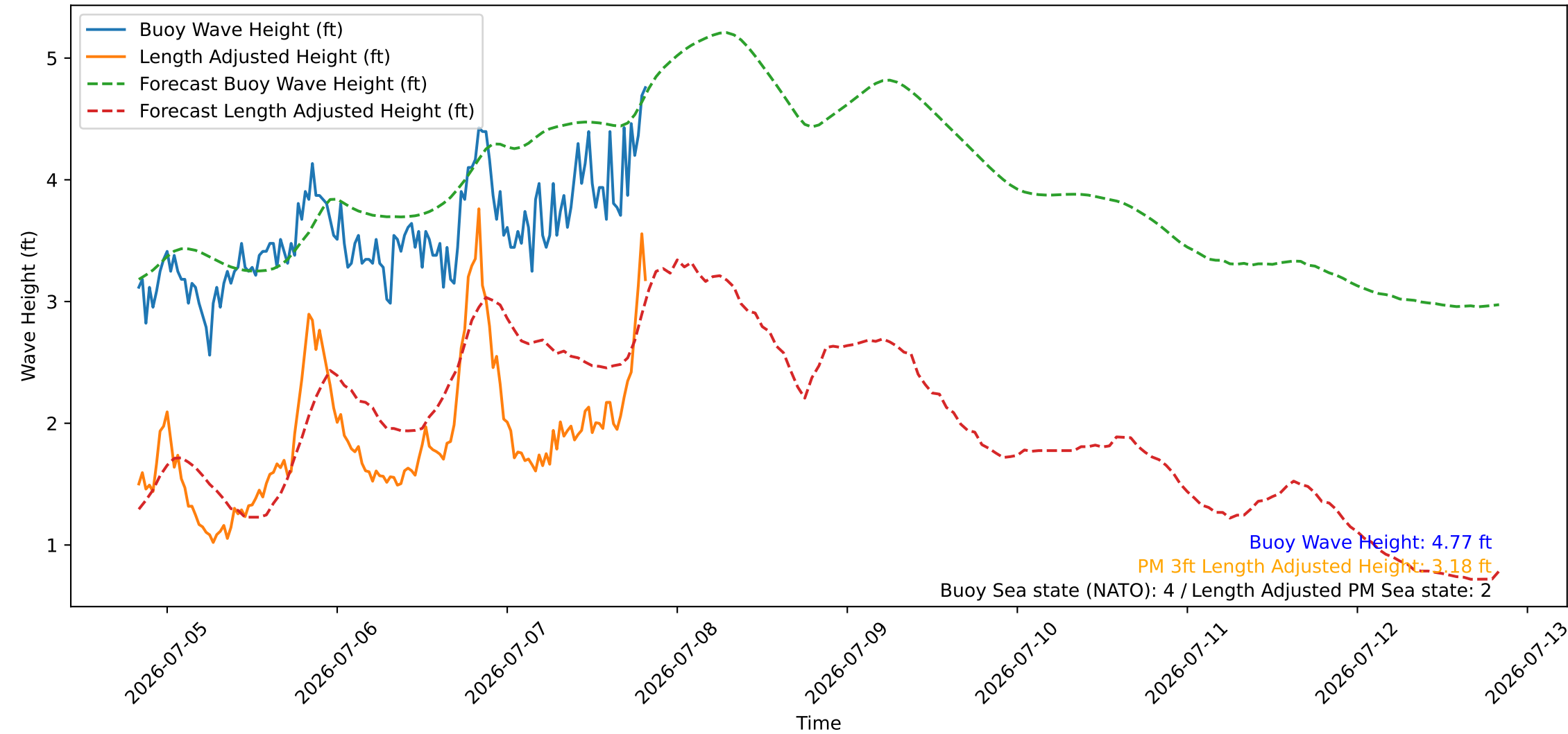
Wave Heights over Time for Green Beach at 2026-07-07 20:11:08
