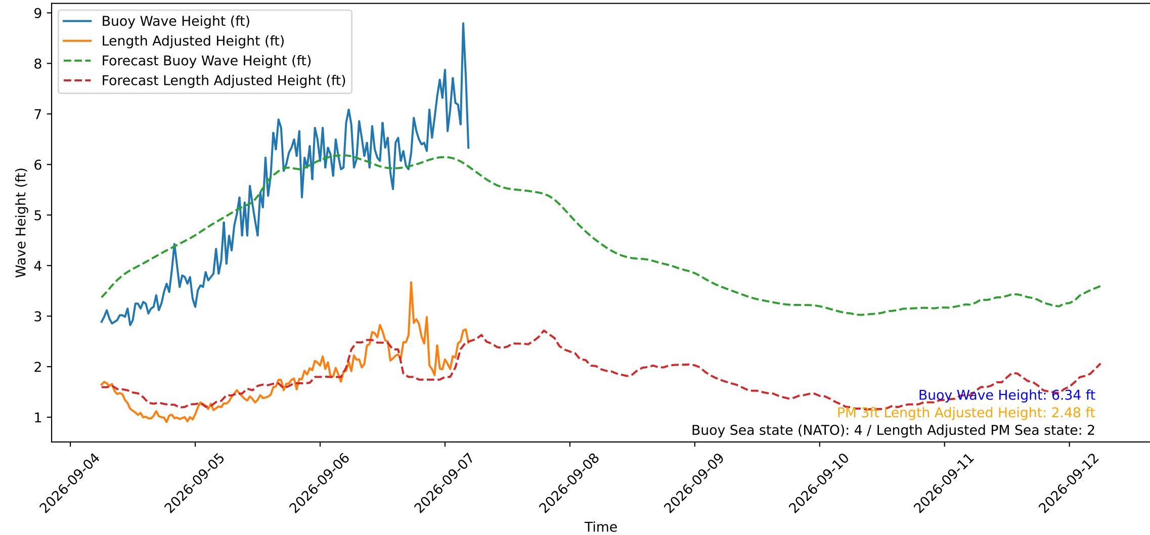
Wave Heights over Time for Green Beach at 2026-09-07 05:31:13
