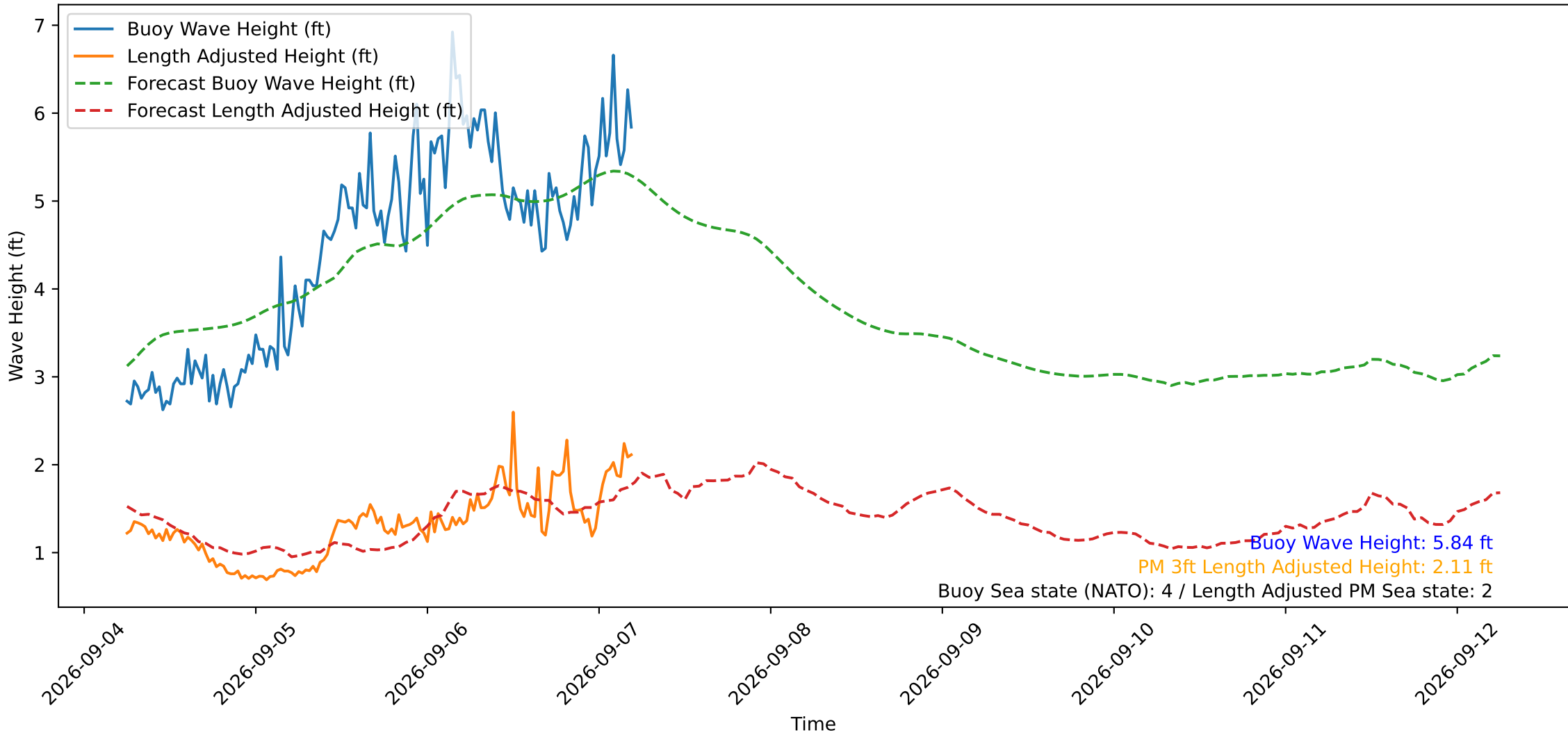
Wave Heights over Time for Red Beach at 2026-09-07 05:30:50
