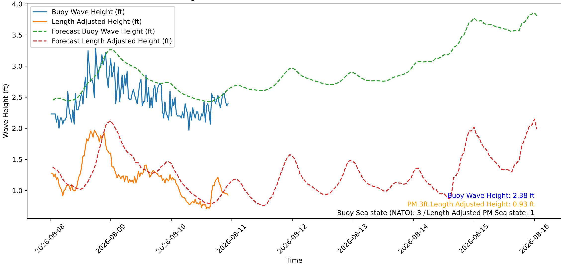
Wave Heights over Time for Oceanside Harbor at 2026-08-11 00:40:26
