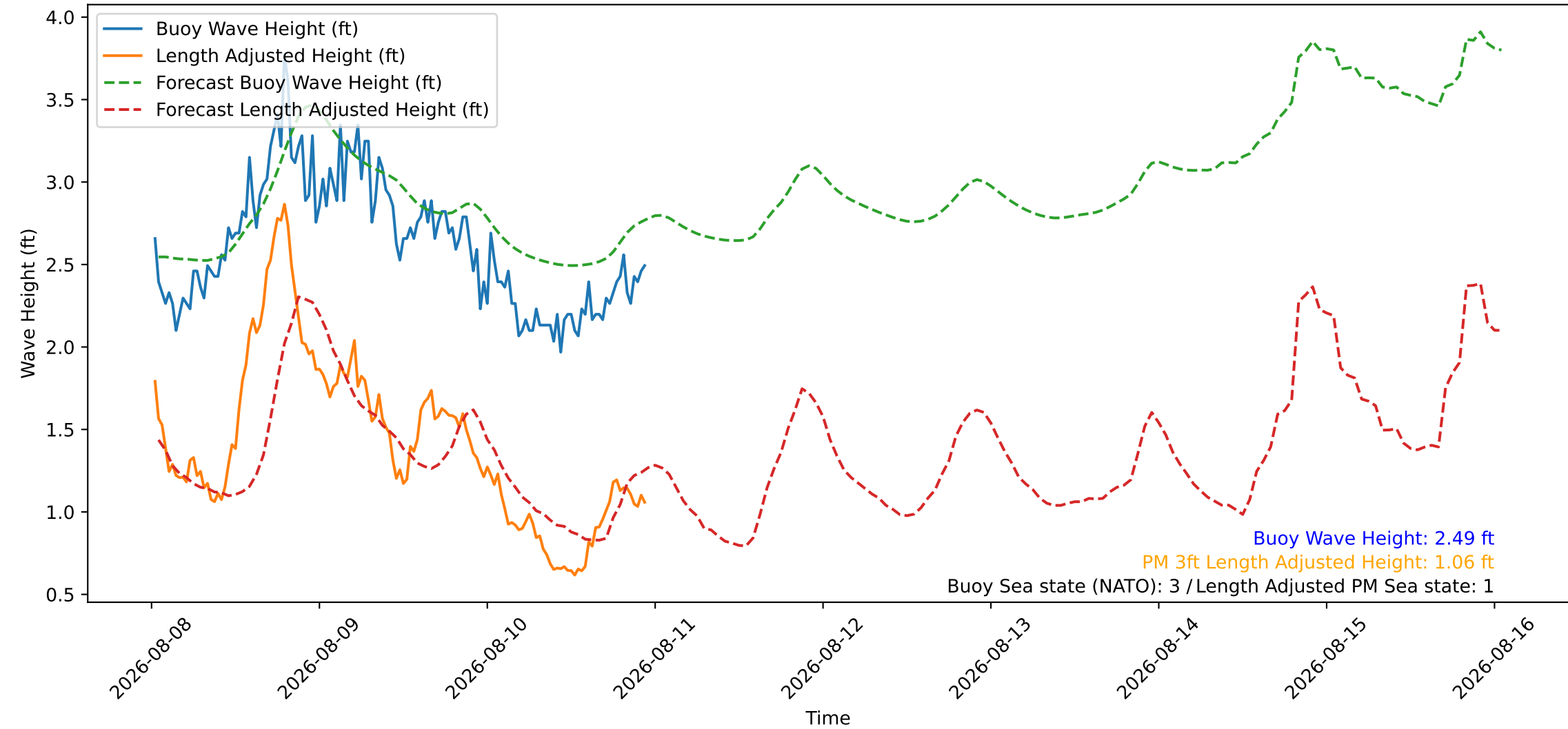
Wave Heights over Time for Green Beach at 2026-08-11 00:41:08
