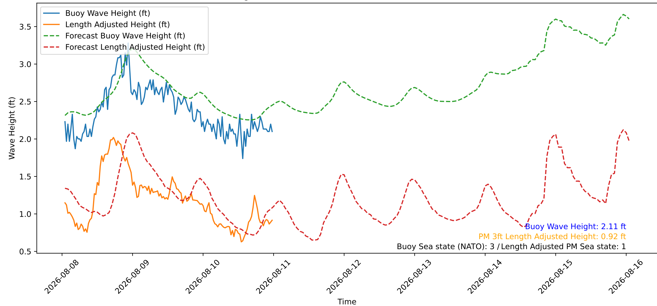
Wave Heights over Time for Red Beach at 2026-08-11 00:40:45
