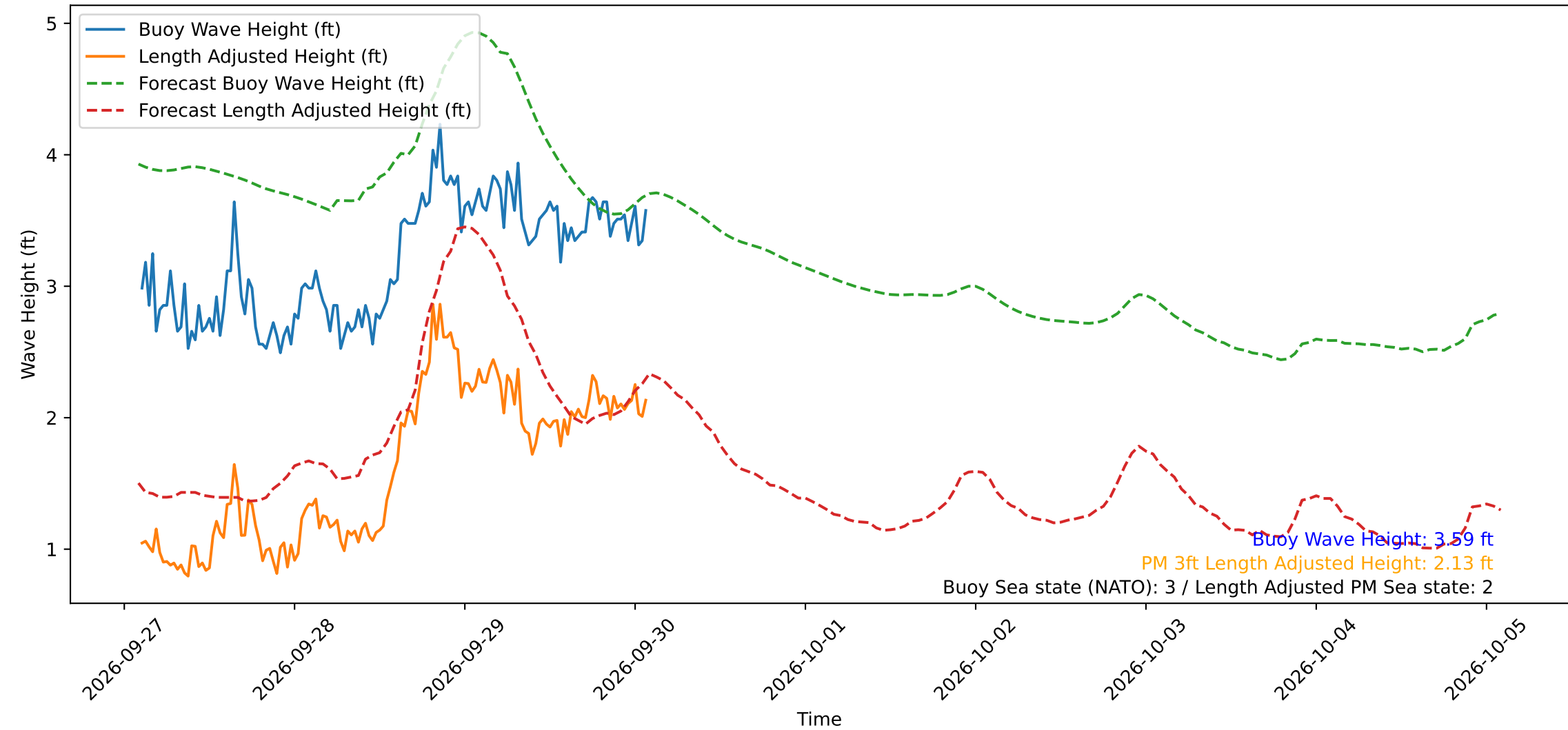
Wave Heights over Time for Oceanside Harbor at 2026-09-30 02:20:30
