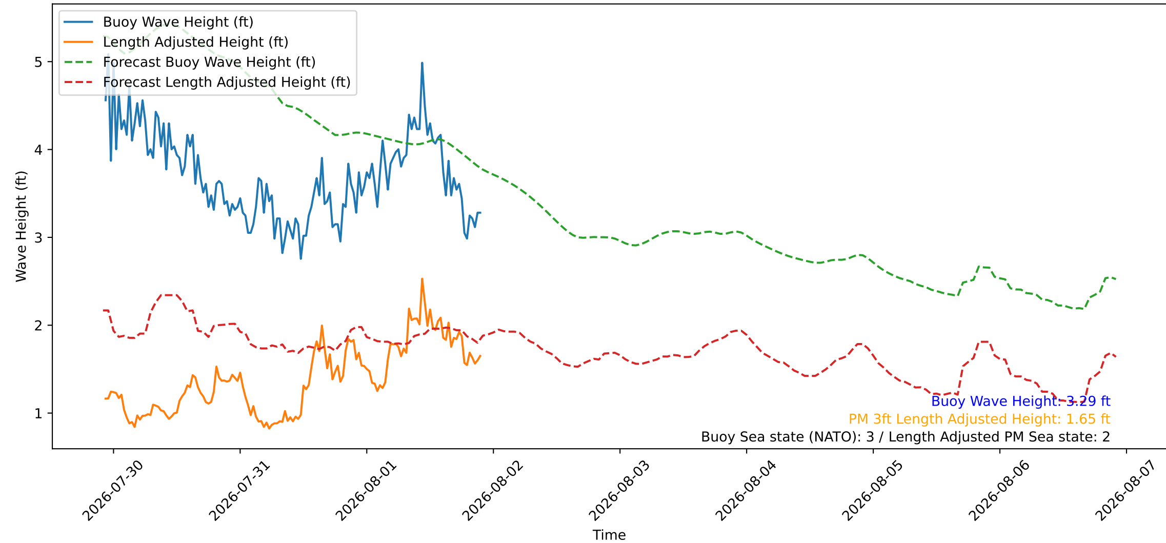
Wave Heights over Time for Green Beach at 2026-08-01 22:21:08
