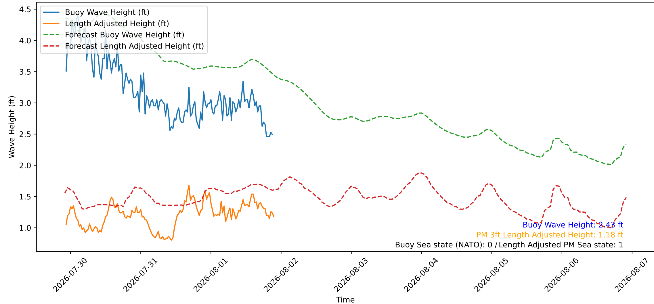
Wave Heights over Time for Red Beach at 2026-08-01 22:20:46
