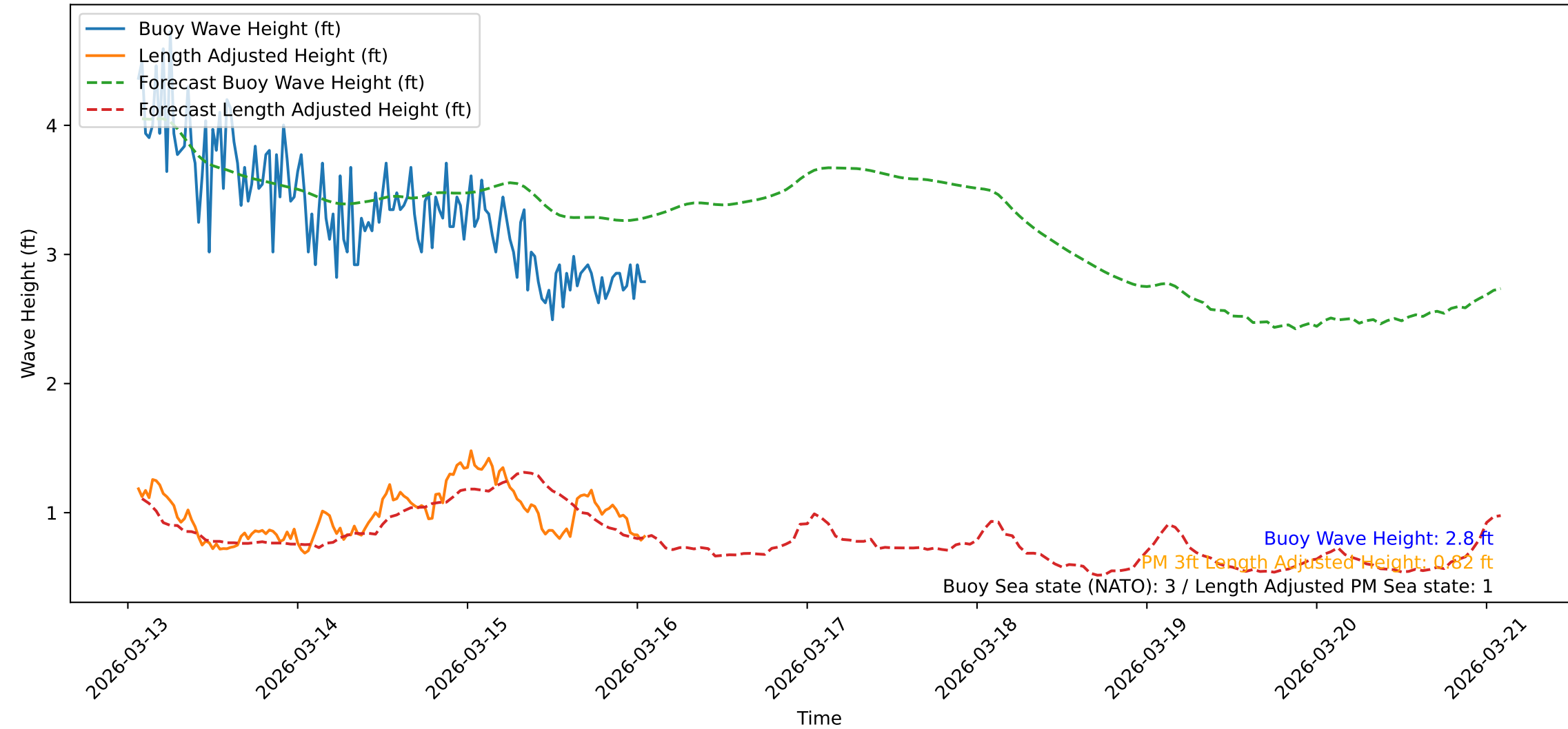
Wave Heights over Time for Oceanside Harbor at 2026-03-16 01:40:42
