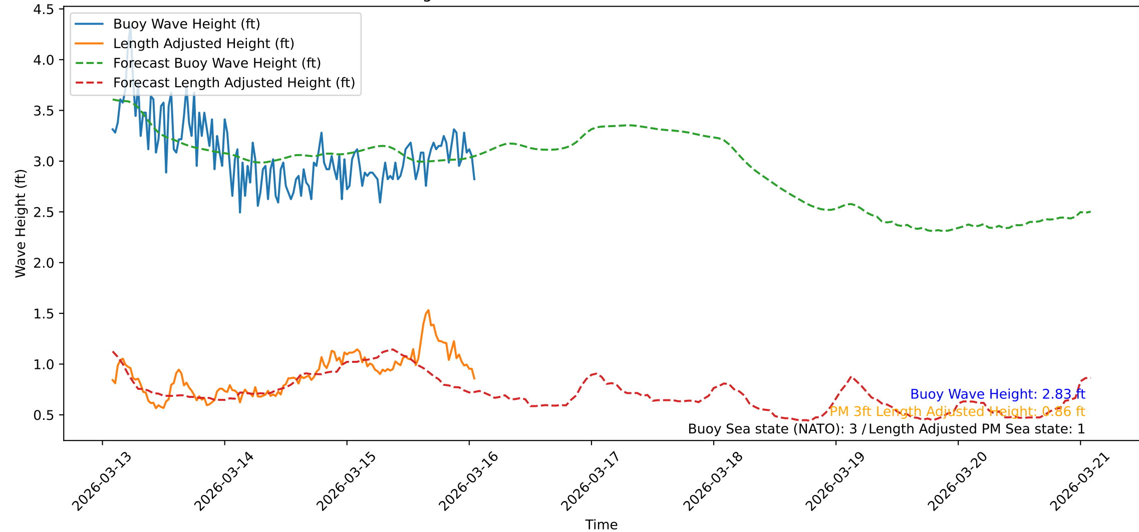
Wave Heights over Time for Red Beach at 2026-03-16 01:41:10
