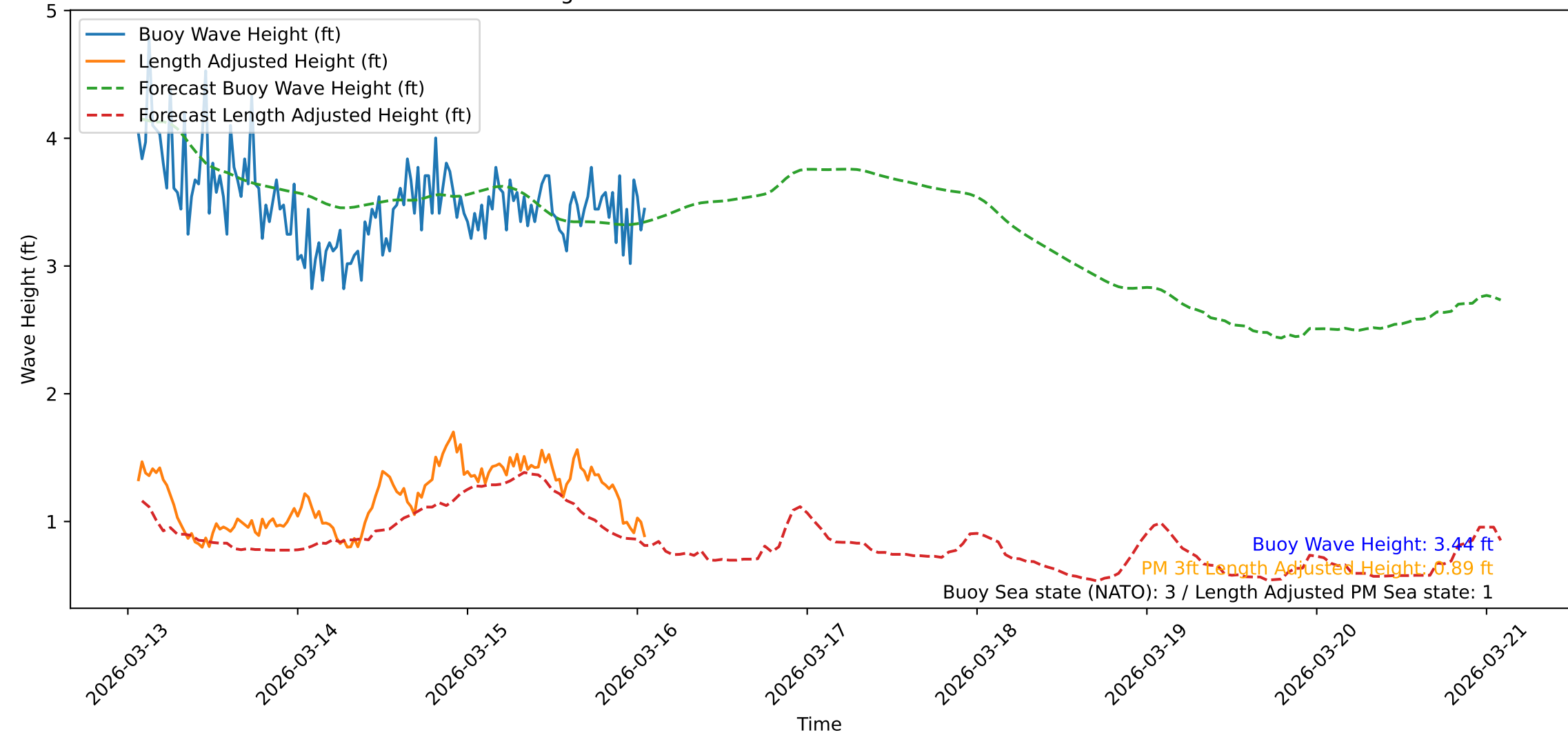
Wave Heights over Time for Green Beach at 2026-03-16 01:41:43
