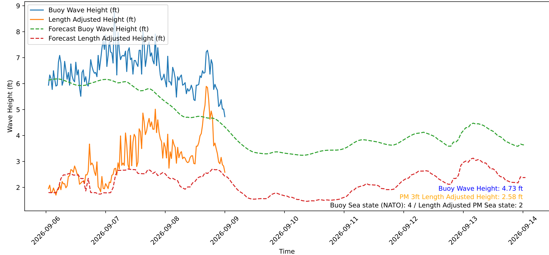
Wave Heights over Time for Green Beach at 2026-09-09 00:51:13
