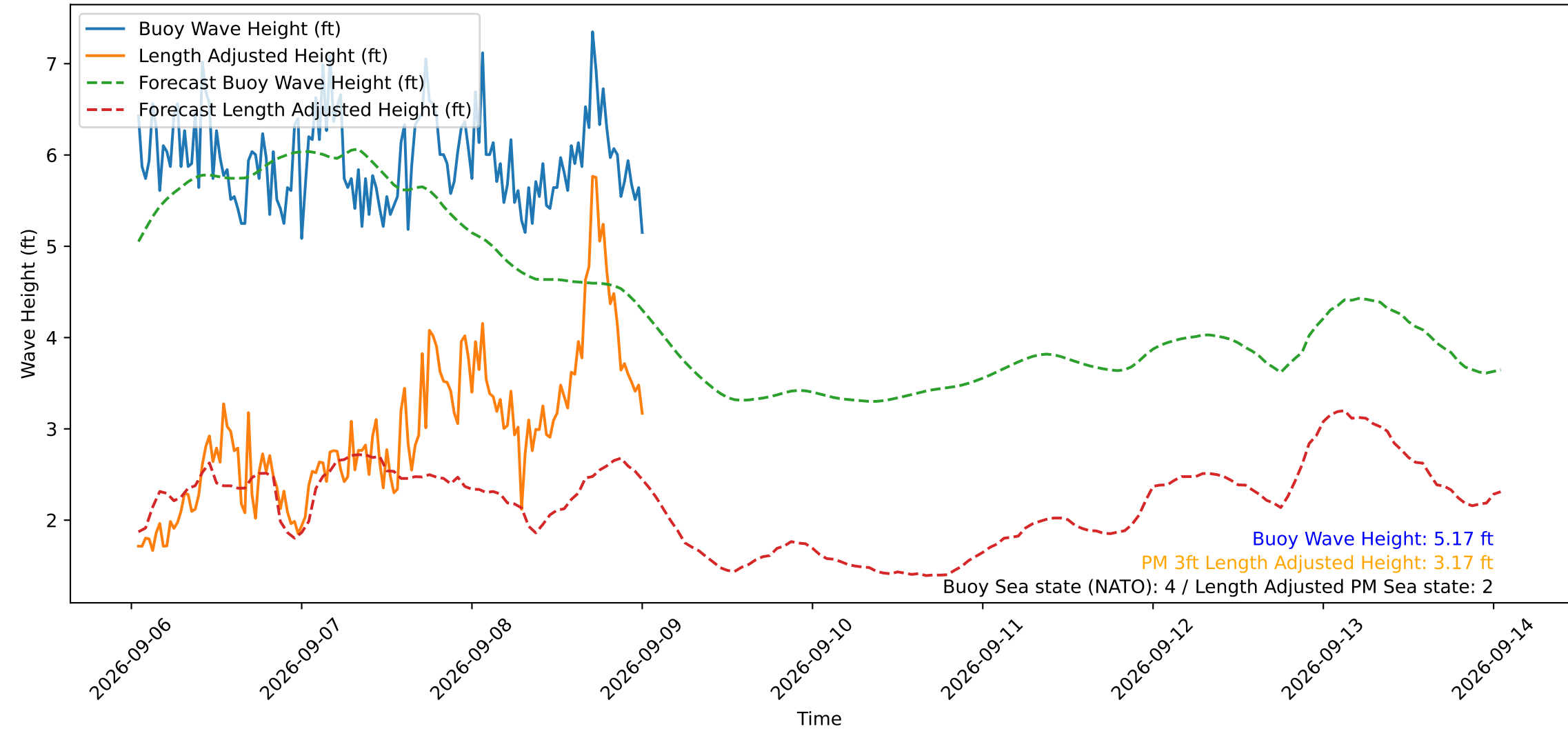
Wave Heights over Time for Oceanside Harbor at 2026-09-09 00:50:29
