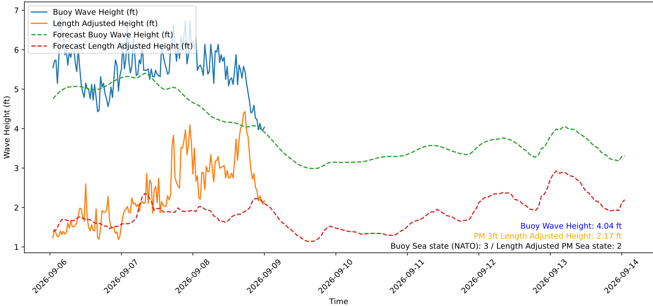
Wave Heights over Time for Red Beach at 2026-09-09 00:50:49
